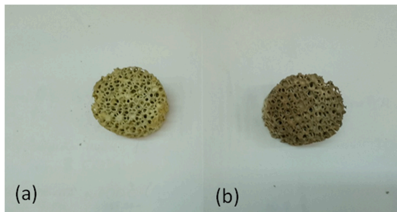
Figure 2. Structured OCF washcoated catalyst: (a) Ce 2 Ni and (b) Ce/Zr 2 Ni.
