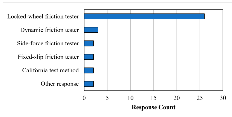
Figure 4. Pavement friction testing methods followed by state DOTs.
