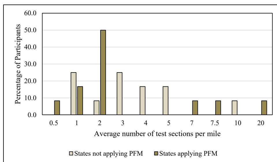
Figure 10. Average number of friction tests per mile for state DOTs.
