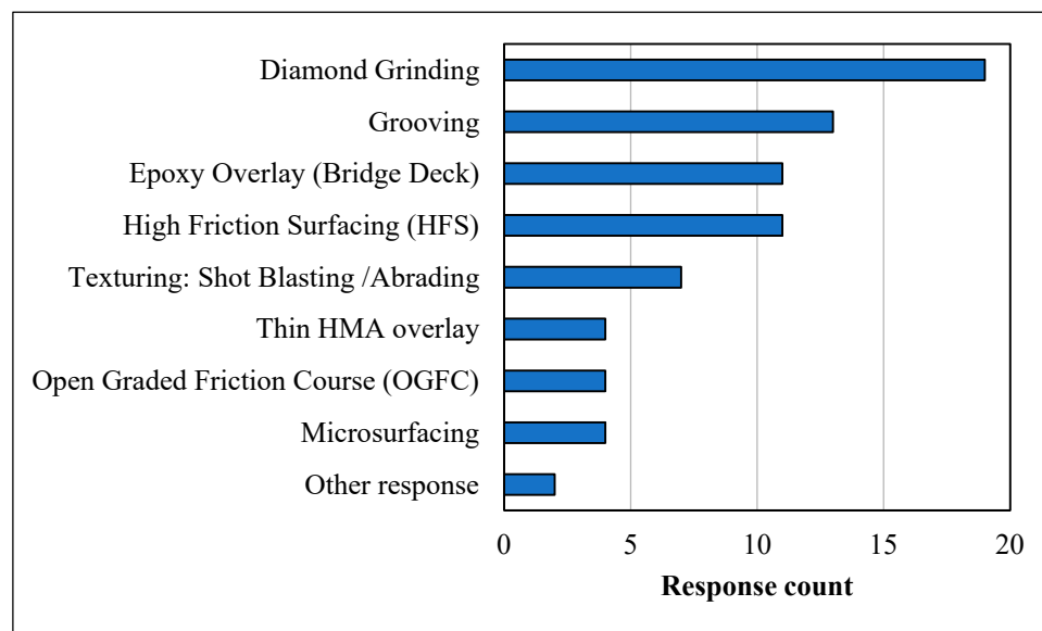
Figure 8. Types of pavement friction treatments considered for concrete pavement.
