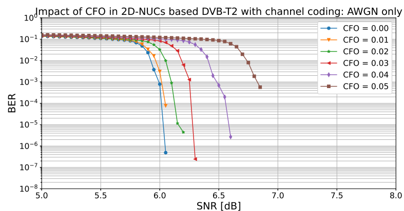
Figure 18. BER vs. SNR in the NUC-based DVB-T2 system with coding: CFO evaluation in the AWGN-only case.
