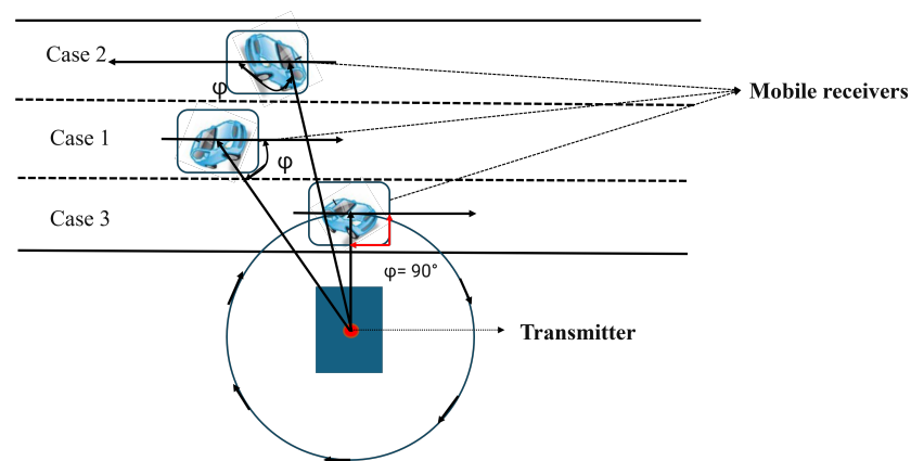
Figure 8. Doppler effect.
