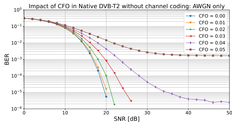
Figure 12. BER vs. SNR in the native DVB-T2 system without coding: CFO impact evaluation in the AWGN case.
