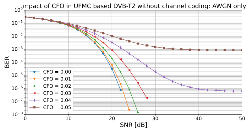
Figure 14. BER vs. SNR in the UPMC-based DVB-T2 system without coding: CFO evaluation in the AWGN-only case.
