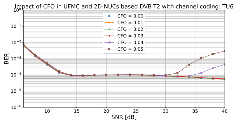
Figure 23. BER vs. SNR in the UPMC/NUC-based DVB-T2 system with coding: CFO evaluation in the TU6 and AWGN case. The comparison of curves in terms of signal-to-noise ratio (SNR) values obtained at different BER values ( 10^{-3} , 10^{-4} , 10^{-5} ) is shown in the following table.
