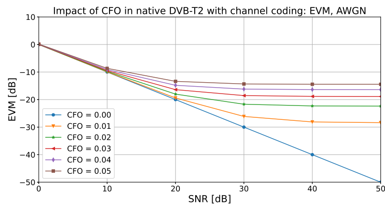
Figure 26. EVM vs. SNR in the native DVB-T2 system with coding: CFO evaluation in AWGN case only.
