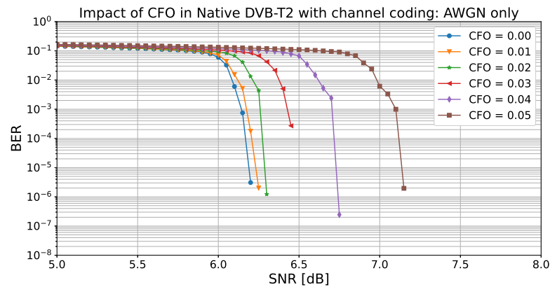
Figure 16. BER vs. SNR in the native DVB-T2 system with coding: CFO evaluation in the AWGN-only case.
