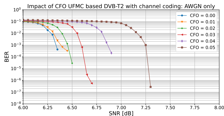
Figure 20. BER vs. SNR in the UPMC-based DVB-T2 system with coding: CFO evaluation in the AWGN-only case.
