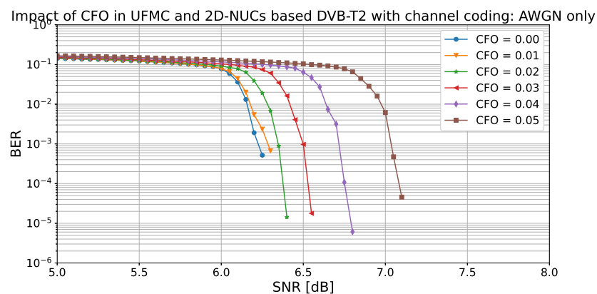
Figure 22. BER vs. SNR in the UPMC/NUC-based DVB-T2 system with coding: CFO evaluation in the AWGN-only case. The comparison of curves in terms of signal-to-noise ratio (SNR) values obtained at different BER values ( 10^{-3} , 10^{-4} , 10^{-5} ) is shown in the following table.
