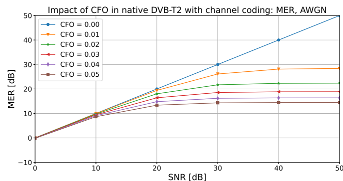
Figure 24. MER vs. SNR in the native DVB-T2 system with coding: CFO evaluation in the AWGN-only case.
