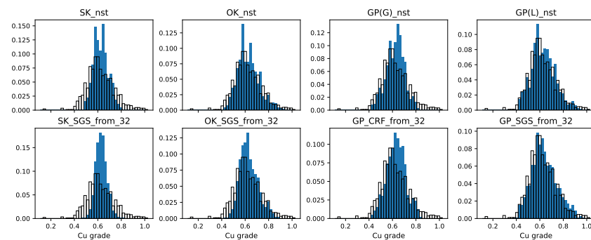
Figure 11. Copper grade histograms for g_D = 2310 and m_A = 4 . Black hollow: ground truth. Blue: model predictions.
