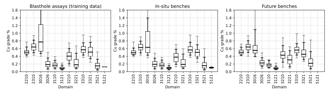
Figure 5. Copper grade distribution across different domains for inference period m_A = 6 . In each box-plot, the outer (faint) and inner (dark) whiskers represent the 2.15/97.85 and 8.87/91.13 percentiles, whereas the horizontal bar and box edges represent the median and lower/upper quartiles, respectively. From an economic perspective, porphyry orebodies can be mined profitably from Cu concentrations as low as 0.15–0.3%. The left, middle and right plots pertain to blasthole training data, blocks that require in situ regression and future-bench prediction, respectively. As expected, in situ distributions more closely resemble the training data than future-bench distributions.
