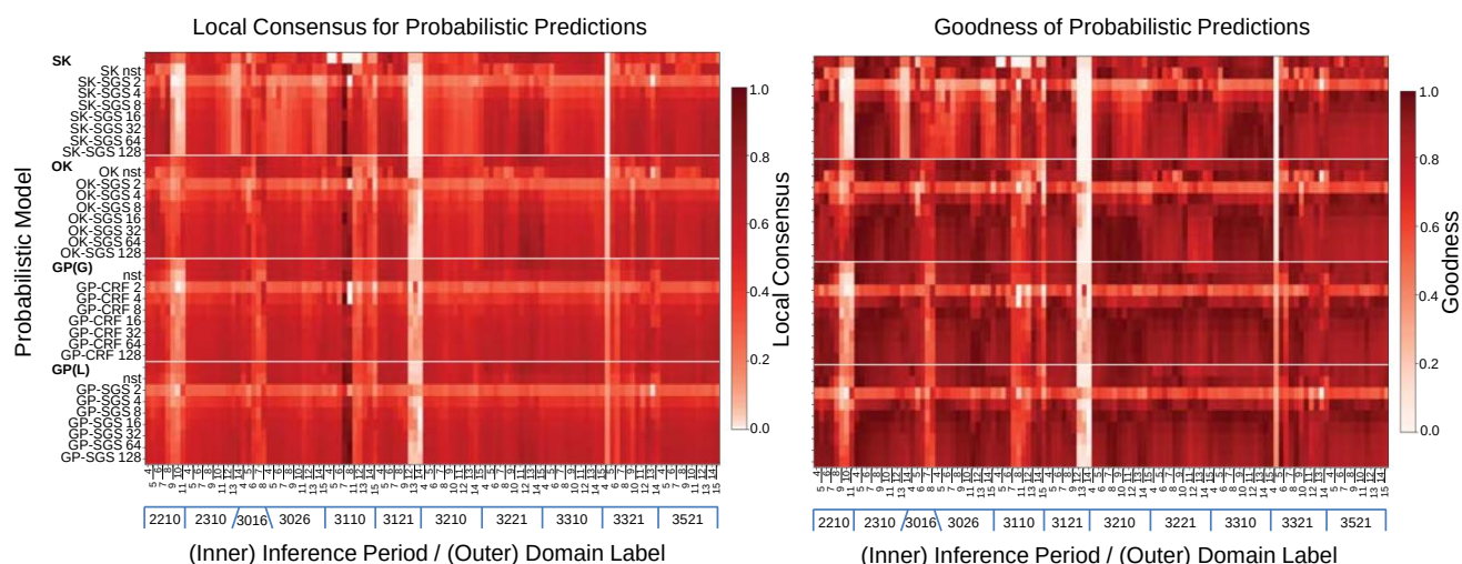
Figure 21. View of (left) consensus L and (right) goodness G for future-bench prediction across domains and inference periods.
