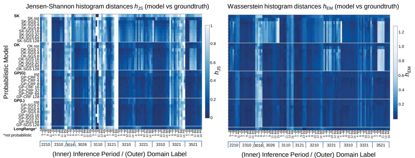
Figure 18. View of (left) Jensen–Shannon and (right) EM histogram distances for future-bench prediction across domains and inference periods.
