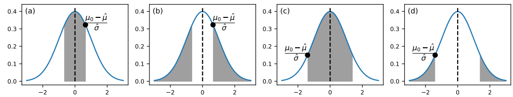
Figure 2. Illustration of coverage probability in (a,c) and consensus between model and observation in (b,d).
