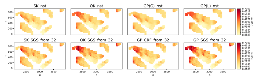
Figure 8. Mean copper grade predicted by models for domain g_D = 3521 and inference period m_A = 4 .
