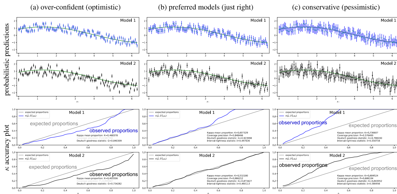
Figure 3. Evaluating the uncertainty and predictive performance of two synthesised models. Top: probabilistic predictions. Bottom: \kappa accuracy plots. From left to right, (a–c) show what can be expected from the optimistic, preferred and conservative models.
