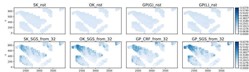
Figure 10. Copper grade standard deviation predicted by models for domain g_D = 3521 and inference period m_A = 4 .
