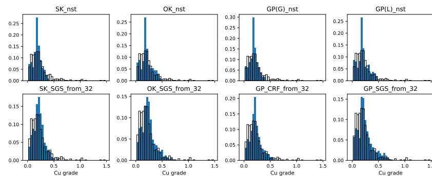
Figure 12. Copper grade histograms for g_D = 3521 and m_A = 4 . Black hollow: ground truth. Blue: model predictions.
