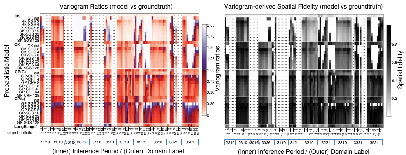
Figure 19. View of (left) variogram ratios R and (right) spatial fidelity F for future-bench prediction across domains and inference periods.
