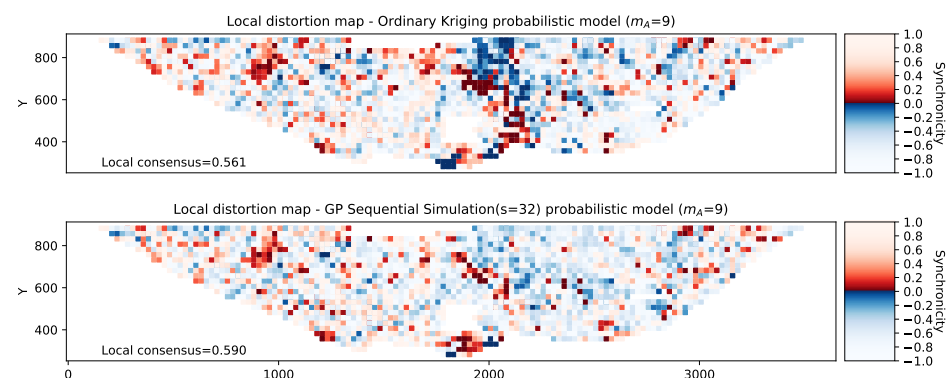
Figure 23. Synchronicity map comparing model predictions with the ground truth across multiple domains. Dark patches indicate a high degree of inconsistency between prediction and ground truth. Red and blue colours indicate underestimation and overestimation, respectively.
