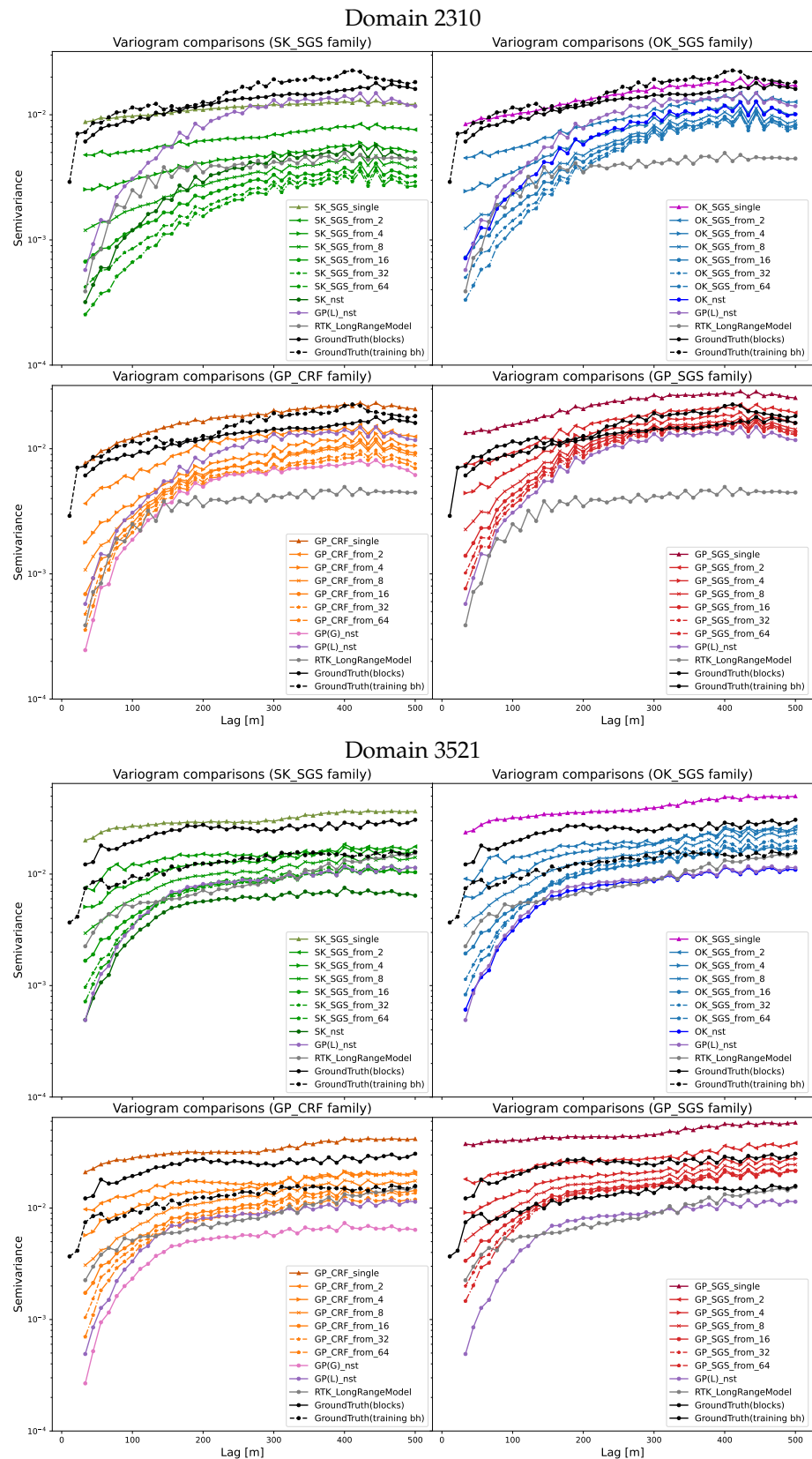
Figure 14. Copper grade variograms for g_D = 2310 and g_D = 3521 in m_A = 4 . The quadrants group together models in the following families: (northwest) SK/SK-SGS, (northeast) OK/OK-SGS, (southwest) GP(G)/GP-CRF, (southeast) GP(L)/GP-SGS.
