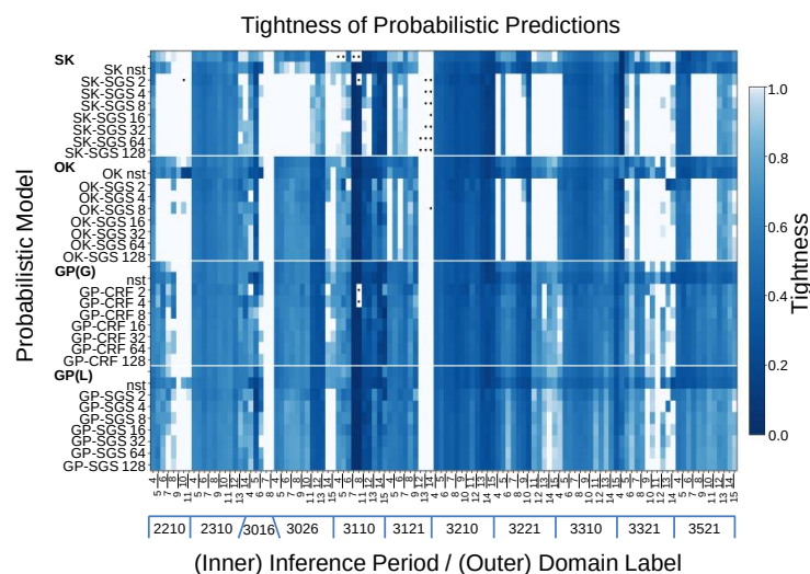
Figure 22. View of interval tightness I for future-bench prediction across domains and inference periods.
