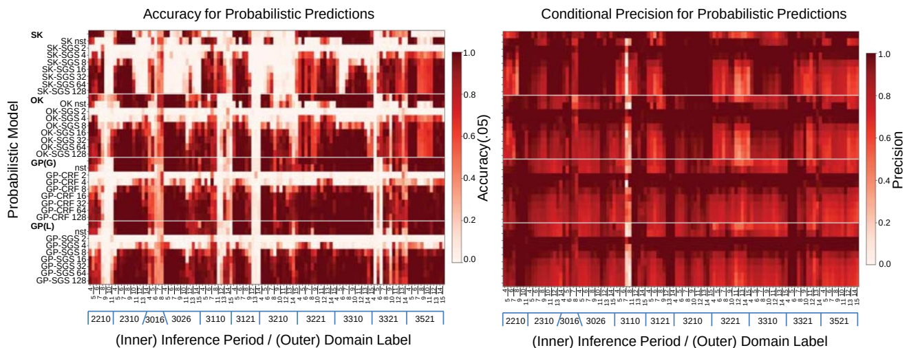
Figure 20. View of (left) accuracy A and (right) precision P for future-bench prediction across domains and inference periods.
