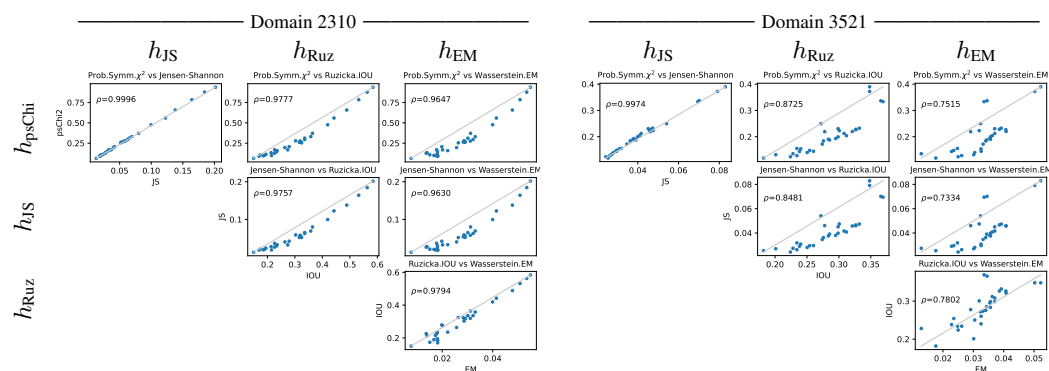
Figure 13. Histogram distances cross-plots for g_D = 2310 and g_D = 3521 in m_A = 4 .
