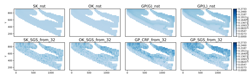
Figure 9. Copper grade standard deviation predicted by models for domain g_D = 2310 and inference period m_A = 4 .
