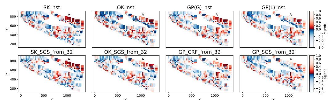
Figure 16. Synchronicity of grade predictions with regard to the ground truth for g_D = 2310 and m_A = 4 .
