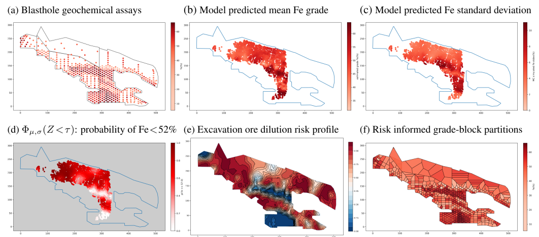
Figure 1. A motivating example. For open-pit mining at iron ore deposits, (a) sparse assay measurements are taken from blastholes to facilitate ore grade probabilistic modelling. (b,c) These show the estimated mean Fe concentration and standard deviation in a local region soon to be excavated. The value of having a probabilistic model is that it provides a reliable and objective description of ore/waste distribution in spite of sampling errors and epistemic uncertainty. This allows operators to assess risks, such as ore dilution in (d), if a volume of low-grade material is dug up at a [red] location and transported to a high-grade destination. (e) A high-fidelity probabilistic model makes informed decision-making possible. Its applications include high-precision large-scale tracking of material movement, as well as (f) grade-block partitioning and reconfiguration during mine planning and the ability to reroute material to different destinations on demand [19].
