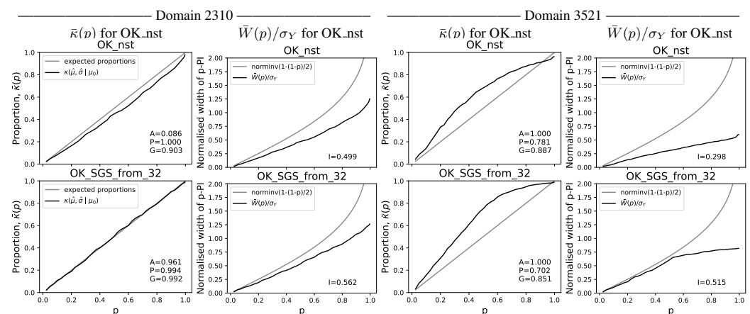
Figure 15. Copper grade predictive distribution accuracy and uncertainty interval plots. Selected results for g_D = 2310 and g_D = 3521 in m_A = 4 .
