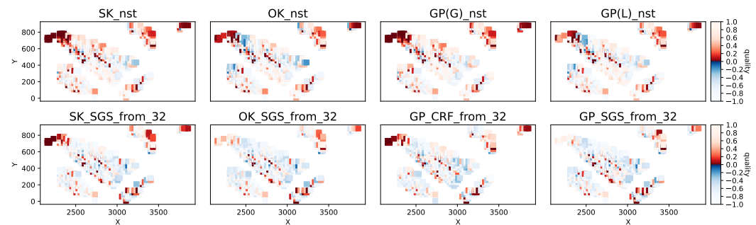
Figure 17. Synchronicity of grade predictions with regard to the ground truth for g_D = 3521 and m_A = 4 .
