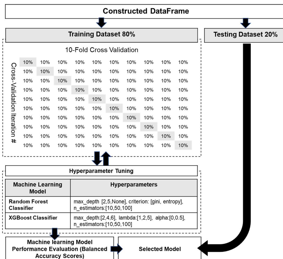
Figure 3. Machine learning model development summary.
