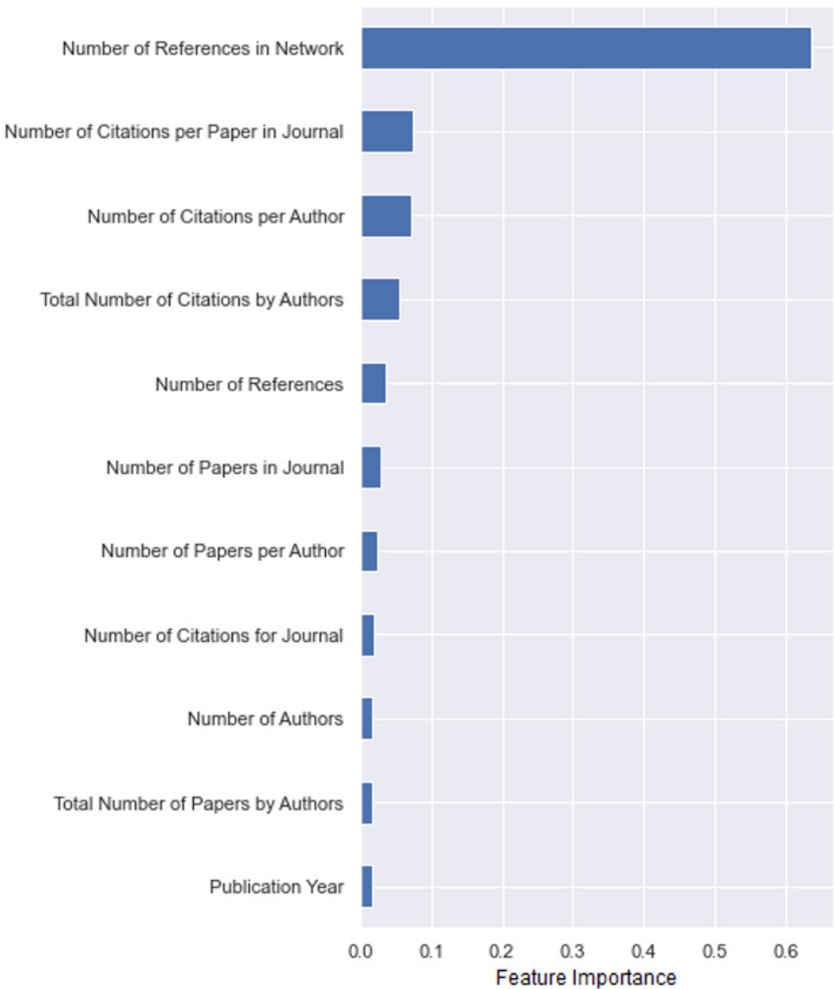
Figure 8. Feature importance.
