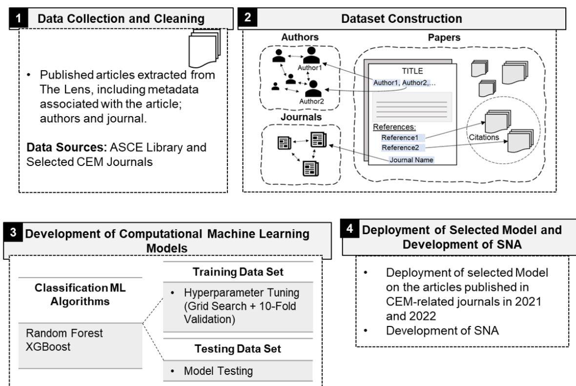
Figure 1. Research methodology.
