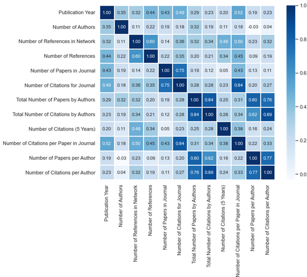
Figure 6. Correlation heatmap.
