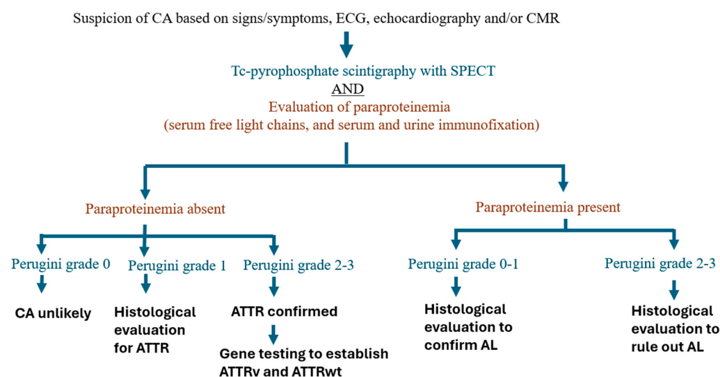
Figure 1. Multimodality imaging in cardiac amyloidosis. CA—cardiac amyloidosis; ATTRwt—wild-type transthyretin cardiac amyloidosis; ATTRv—variant transthyretin cardiac amyloidosis; AL—light-chain cardiac amyloidosis; CMR—cardiac magnetic resonance.
