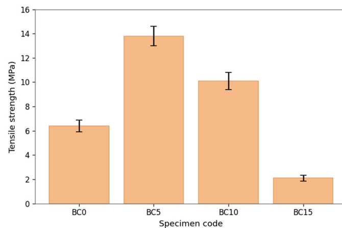
Figure 6. Tensile strength of biochar/coconut-fiber-reinforced vinyl ester composites.
