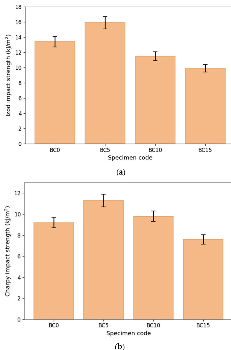
Figure 8. (a) Izod impact test; (b) Charpy impact test.
