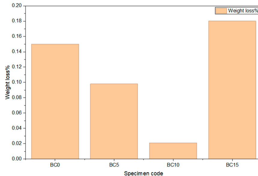
Figure 10. Weight loss percentage of biochar/coconut-leaf-sheath-fiber-reinforced vinyl ester composites.
