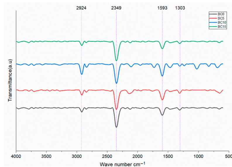
Figure 5. FTIR analysis of biochar/coconut-fiber-reinforced vinyl ester composites.
