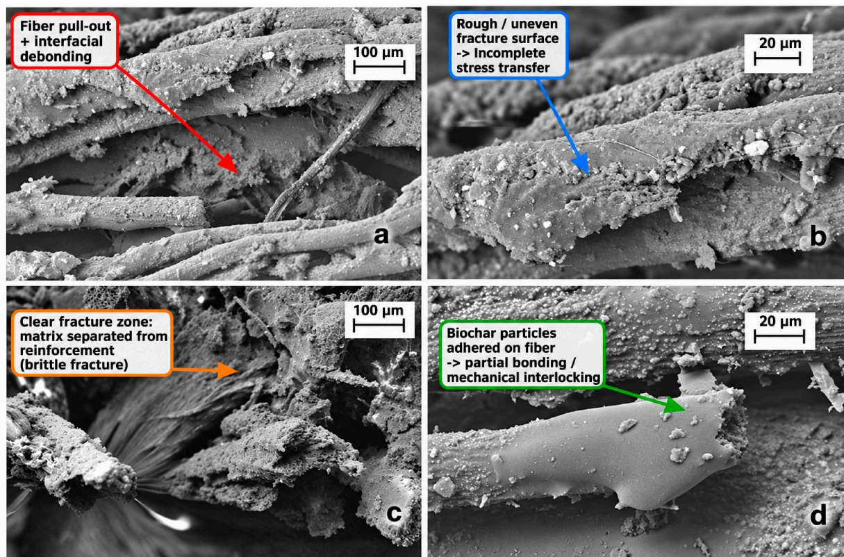
Figure 12. SEM micrographs of the fracture surfaces under flexural failure: (a,b) 5% biochar; (c,d) 10% biochar.
