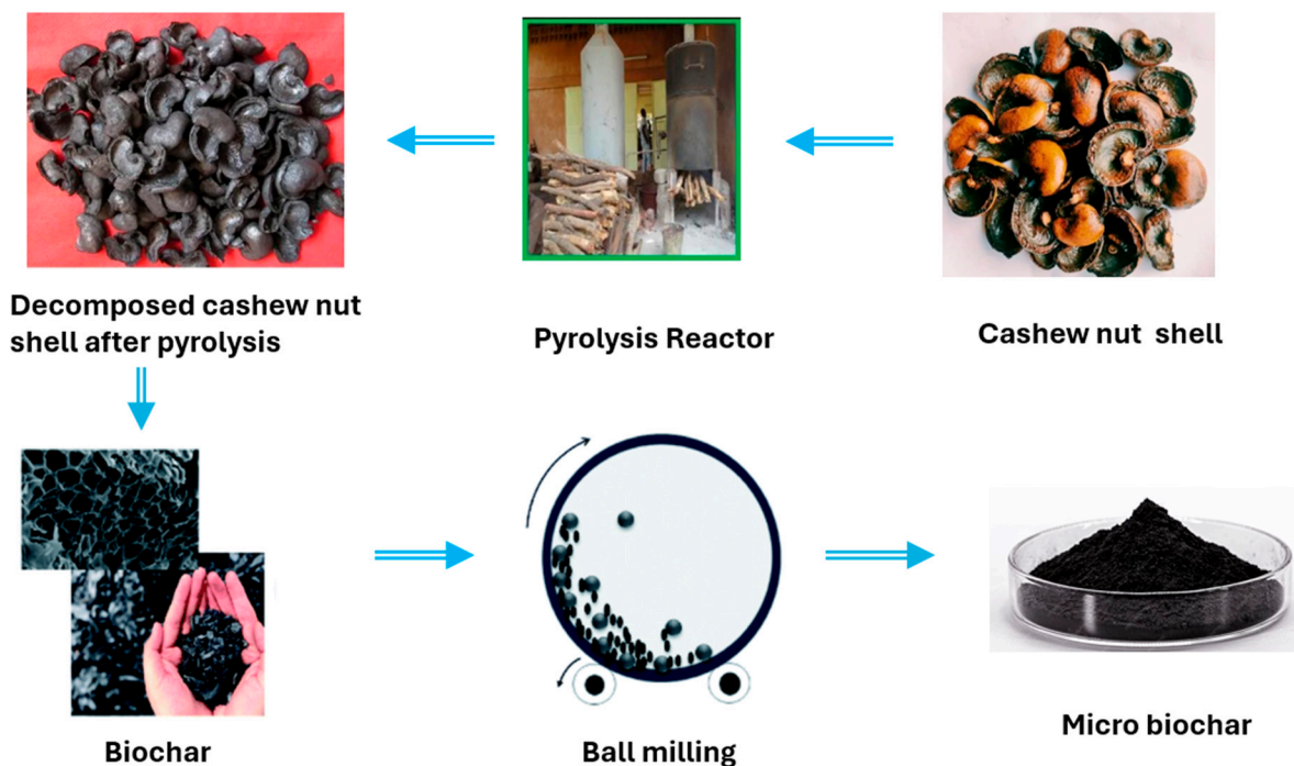
Figure 2. Schematic diagram of micro biochar production.
