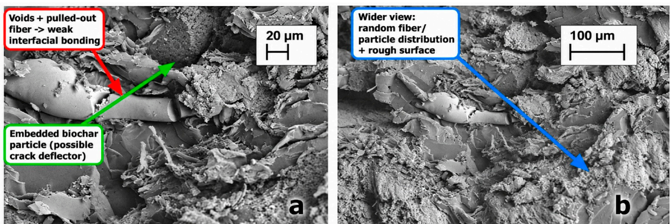
Figure 13. SEM micrographs of the fracture surfaces under impact failure of composite containing 10 wt.% biochar. (a) High Magnification; (b) Low Magnification.
