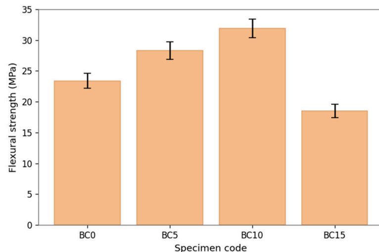
Figure 7. Flexural strength of biochar/coconut-fiber-reinforced vinyl ester composites.
