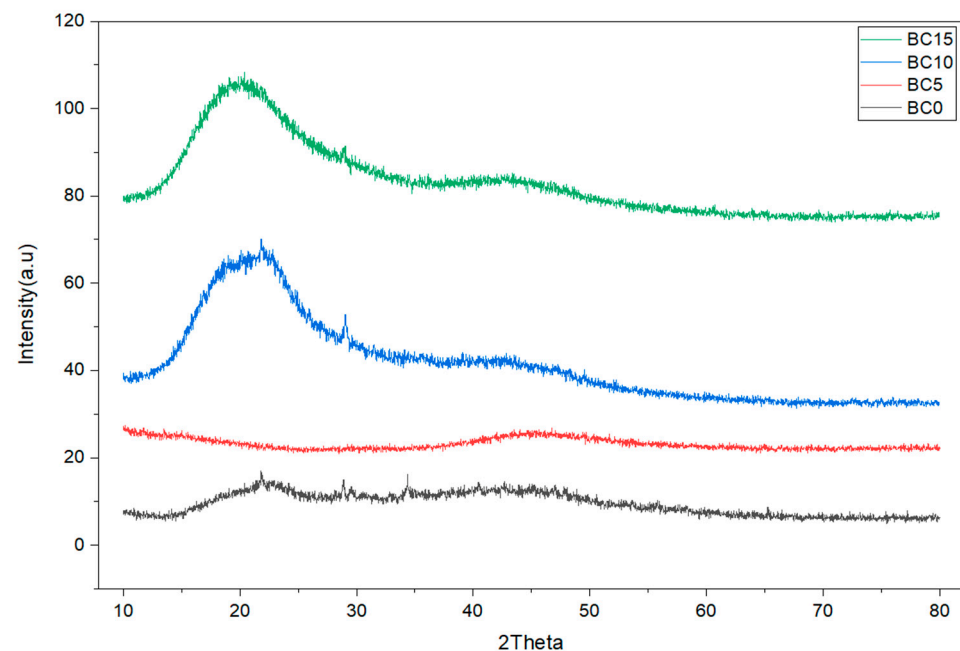
Figure 4. XRD analysis of biochar/coconut-fiber-reinforced vinyl ester composites.
