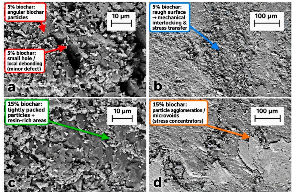
Figure 11. SEM micrographs of the fracture surfaces under tensile failure: (a,b) 5% biochar; (c,d) 15% biochar.
