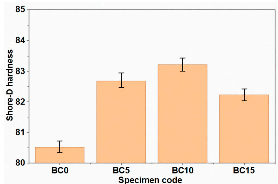
Figure 9. Shore-D hardness of biochar/coconut-fiber-reinforced vinyl ester composites.
