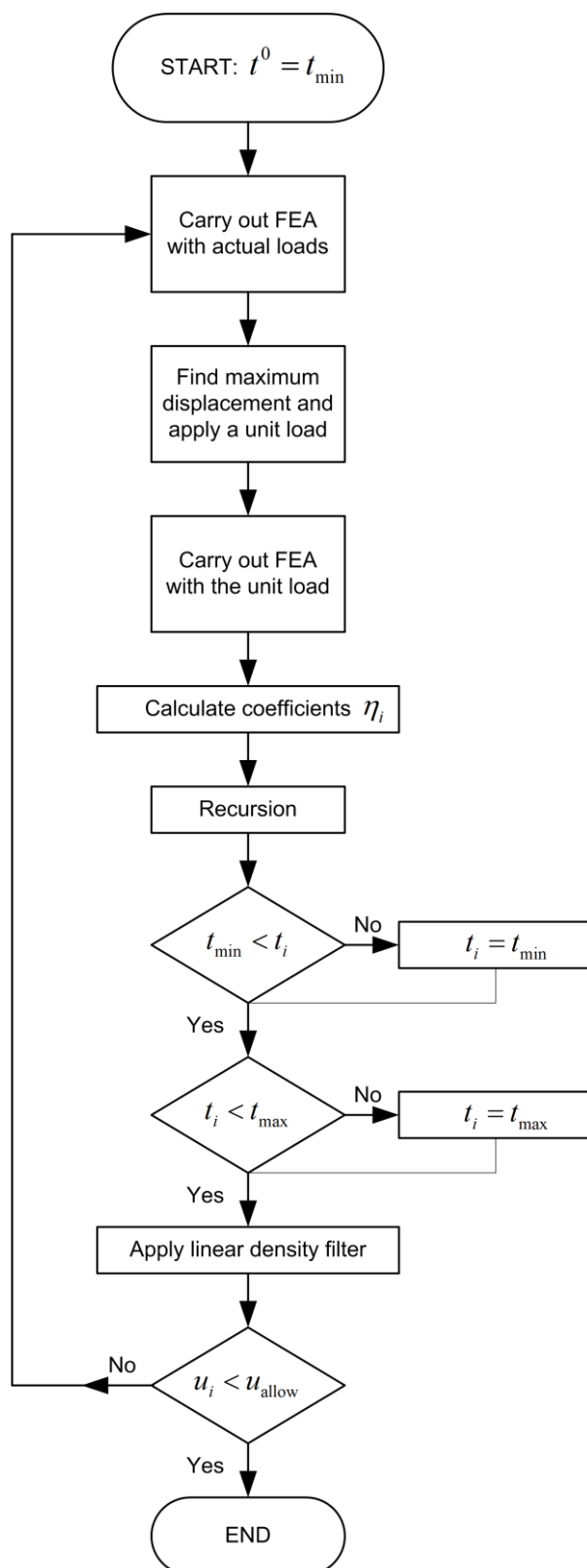
Figure 1. Flowchart of the proposed algorithm.
