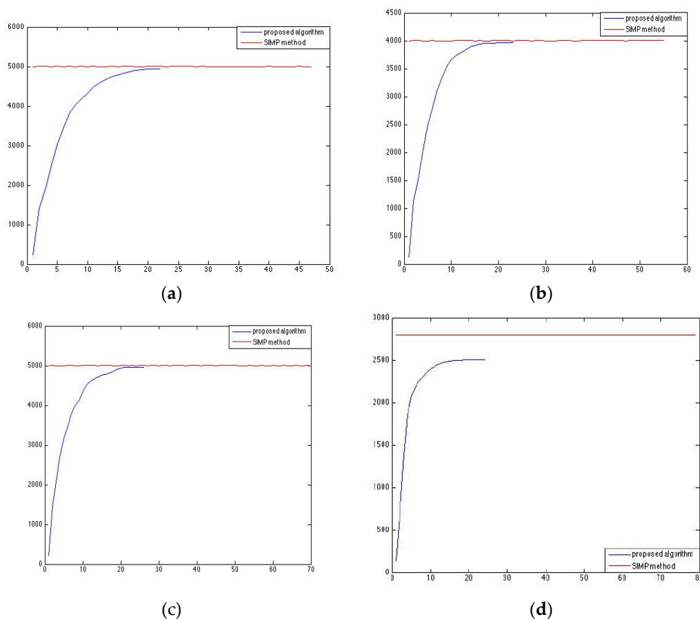
Figure 4. Convergence of volume in (a) cantiliver with load in middle, (b) cantiliver with load in corner, (c) half-MBB beam, and (d) L-shaped structure.
