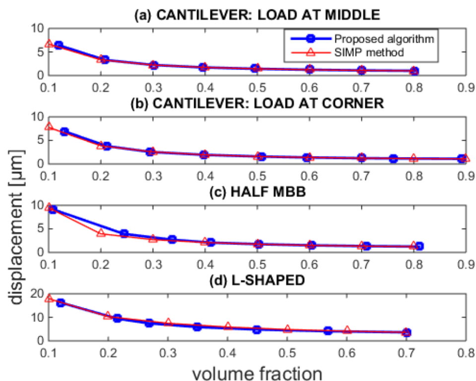
Figure 8. Comparison of the proposed algorithm with SIMP method for a variety of volume fractions in (a) cantilever with load in middle, (b) cantilever with load in corner, (c) half-MBB beam, and (d) L-shaped structure.
