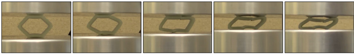
Figure 21. Experimental compression test of standard hexagonal cell under lateral load.
