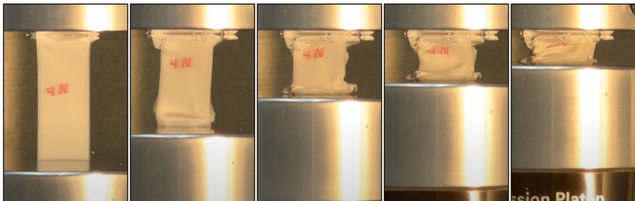
Figure 8. Experimental compression test of the novel cell under axial load during the different stages graphed in Figure 7: (a) First collapse; (b) Second collapse (c,d) Between 20 mm and 42 mm; and (e) Densification.
