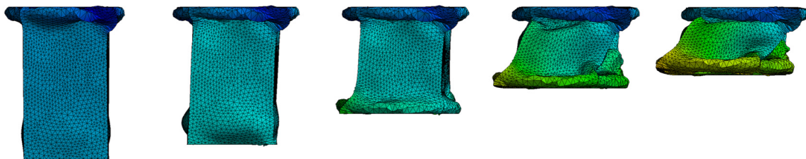
Figure 9. FE analysis of deformation process for the novel cell under axial load.
