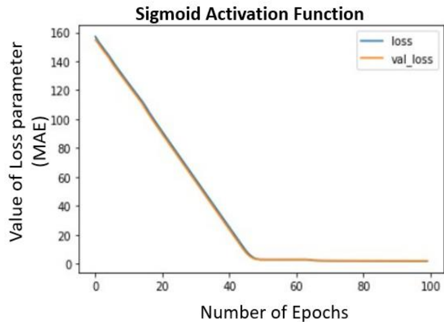
Figure 3. Training and Validation loss curves while training of the model using sigmoid activation function (x-axis represents the number of successive epochs and y-axis holds the value of loss parameter (MAE) for each epoch).
