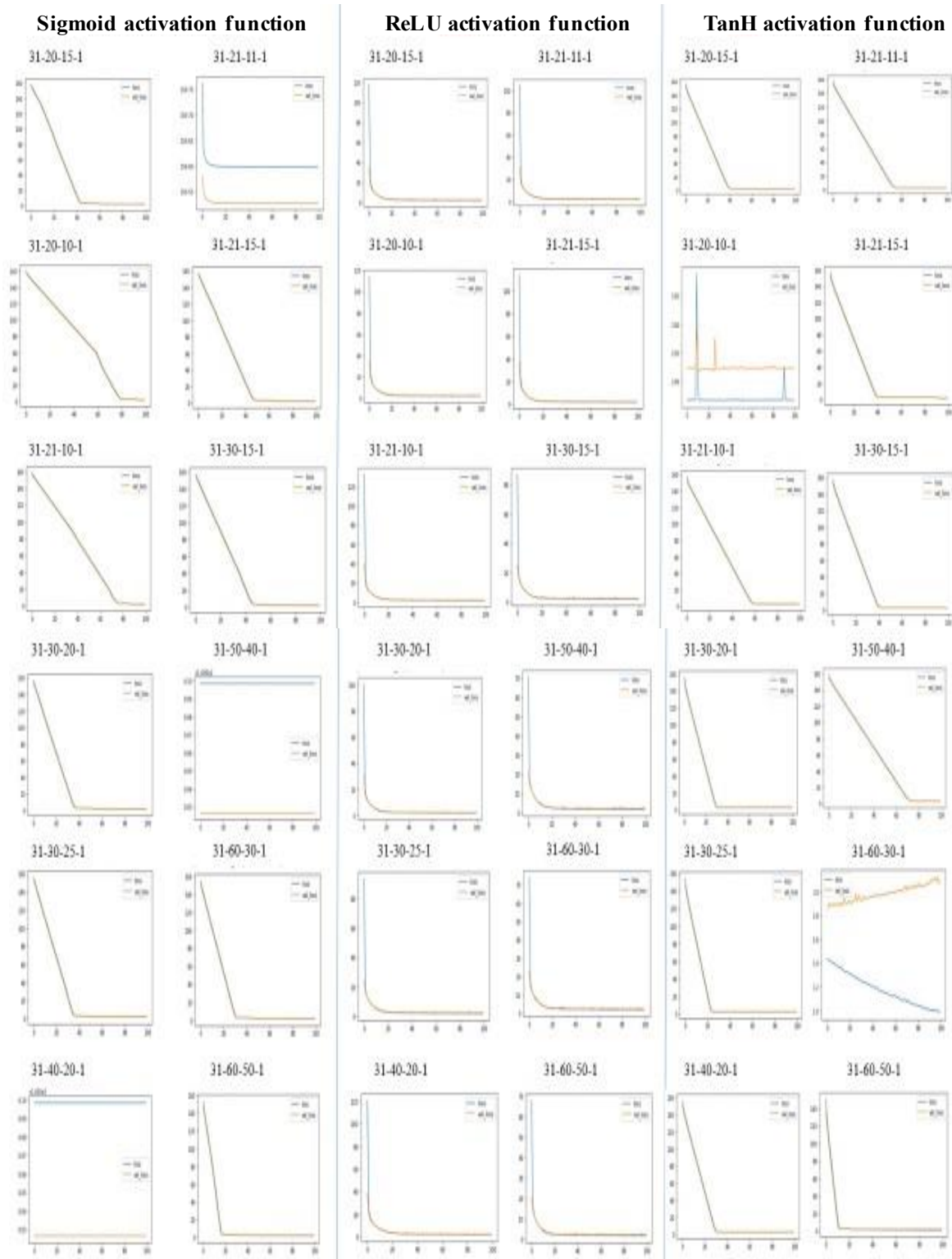
Figure A1. Training loss and Validation loss curves depicting the training performance of the models with three different activation functions for Ghaziabad and surrounding regions.
