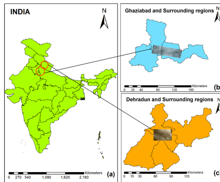
Figure 1. Study Area Map with overlay of DEMs to show the extent of study areas: (a) India; (b) Study Area 1: Ghaziabad and Surrounding regions; (c) Study Area 2: Dehradun and Surrounding regions.
