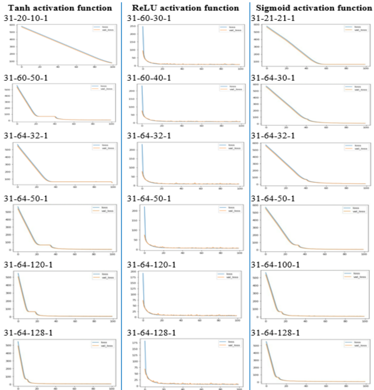
Figure A2. Training loss and Validation loss curves depicting the training performance of the models with three different activation functions for Dehradun and surrounding regions.
