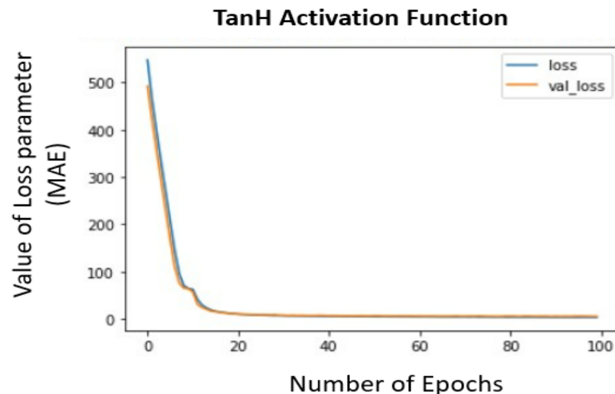
Figure 6. Training and Validation loss curves while training the model using TanH activation function (x-axis represents the number of successive epochs and the y-axis holds the value of loss parameter (MAE) for each epoch).
