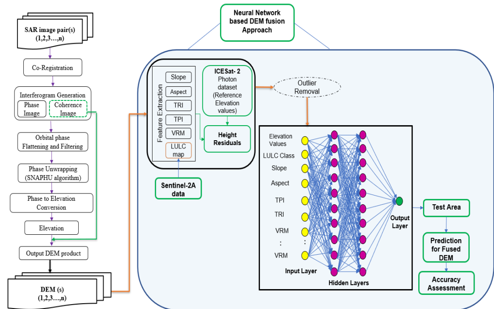
Figure 2. Workflow of the Neural Network-based Fusion Framework for DEM Improvement.
