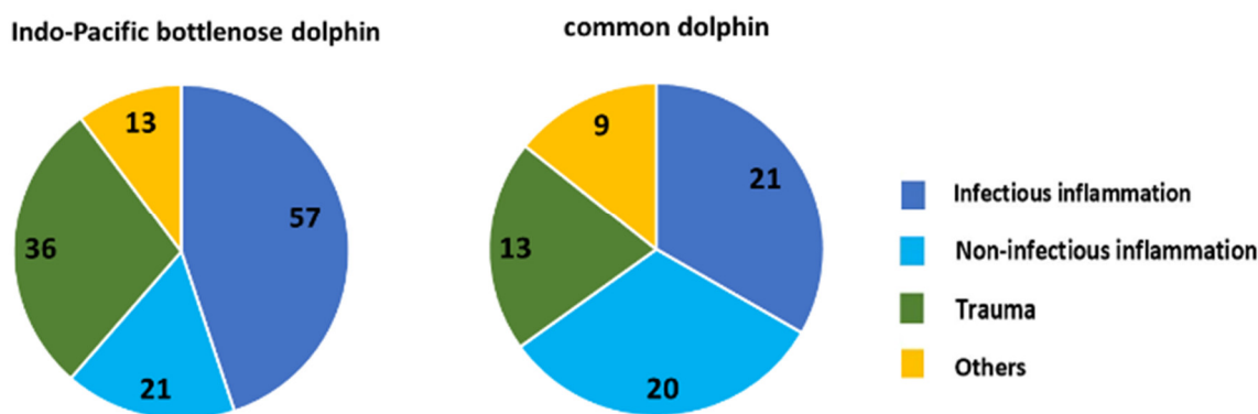
Figure 5. Proportional representation of the types of pathological changes in the Indo-Pacific bottlenose dolphin ( Tursiops aduncus ) and common dolphin ( Delphinus delphis ) from the St Vincent Gulf Bioregion, South Australia, during 2009–2020. Numbers are the counts of cases in each category.
