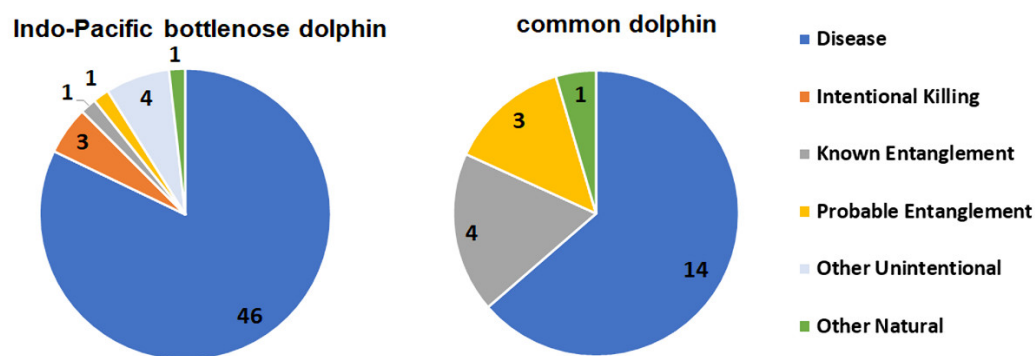
Figure 4. Proportional representation of circumstance of death categories for necropsied Indo-Pacific bottlenose dolphins ( Tursiops aduncus ) and common dolphins ( Delphinus delphis ) from the St
