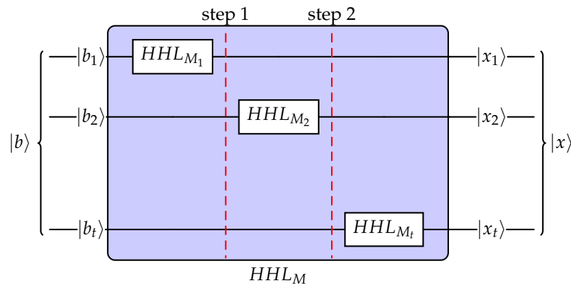
Figure 2. Vertical HHL scheme. We note that we actually apply a single HHL_{M_i} at a time in t steps. The register after step 1 is (HHL_{M_1} \otimes \bigotimes_{i=2}^t E_i) |b\rangle . The state in step 2 is (E_1 \otimes HHL_{M_2} \otimes \bigotimes_{i=3}^t E_i) \circ (M_1 \otimes \bigotimes_{i=2}^t E_i)^{-1} |b\rangle .
