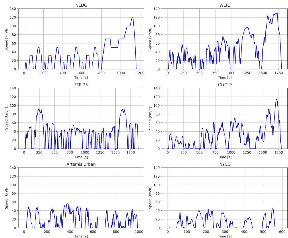
Figure 6. Speed profiles for six standard driving cycles.
