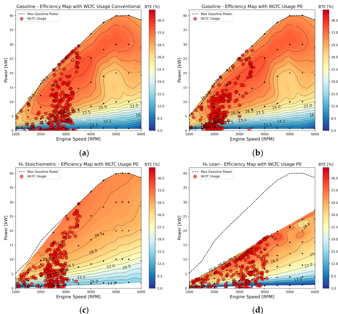
Figure 10. Engine use for gasoline conventional (a), gasoline P0 (b), stoichiometric H 2 P0 (c), and lean H 2 P0 (d) in the WLTC.
