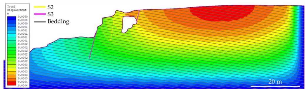
Figure 21. Displacement values resulting from geotechnical modeling along cross-section CC'.
