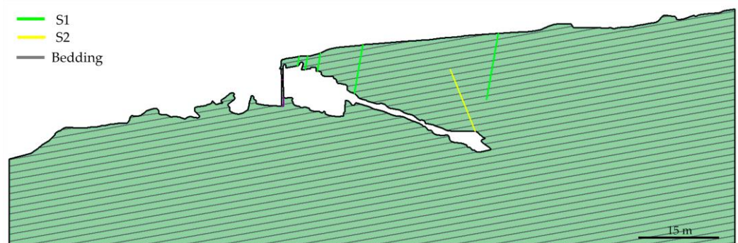
Figure 8. Geotechnical AA' cross-section; the green and yellow lines represent the main identified joints, while the gray lines indicate the limestone bedding.
