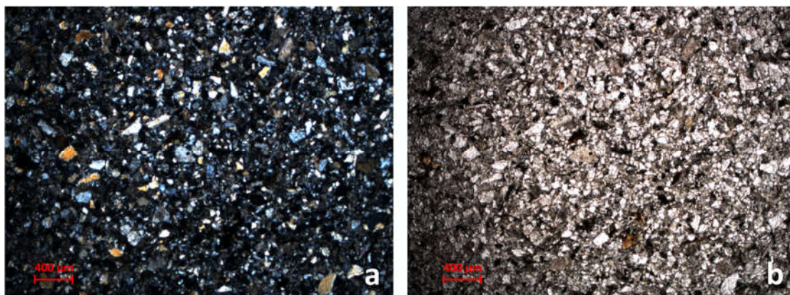
Figure 3. (a) GC sample image of the thin section in cross polarized light (xpl); (b) image in plane polarized light (ppl) of the same sample: in both images the medium-fine grain size of quartz and feldspars and the higher compactness of the rock are shown.
