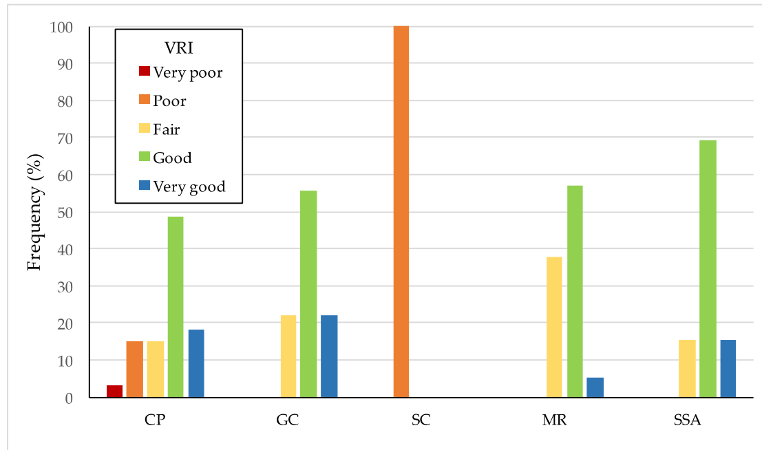
Figure 6. Percentage of Pietra Serena corbels of different qualities according to velocity ratio index (VRI).
