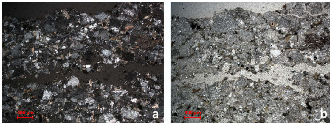
Figure 2. (a) SC sample image of the thin section in cross polarized light (xpl), showing the presence of cracks and fractures parallel to the surface; (b) image in plane polarized light (ppl) of the same sample where cracking and decohesion between the granules are evident.
