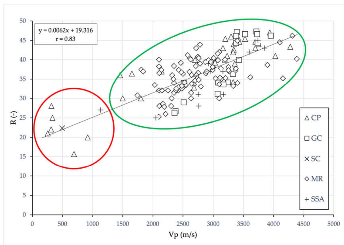
Figure 5. Ultrasonic velocity ( V_p ) versus rebound values ( R ) correlation; red cluster represents low V_p and R values corresponding to the most degraded corbels, while the green cluster represents high V_p and R values, which indicate a good state of preservation of Pietra Serena .
