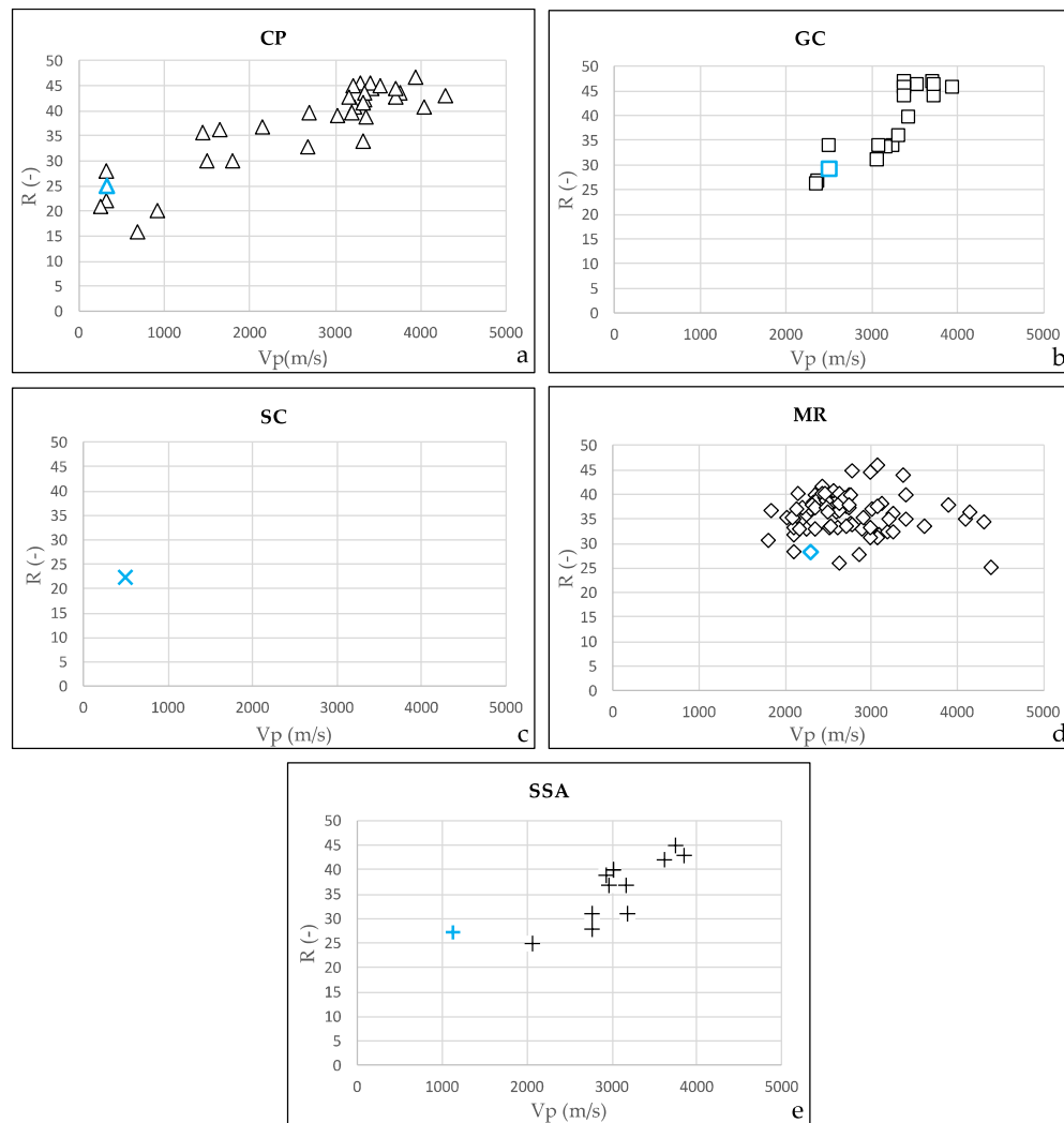
Figure 4. Ultrasonic velocity ( V_p ) versus rebound values ( R ). In blue the corbels selected for sampling. Results for (a) Palazzo Corsini Palace, (b) Ginori Conti Palace, (c) Santa Croce Basilica, (d) Medici Riccardi Palace and (e) Santissima Annunziata Basilica, corbels.
