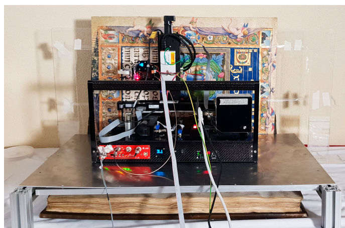
Figure 1. Setup for the XRF scanning system.
