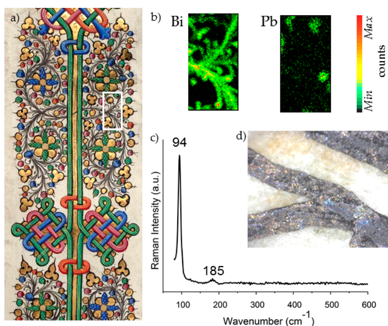
Figure 10. Identification of metallic bismuth in decorative borders: (a) Antiphonary Q, detail from folio 29v; (b) XRF maps of Bi-L \alpha and Pb-L \alpha in the area outlined in white in Figure 10a; (c) Raman spectrum of the black line within area outlined in white; (d) microscope image of the black line (original magnification 200X).
