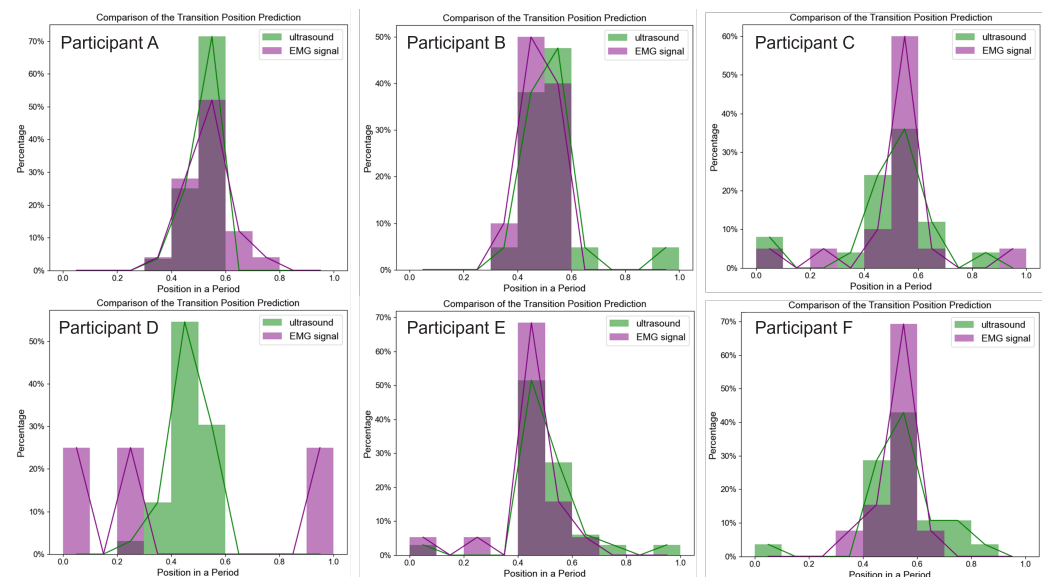
Figure 9. The histogram shows the transition locations of the two models' classifications (determined by the post-processing from the full sequence classification results), regardless of ground truth labels, and expressed as a percentage over the single motion cycle (e.g., 0.2 on the x-axis indicates the 20% position of a full cycle duration). The participants A to F are displayed in a zigzag order from top left to bottom right. The lines connect the peak values of the bars within each distribution slot, illustrating the slot distribution from each participant. The post-processing steps to obtain the transition locations from the models are described in Section 3.2.
