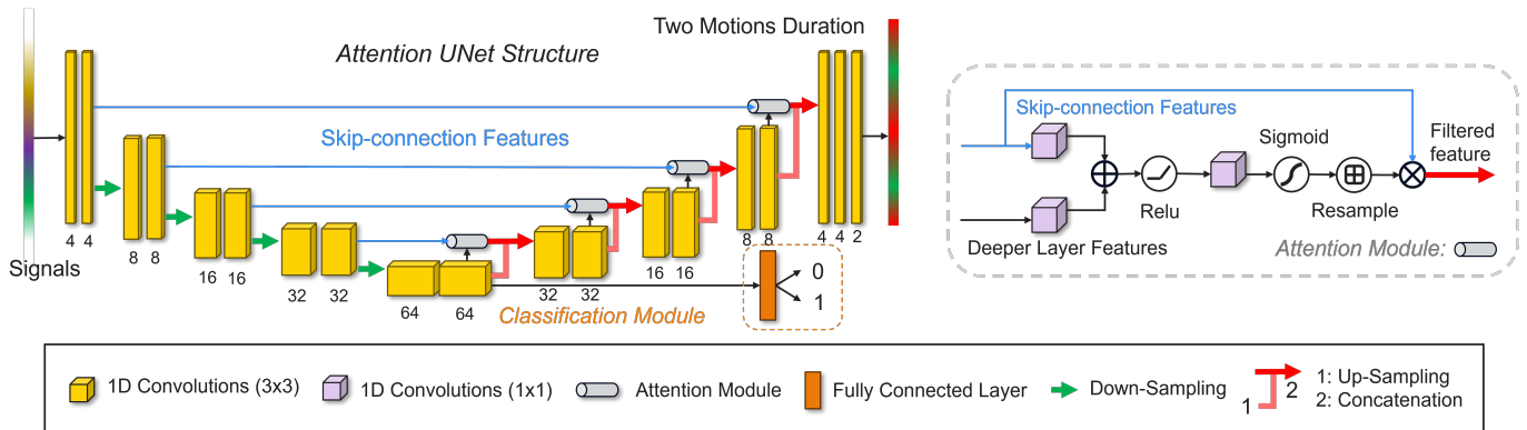
Figure 5. The proposed attention UNet for predicting the arm movement phase using ultrasound signals. The input is the recorded bio-signals, while the output from the encoder is the classification of movement transitions, and the final output is the motion types throughout the full sequence (red and green represent the two motion phases). The attention module has a horizontal cylindrical shape and is demonstrated on the right in detail.
