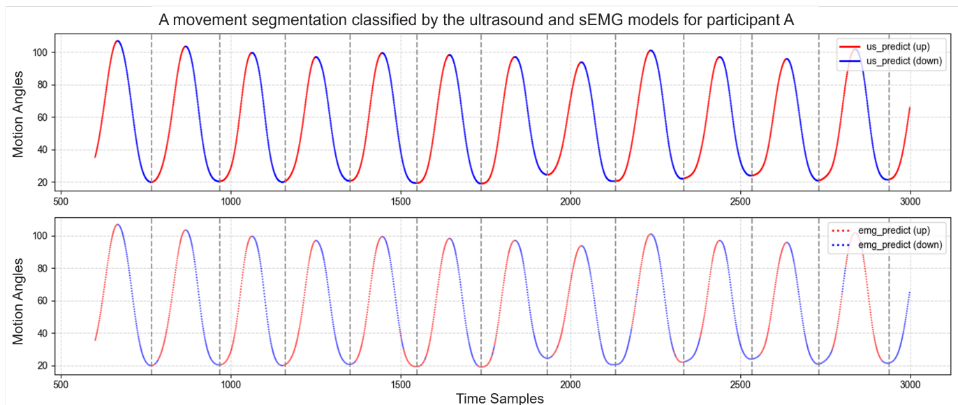
Figure 6. This shows the classification results from the two models of participant A. A random segment of the motion cycles was selected from the test dataset, which contains several motion cycles (due to the repeatable motion). The solid curves represent the prediction results from the ultrasound model, while the dotted curves represent the results from the EMG model. The red color represents the class of lowering the arm, while the blue color represents the class of lifting the arm. The gray vertical dashed lines represent the prediction positions from the ultrasound model.
