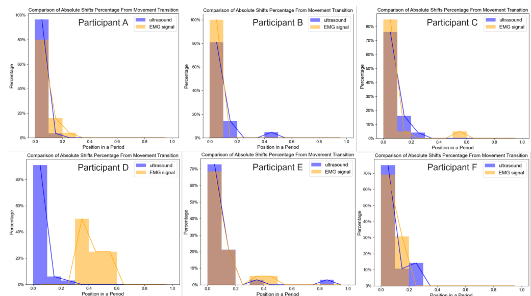
Figure 8. The histograms show the distribution of the absolute shift errors between the transition locations of models' classifications (determined by the post-processing from the full sequence classification results) and the transition locations from the ground truth labels, expressed as a percentage of the full motion cycle duration (e.g., 0.2 on the x-axis indicates an error of 20% of the full cycle duration). The results of participants A to F are arranged from top left to bottom right in a zigzag pattern. The lines connect the peak values of the bars within each distribution slot. The brown color represents the overlapping areas between the results of ultrasound and EMG models. The post-processing steps to obtain the transition locations from the models are described in Section 3.2.
