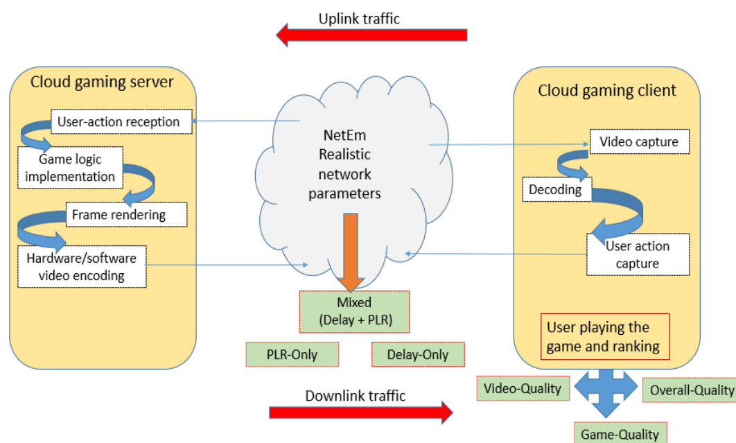
Figure 3. Block diagram of processes taking place on the client and server side and the flow of traffic.
