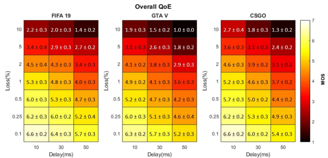
Figure 10. Heatmap of O-QoE (MOS with Confidence Intervals) for mixed network scenarios.
