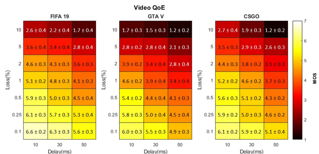
Figure 8. Heatmap of V-QoE (MOS with Confidence Intervals) for mixed network scenarios.
