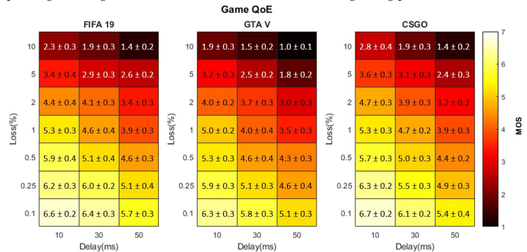
Figure 9. Heatmap of GP-QoE (MOS with Confidence Intervals) for mixed network scenarios.
