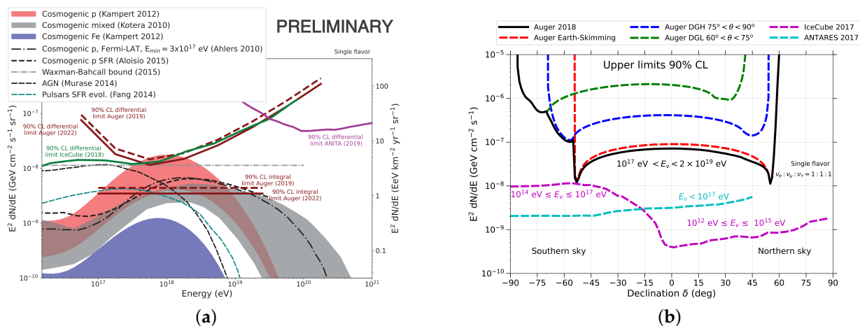
Figure 1. (a) Diffuse neutrino flux upper limits (integral: straight lines, differential: curved lines) compared with expectations from [3]. (b) and declination dependent “point-source” flux upper limits from [5].
