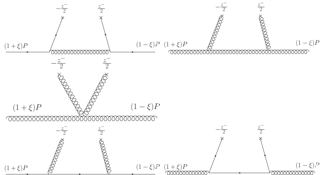
Figure 6. Feynman diagrams used to compute the one-loop anomalous dimension in the lightcone gauge. On the first and second lines, we display non-mixing terms, while the third line display diagrams mixing quark and gluon GPDs. On top of these connected diagrams, disconnected self-energy diagrams need to be added. In covariant gauges, additional contributions come from gluon exchanges with the Wilson line.
