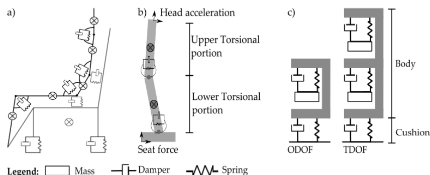
Figure 3. Representation of the mechanical models developed by Kawai et al. and Mastuoka et al. (a) Brown et al. (b), and Garcia-Mendez et al. (c).
