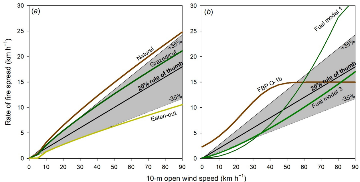
Figure 6. Model predictions of rate of fire spread as a function of 10 m open wind speed on level ground for the 20% rule of thumb in contrast to those fire spread models used operationally in Australia and North America and the \pm 35\% error prediction intervals as per [40]. This includes the following: (a) the three grassland fuel condition types (natural, grazed or cut and eaten-out) in southern Australia of [10]; and (b) fuel type O-1b (standing grass) in the Canadian Forest Fire Behavior Prediction (FBP) System [43,44] and the Rothermel [45] model as implemented in the US BehavePlus Fire Modeling System [46] for two of the three grass fuel models (1—short grass (0.3 m); 3—tall grass (0.75 m)) found in [47] based on a wind adjustment factor of 0.4 [48]. Simulations assume a 100% degree of curing and a fine dead fuel moisture content of 3.7% (the average in the database used in the present study analysis).
