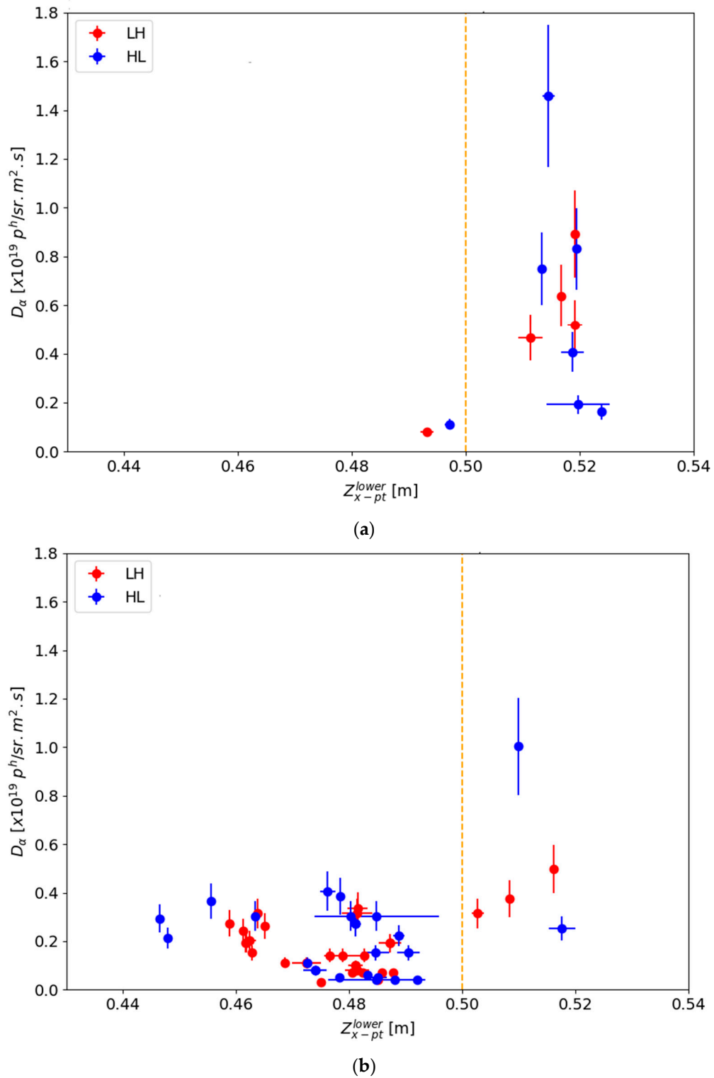
Figure 6. Divertor D_\alpha intensity at the L–H and H–L transitions plotted as a function of lower X-point height distance from the divertor floor for (a) I_p = 0.67\text{--}0.75 MA and (b) I_p = 0.75\text{--}0.77 MA.
