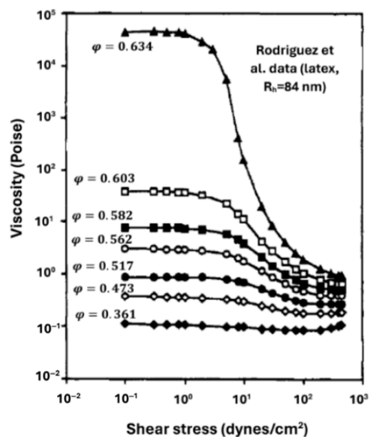
Figure 66. Viscous behaviour of Brownian suspensions of latex 84. Adapted from [60].
