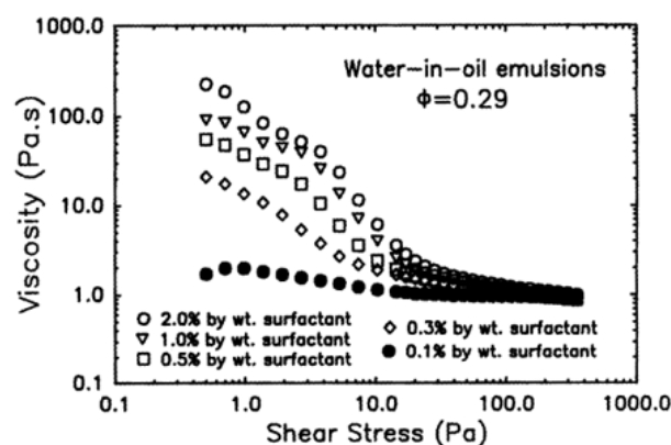
Figure 73. Viscous behaviour of micelle-induced depletion-flocculated emulsions at different surfactant concentrations.
