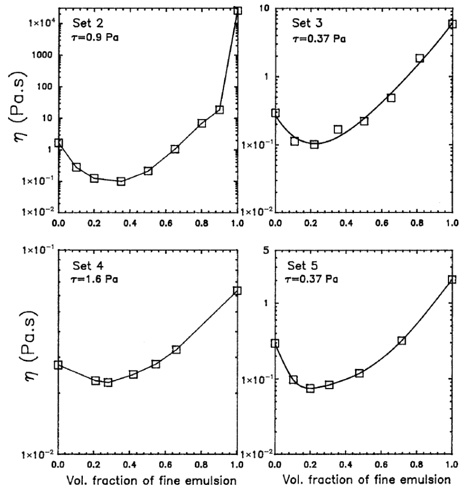
Figure 19. Viscosity versus fine emulsion content of a bimodal emulsion. The data shown in Figure 19 is obtained from Figure 18. The droplet size information is given in Table 1. The \phi values for various sets shown are as follows: Set 2 ( \phi = 0.745 ), Set 3 ( \phi = 0.71 ), Set 4 ( \phi = 0.63 ), and Set 5 ( \phi = 0.70 ).
