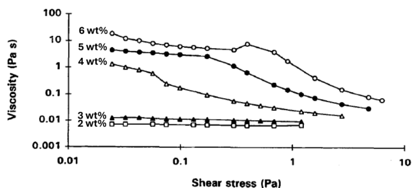
Figure 76. Pseudoplastic behaviour of protein-flocculated emulsion at different protein concentrations (35 vol% n-tetradecane, pH 6.8, 30 ^{\circ}\text{C} ). Adapted from [67].
