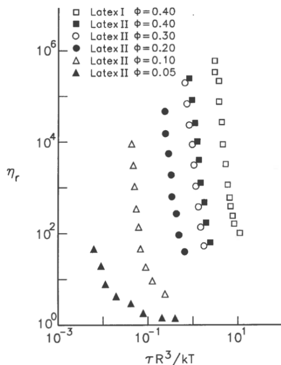
Figure 51. Viscous behaviour of electrically charged suspensions at different values of \phi . Adapted from [48].
