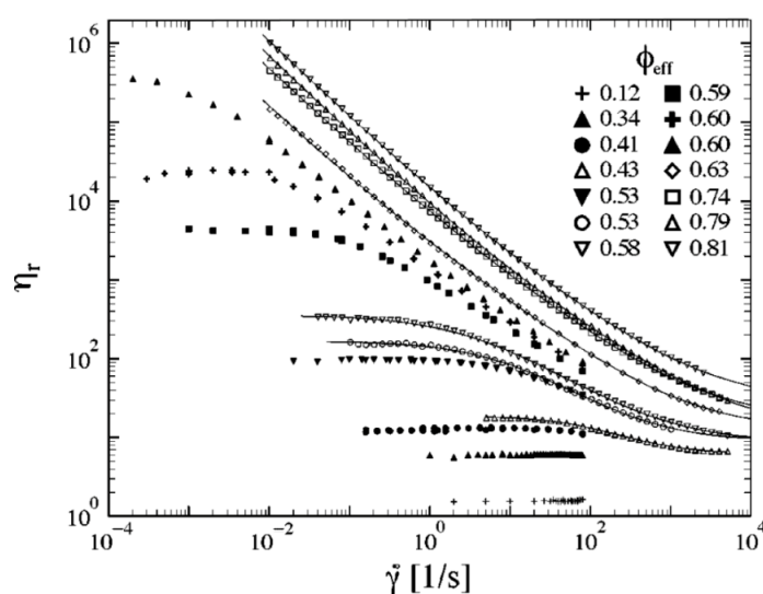
Figure 58. Viscous behaviour of sterically stabilized suspensions at different values of \phi . Adapted from [52].
