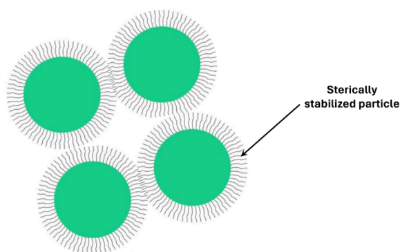
Figure 59. Merging of steric layers of neighbouring particles and crowding of particles at high \varphi .
