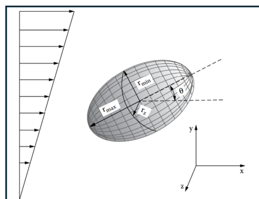
Figure 30. Deformed droplet in shear flow.
