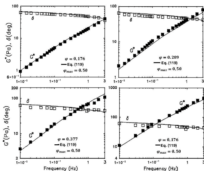
Figure 88. Comparisons between theoretical predictions (Pal model, Equation (119)) and experimental data of G^* and \delta of non-dilute suspensions.
