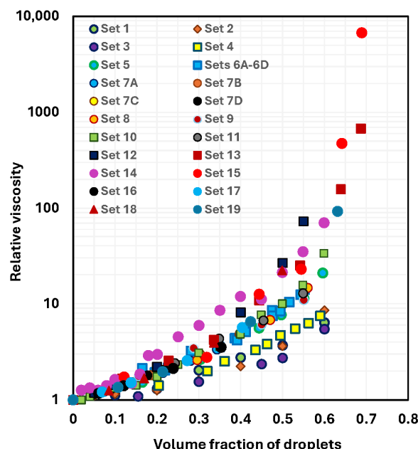
Figure 11. Data of emulsions collected from different sources.
