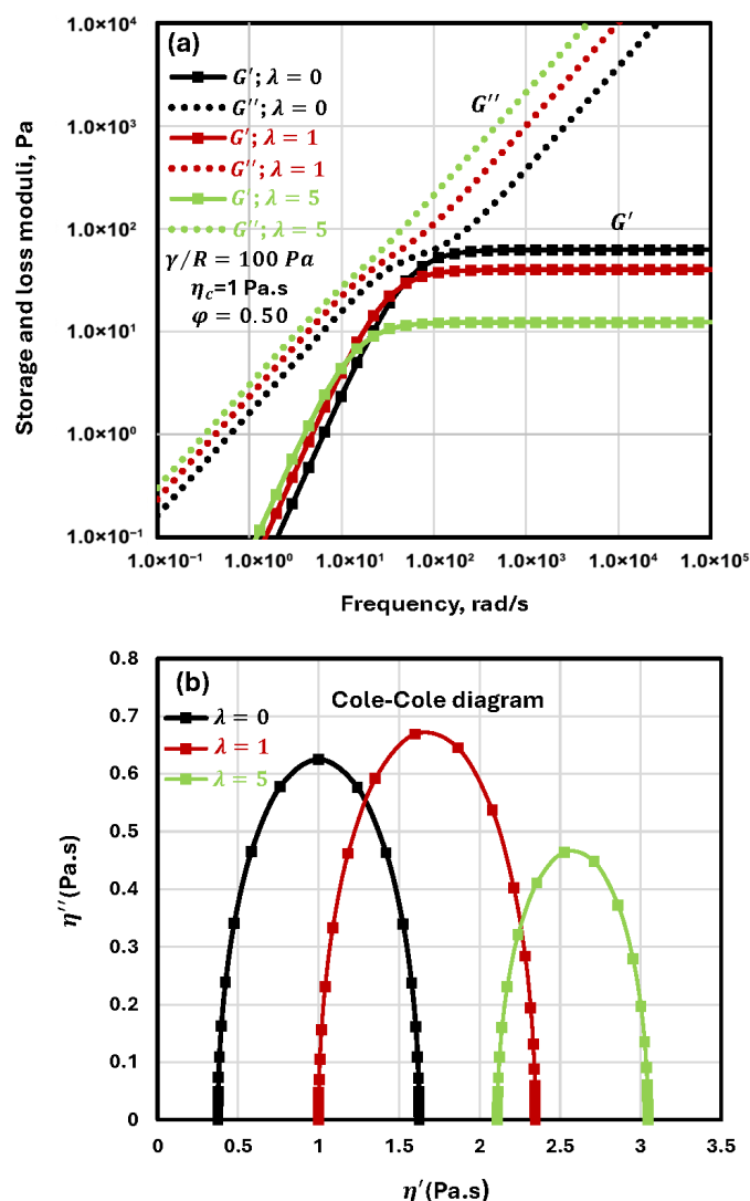
Figure 84. Moduli and Cole–Cole plots of a non-dilute emulsion ( \phi = 0.50 ) generated from the Palierne model (Equation (107)) for different values of \lambda .
