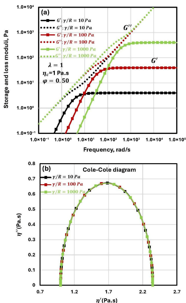
Figure 83. Moduli and Cole–Cole plots of a non-dilute emulsion ( \varphi = 0.50 ) generated from the Palierne model (Equation (107)) for different values of interfacial stress \gamma/R .
