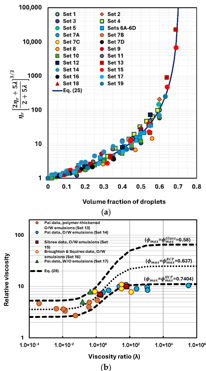
Figure 17. (a) Comparison between data and model predictions given by Equation (25). (b) Comparison of experimental viscosity and the prediction of Equation (25) at a fixed \phi of 0.5 but varying \lambda .
