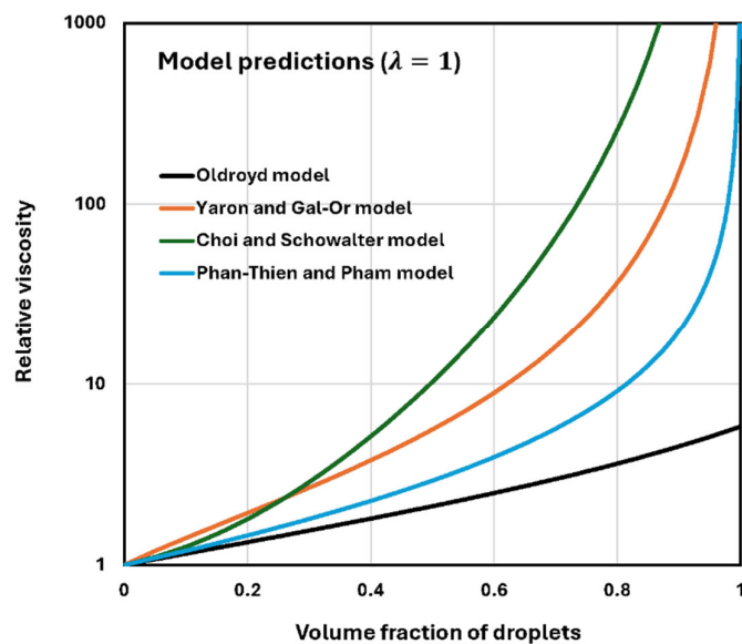
Figure 2. Comparison of relative viscosity versus volume fraction ( \phi ) plots predicted by different models when the viscosity ratio is unity.
