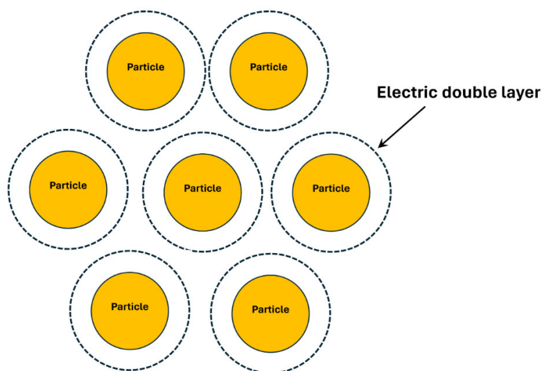
Figure 52. Merging electrical double layers of neighbouring particles and crowding of particles at high \phi .
