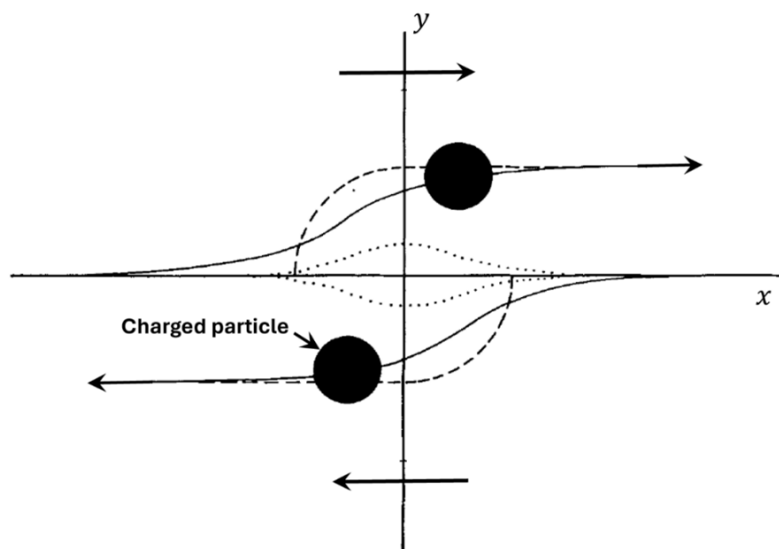
Figure 46. Trajectories of particles in flow. .... denotes uncharged particles with hydrodynamic interactions; — denotes charged particles without hydrodynamic interactions; and --- denotes paths of charged particles according to Chan et al. [45]. Adapted from [39].
