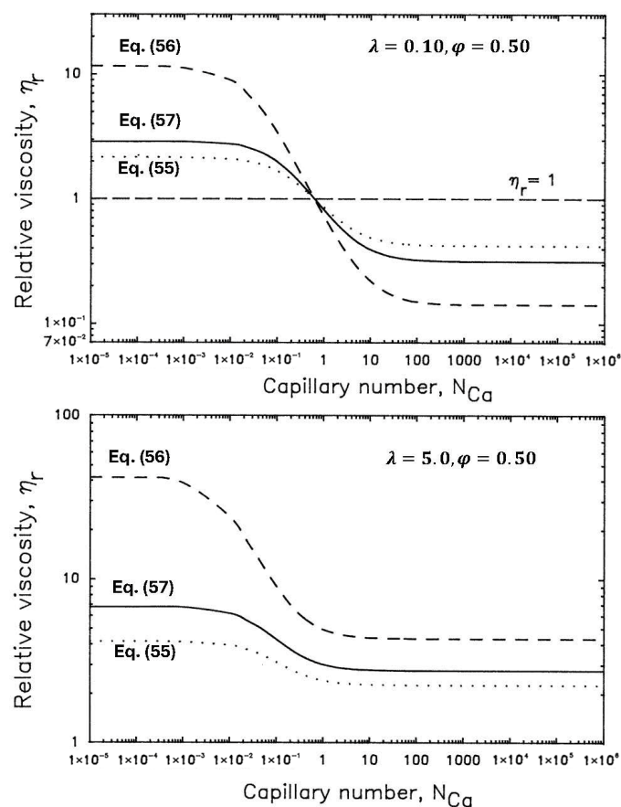
Figure 32. Relative viscosity versus capillary number predicted by Equations (55)–(57) at \phi = 0.50 . The \phi_{max} used is 0.637 in calculations.
