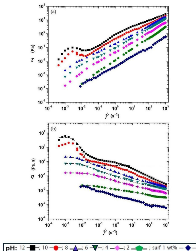
Figure 47. The evolution of flow curves of O/W emulsions with pH. (a) Shear stress versus shear rate. (b) Viscosity versus shear rate. Adapted from [46].
