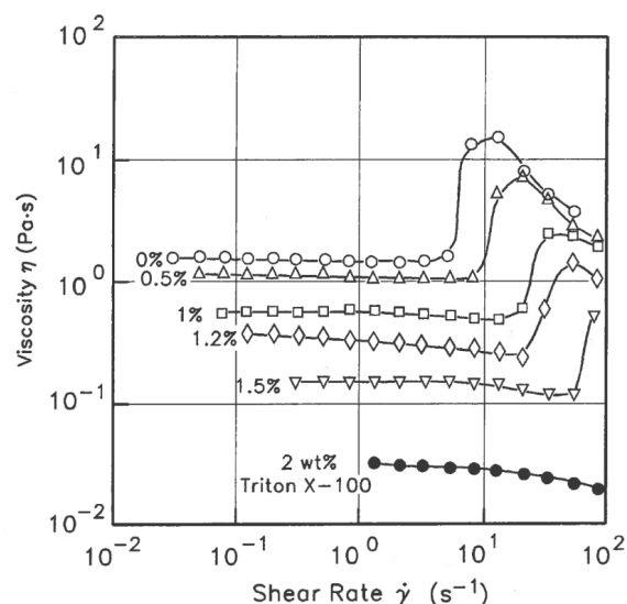
Figure 81. Influence of surfactant on the rheological behaviour of suspension flocculated by polymer bridges. The \phi is 0.15 and the polymer is polyacrylic acid at a concentration of 2 wt%. Adapted from [70].
