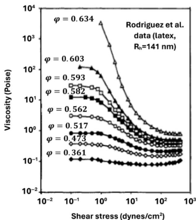
Figure 65. Viscous behaviour of non-dilute Brownian suspensions of latex 141. Adapted from [60].
