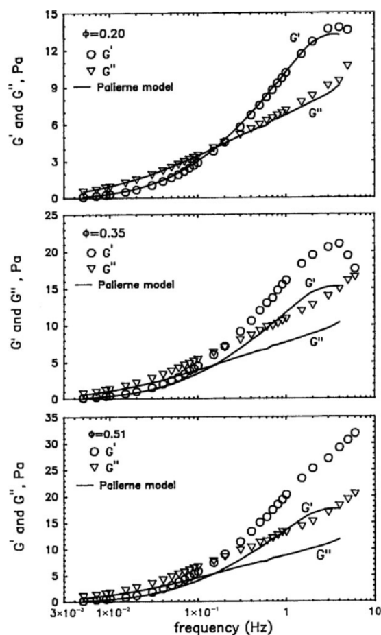
Figure 85. Comparisons between theoretical predictions (Palierne model, Equation (96)) and data of storage and loss moduli of non-dilute O/W emulsions.
