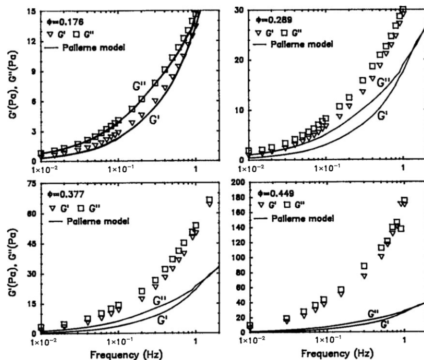
Figure 86. Comparisons between theoretical predictions (Palierne model, Equation (96)) and experimental data of storage and loss moduli of non-dilute suspensions.
