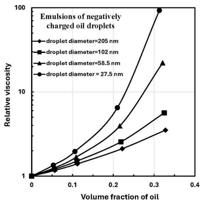
Figure 42. Relative viscosity of electrically charged non-dilute emulsions.
