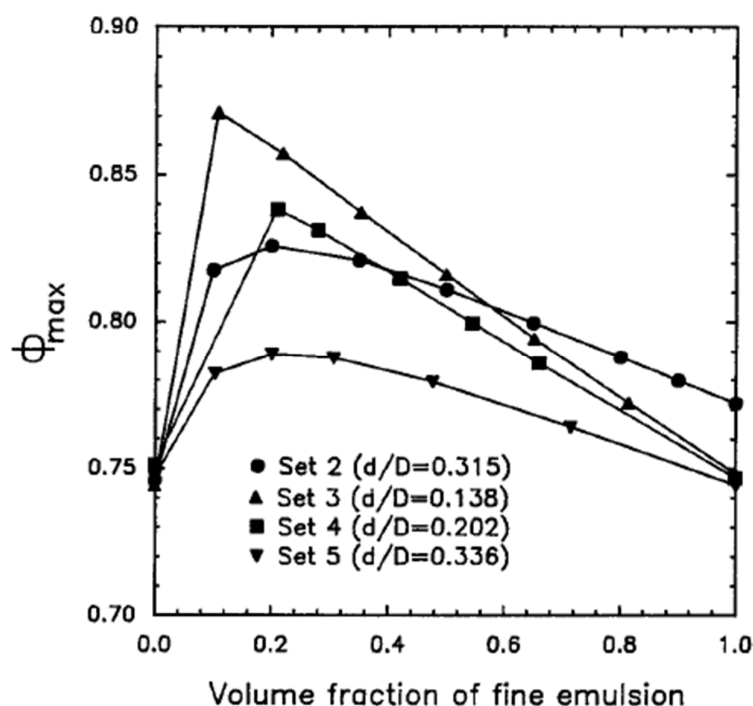
Figure 20. Variation of \varphi_{max} with fine emulsion content of bimodal emulsions, as predicted by the Ouchiya and Tanaka theory.
