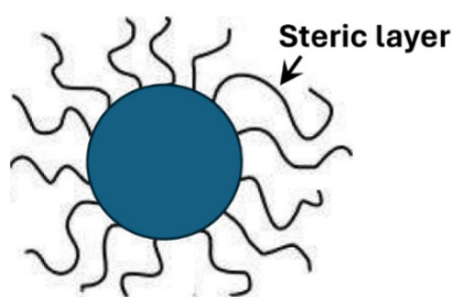
Figure 56. Droplet covered by a steric layer.
