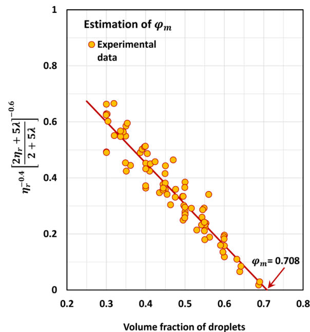
Figure 12. \varphi_{max} estimation.
