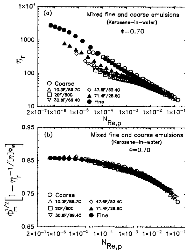
Figure 29. Correlation of \eta_r and \phi_m^{1/2} [1 - \eta_r^{-1/\phi_{\max}[\eta]}] as a function of N_{Re,p} for bimodal emulsions at \phi = 0.70 . (a) \eta_r versus N_{Re,p} . (b) \phi_m^{1/2} [1 - \eta_r^{-1/\phi_{\max}[\eta]}] versus N_{Re,p} .
