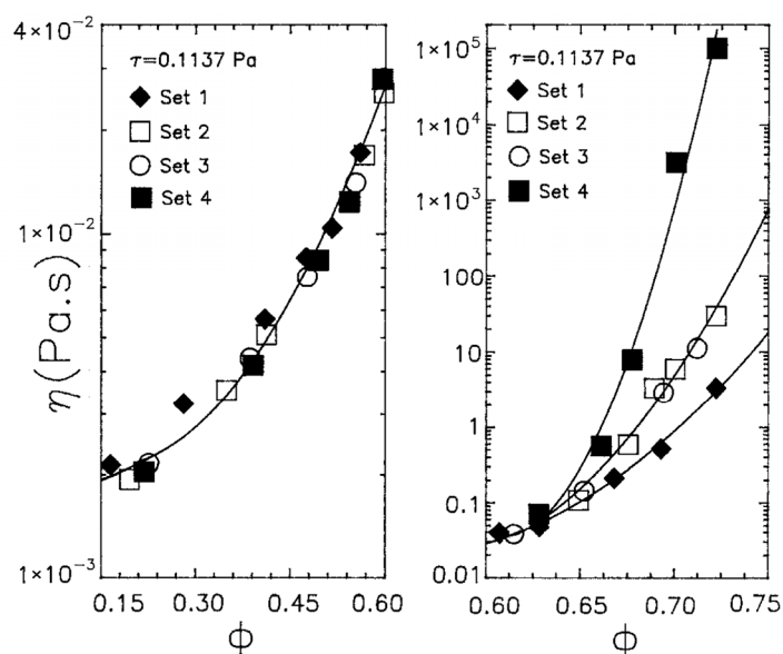
Figure 5. Zero-shear (low-shear-stress) viscosity versus \phi for different sets with different droplet diameters.
