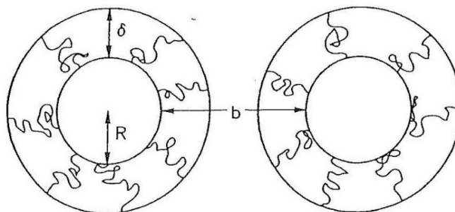
Figure 57. Interaction between droplets covered by steric layers.
