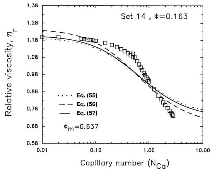
Figure 36. Comparison between model predictions and data of \eta_r as a function of N_{Ca} .
