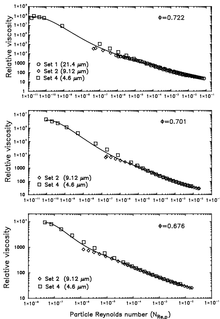
Figure 25. Scaling of relative viscosity with N_{Re,p} .
