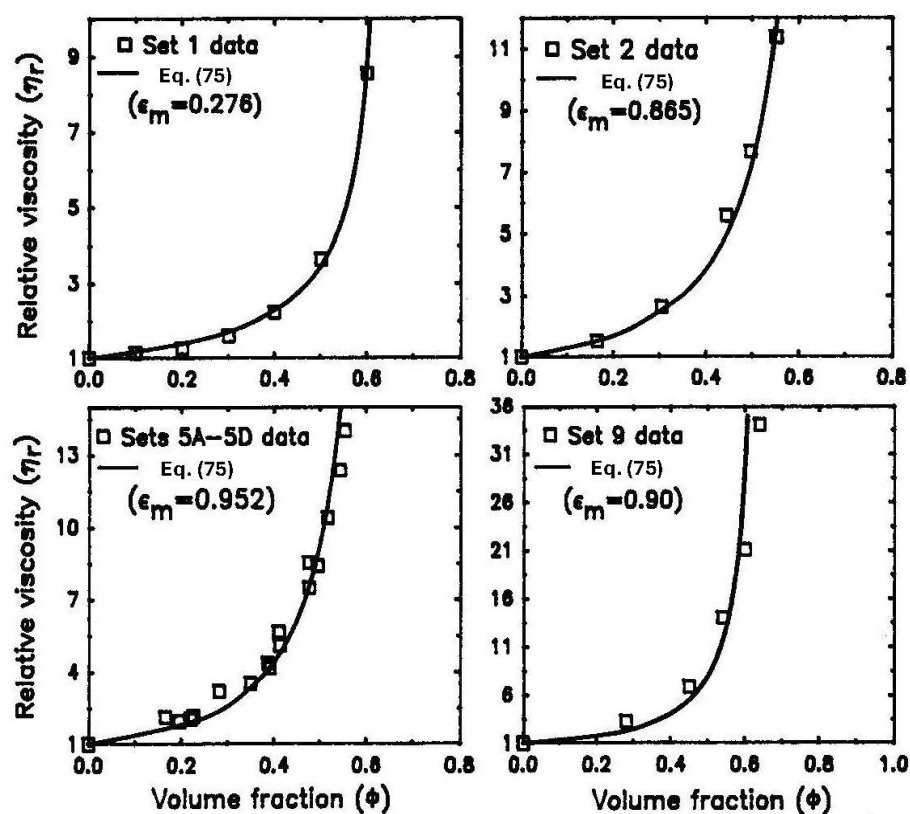
Figure 39. Comparisons between data and predictions of Equation (75).
