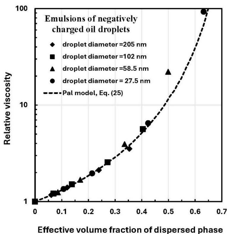
Figure 45. Scaling of \eta_r of electrically charged non-dilute oil-in-water emulsions with respect to \varphi_{eff} .
