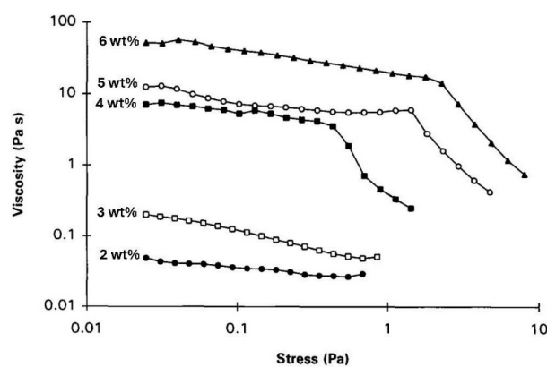
Figure 77. Effect of protein content on viscosity of depletion-flocculated O/W emulsions (45 vol% n-tetradecane, pH 6.8, 30 ^{\circ}\text{C} ). Adapted from [68].
