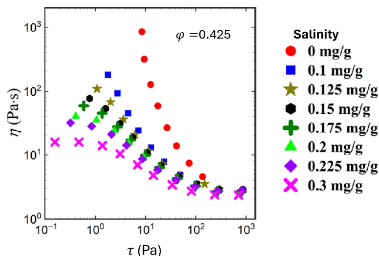
Figure 49. Viscous behaviour of suspensions of charged particles at \phi of 0.425. Adapted from [47].
