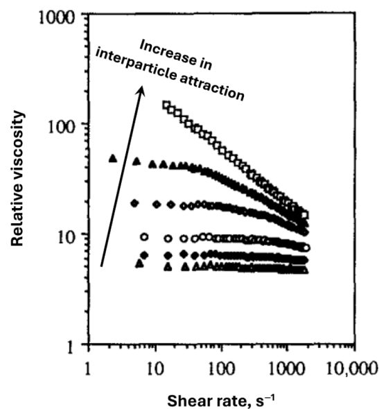
Figure 63. The effect of increasing interparticle attraction on the viscous behaviour of a suspension. Adapted from [56].
