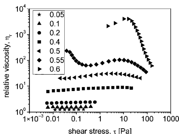
Figure 61. Viscous behaviour of Pickering emulsions at \phi . Adapted from [54].
