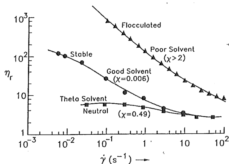
Figure 64. The influence of solvent quality on the steric layer, and hence the relative viscosity, on a sterically stabilized suspension where \chi is the Flory–Huggins interaction parameter. Adapted from [57,58].
