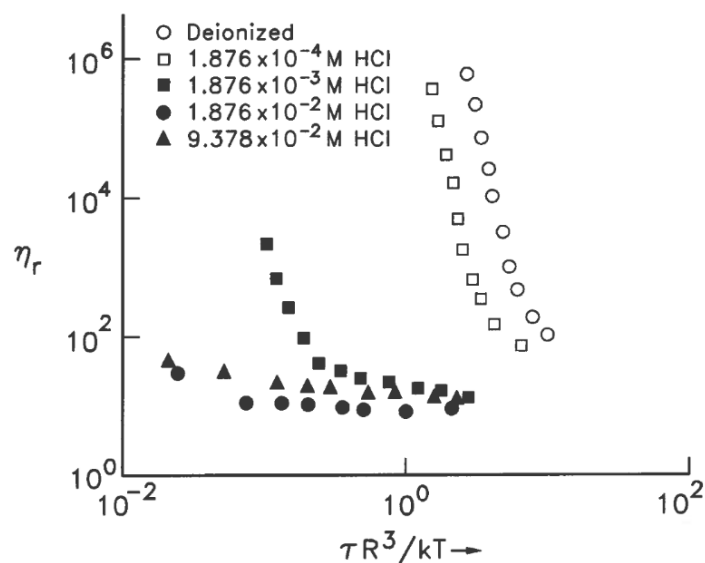
Figure 50. Viscous behaviour of electrically charged suspensions at \phi = 0.40 . Adapted from [48].
