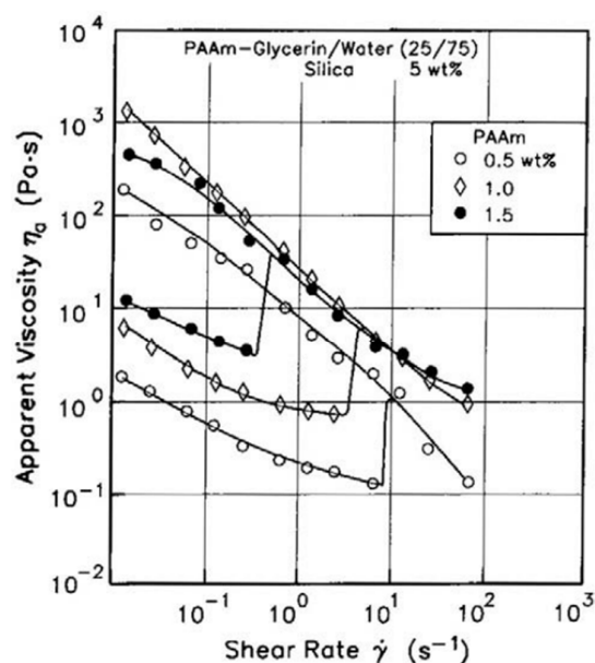
Figure 80. Viscous behaviour of suspensions at different polymer concentrations, keeping the particle concentration fixed at 5 wt% silica. Adapted from [70].
