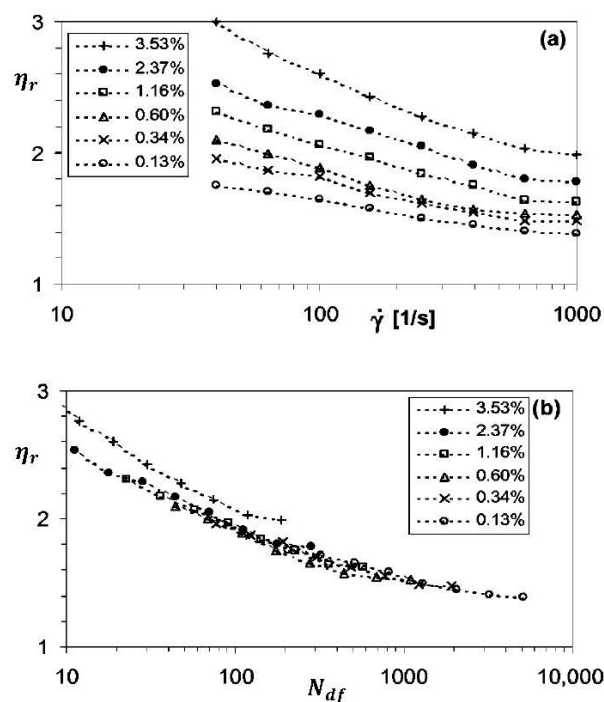
Figure 75. Effect of surfactant concentration on the relative viscosity of a W/O emulsion. (a) \eta_r versus shear rate. (b) \eta_r versus depletion flow number N_{df} . The numbers in the plots indicate volume fractions of surfactant (sorbitan monostearate). The value of \phi is 0.15 and the Sauter mean diameter of the emulsions is 3 \mu\text{m} . Adapted from [66].
