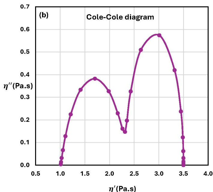
Figure 91. Dynamic rheology of an emulsion with viscoelastic oil–water interfaces. The plots are generated from the generalized Paliarne model. (a) Storage and loss moduli. (b) Cole-Cole diagram.
