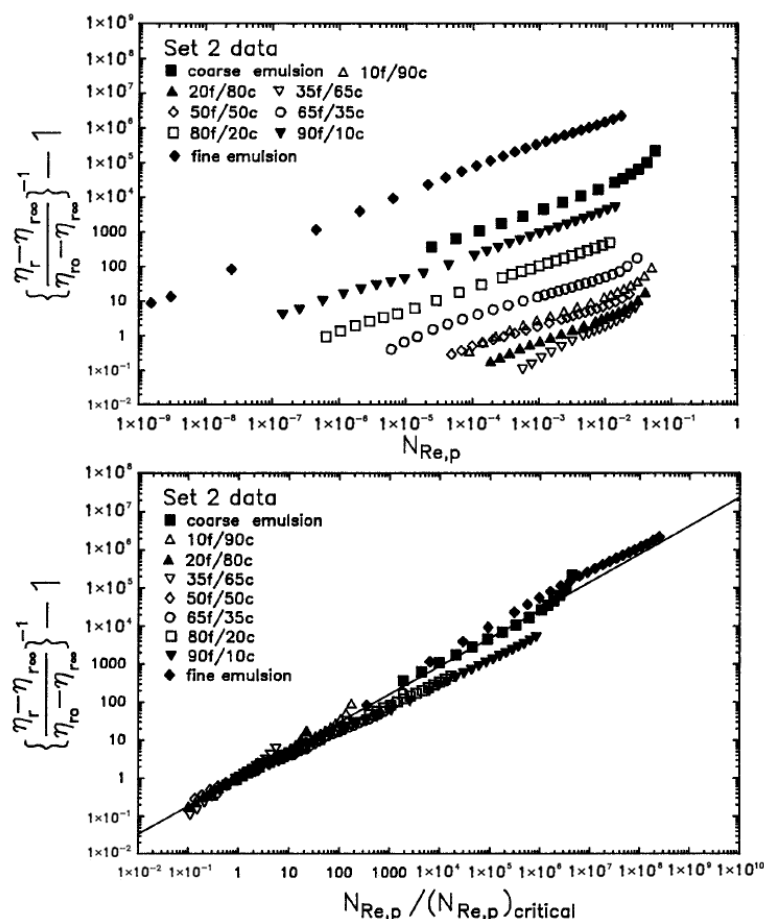
Figure 28. [(\eta_r - \eta_{r0})/(\eta_{r0} - \eta_{r00})]^{-1} - 1 versus N_{Re,p} and N_{Re,p}/(N_{Re,p})_{critical} for bimodal emulsions at \varphi = 0.745 .
