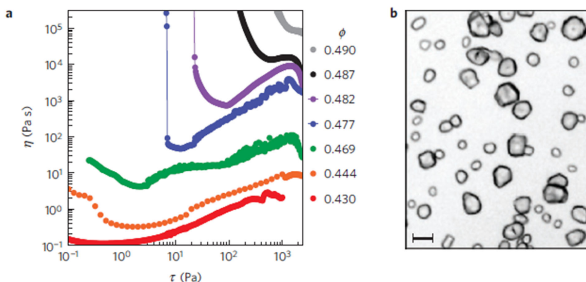
Figure 55. Yield stress and shear-thickening in suspensions. (a) Viscosity curves for cornstarch in water at different \phi . The cornstarch particles have an average diameter of 14 \mu\text{m} . (b) The microscope image of cornstarch particles, indicating the absence of clustering of particles. Adapted from [50].
