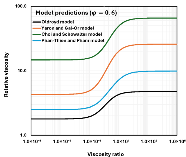
Figure 3. Comparison of \eta_r versus \lambda plots predicted by different models ( \phi = 0.6 ).
