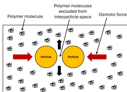
Figure 69. Flocculation of particles caused by polymer-induced depletion.
