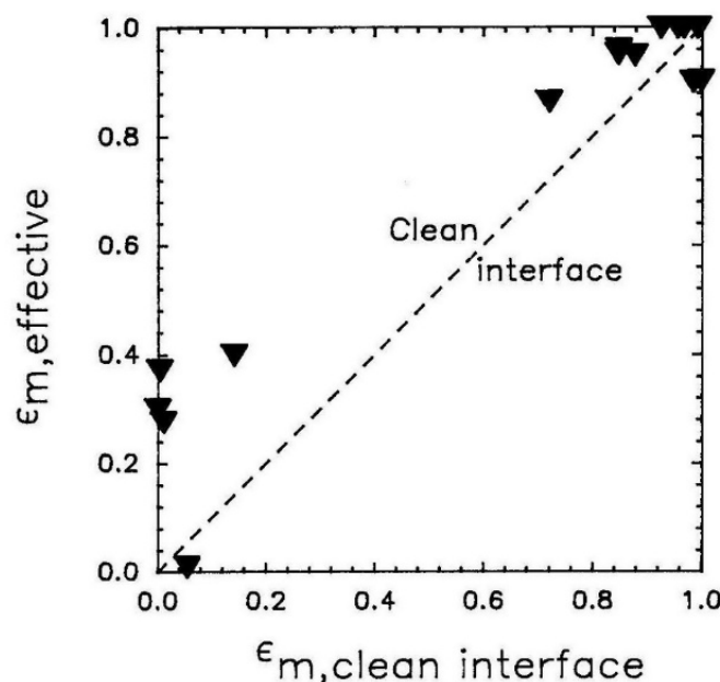
Figure 40. Plot of effective \epsilon_m versus \epsilon_{m, \text{clean}} , where \epsilon_{m, \text{clean}} is calculated from the viscosity ratio \epsilon_{m, \text{clean}} = \eta_r / (1 + \lambda) . Note that \epsilon_{m, \text{clean}} = 0 corresponds to bubbles with clean interface and \epsilon_{m, \text{clean}} = 1 corresponds to high viscosity droplets with clean interface.
