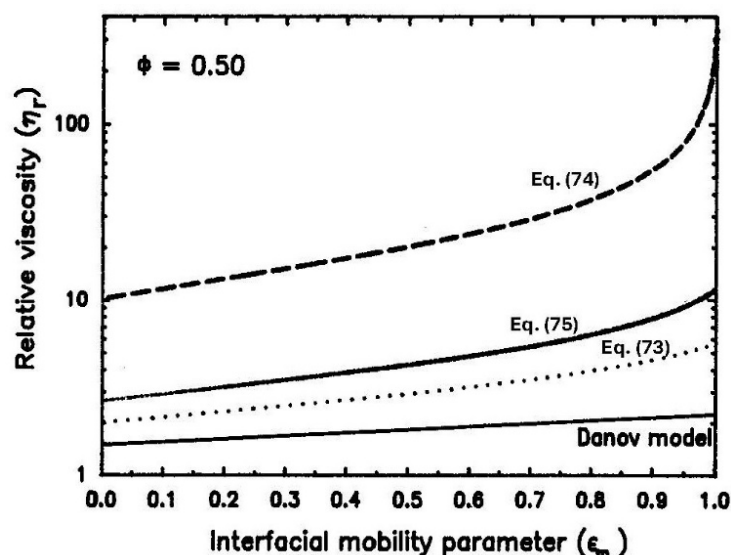
Figure 37. Predictions of \eta_r as a function of \varepsilon_m from the models expressed in Equations (70) and (73)–(75). The emulsion \varphi is 0.5.
