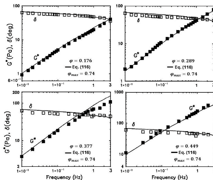
Figure 87. Comparisons between theoretical predictions (Pal model, Equation (116)) and experimental data of G^* and \delta of non-dilute suspensions.
