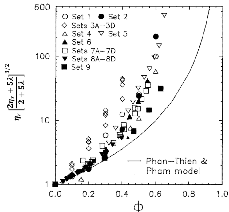
Figure 7. Comparison of experimental viscosity data on emulsions with the predictions of Equation (11).
