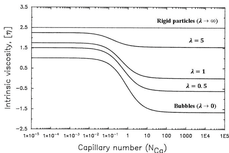
Figure 31. The effect of \lambda on emulsion [\eta] .
