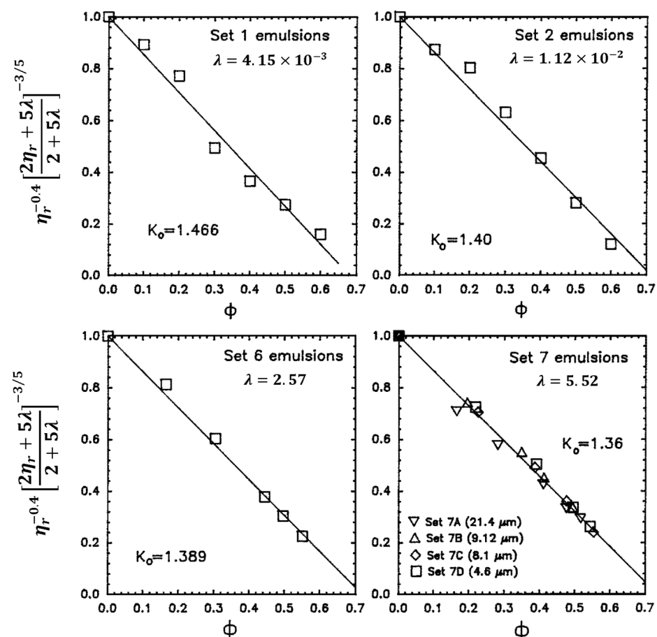
Figure 8. Experimental verification of Equation (13).
