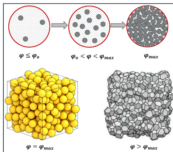
Figure 1. Variations in microstructure of emulsion with increase in \varphi .
