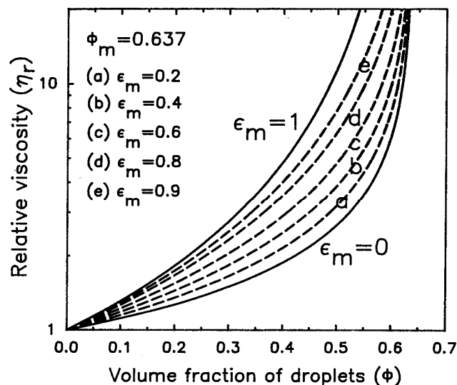
Figure 38. Relative viscosity predicted from Equation (75) for different \varepsilon_m .
