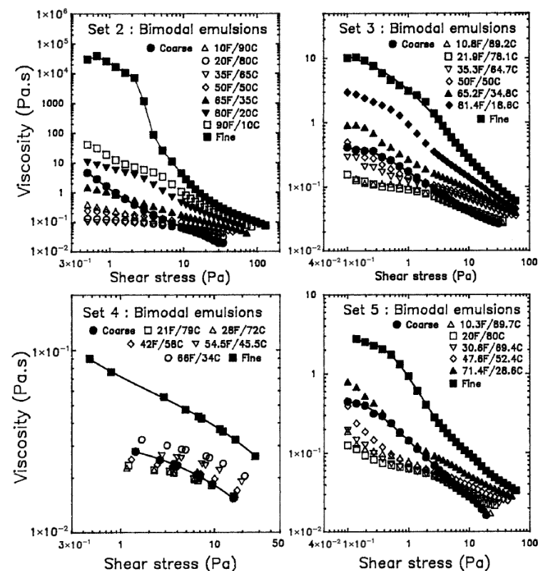
Figure 18. Viscosity plots of bimodal emulsions. Fine and coarse monomodal emulsions are mixed in various proportions at the same \phi . The \phi values for various sets shown are as follows: Set 2 ( \phi = 0.745 ), Set 3 ( \phi = 0.71 ), Set 4 ( \phi = 0.63 ), and Set 5 ( \phi = 0.70 ).
