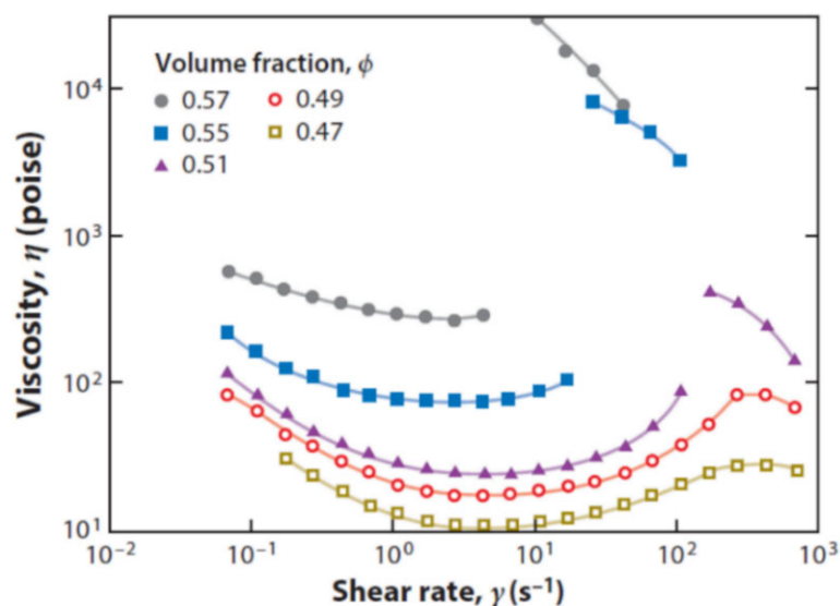
Figure 54. Shear-thickening in suspensions of electrically charged particles at high \phi . Adapted from [49].
