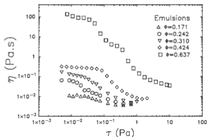
Figure 71. Viscous behaviour of micelle-induced depletion-flocculated emulsions. Adapted from [69].
