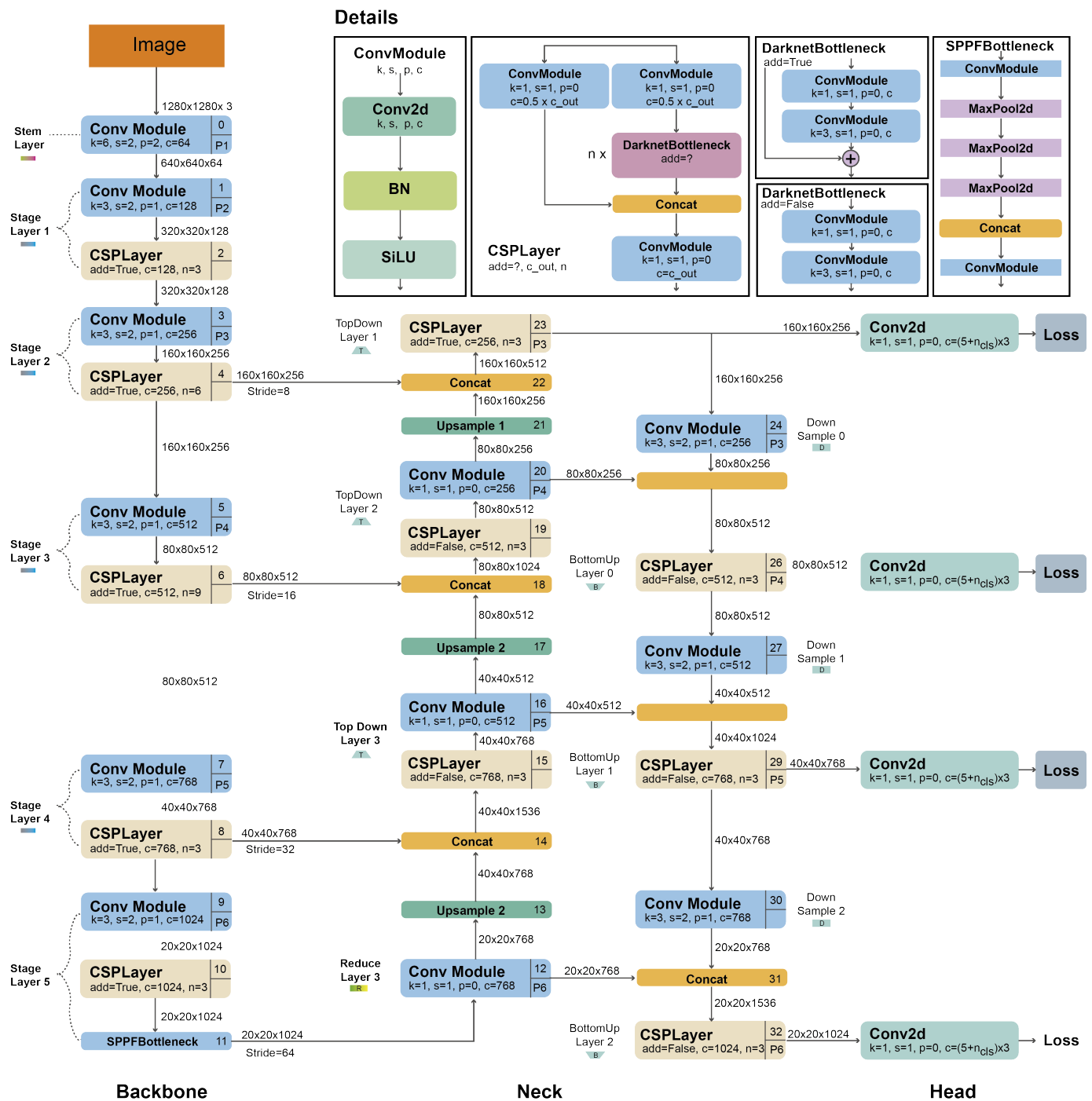
Figure 13. YOLOv5 architecture. The architecture uses a modified CSPDarknet53 backbone with a Stem, followed by convolutional layers that extract image features. A spatial pyramid pooling fast (SPPF) layer accelerates computation by pooling features into a fixed-size map. Each convolution has batch normalization and SiLU activation. The network's neck uses SPPF and a modified CSP-PAN, while the head resembles YOLOv3. Diagram based on [82,83].
