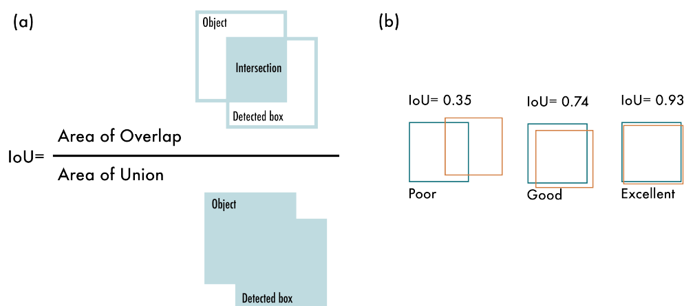
Figure 3. Intersection over Union (IoU). (a) The IoU is calculated by dividing the intersection of the two boxes by the union of the boxes; (b) examples of three different IoU values for different box locations.
