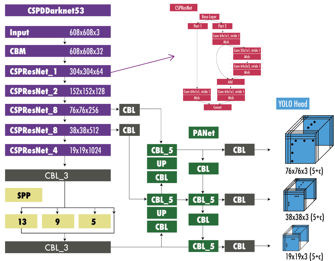
Figure 12. YOLOv4 architecture for object detection. The modules in the diagram are CMB: convolution + batch normalization + Mish activation, CBL: convolution + batch normalization + Leaky ReLU, UP: upsampling, SPP: spatial pyramid pooling, and PANet: path aggregation network. Diagram inspired by [80].
