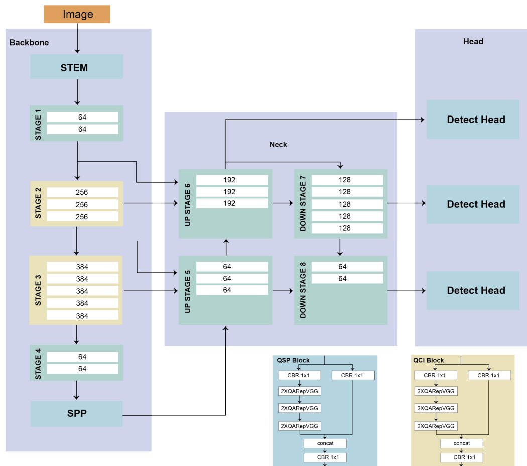
Figure 19. YOLO-NAS architecture. The architecture is found automatically via a neural architecture search (NAS) system called AutoNAC to balance latency vs. throughput. They generated three architectures called YOLO-NASS (small), YOLO-NASM (medium), and YOLO-NASL (large), varying the depth and positions of the QSP and QCI blocks. The figure shows the YOLO-NASL architecture.
