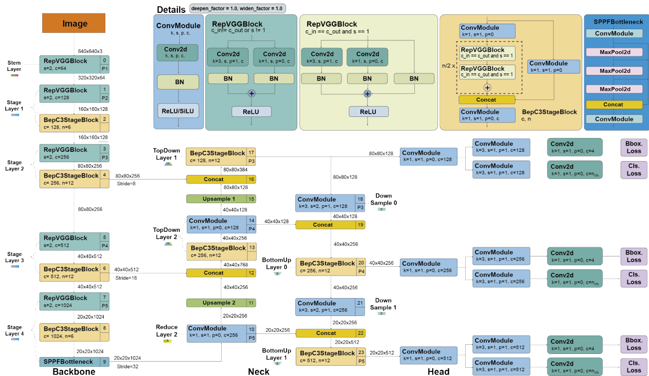
Figure 15. YOLOv6 architecture. The architecture uses a new backbone with RepVGG blocks [99]. The spatial pyramid pooling fast (SPPF) and Conv modules are similar to YOLOv5. However, YOLOv6 uses a decoupled head. Diagram based on [100].
