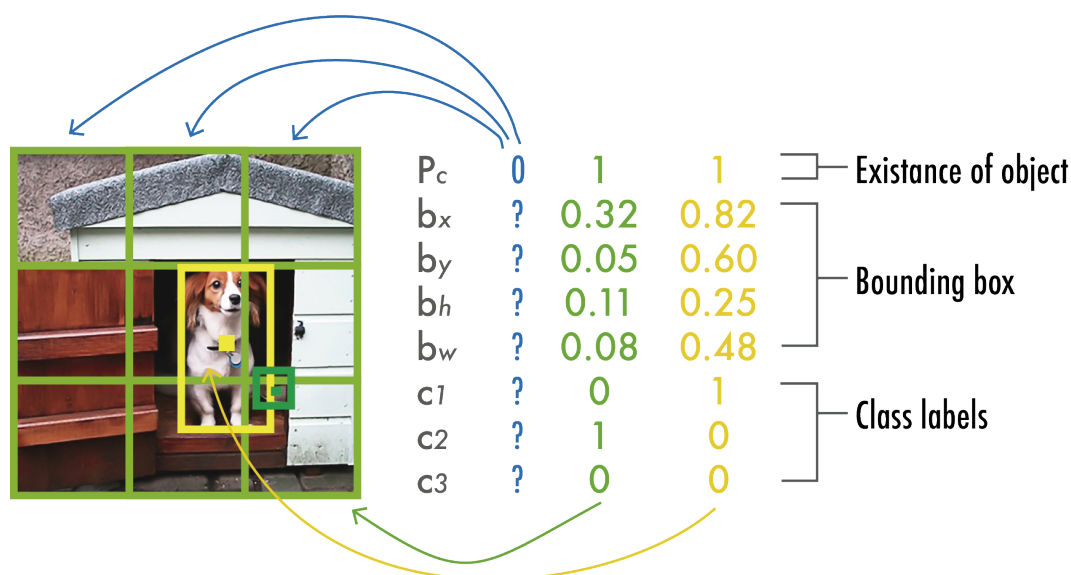
Figure 5. YOLO output prediction. The figure depicts a simplified YOLO model with a three-by-three grid, three classes, and a single class prediction per grid element to produce a vector of eight values.
