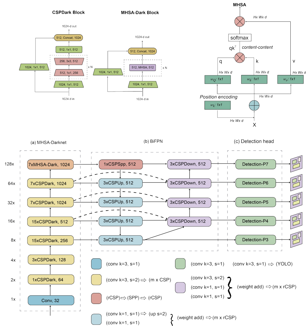
Figure 20. ViT-YOLO architecture. The backbone MHSA-Darknet combines multi-head self-attention blocks (MHSA-Dark Block) with cross-stage partial-connection blocks (CSPDark block). The neck uses BiFPN to aggregate features from different backbone levels, and the head comprises five multi-scale detection heads.
