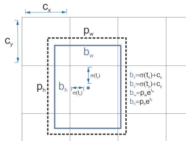
Figure 8. Bounding box prediction. The box's center coordinates are obtained with the predicted t_x , t_y values passing through a sigmoid function and offset by the location of the grid cell c_x , c_y . The width and height of the final box use the prior width p_w and height p_h scaled by e^{t_w} and e^{t_h} , respectively, where t_w and t_h are predicted by YOLOv2.
