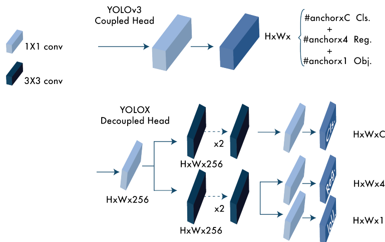
Figure 14. Difference between YOLOv3 head and YOLOX decoupled head. For each level of the FPN, they used a 1 \times 1 convolution layer to reduce the feature channel to 256. Then, they added two parallel branches with two 3 \times 3 convolution layers each for the class confidence (classification) and localization (regression) tasks. The IoU branch is added to the regression head.
