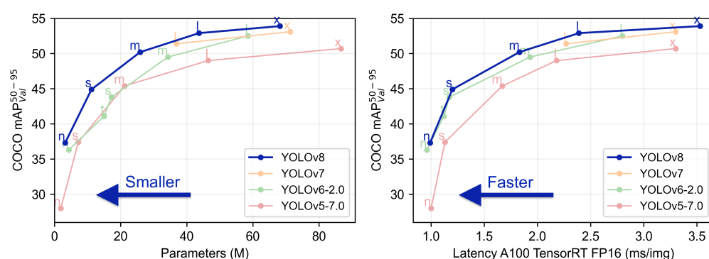
Figure 21. Performance comparison of YOLO object detection models. The left plot illustrates the relationship between model complexity (measured by the number of parameters) and detection accuracy (COCO mAP50-95). The right plot shows the tradeoff between inference speed (latency on A100 TensorRT FP16) and accuracy for the same models. Each model version is represented by a distinct color, with markers indicating size variants from nano to extra . Plots taken from [139].
