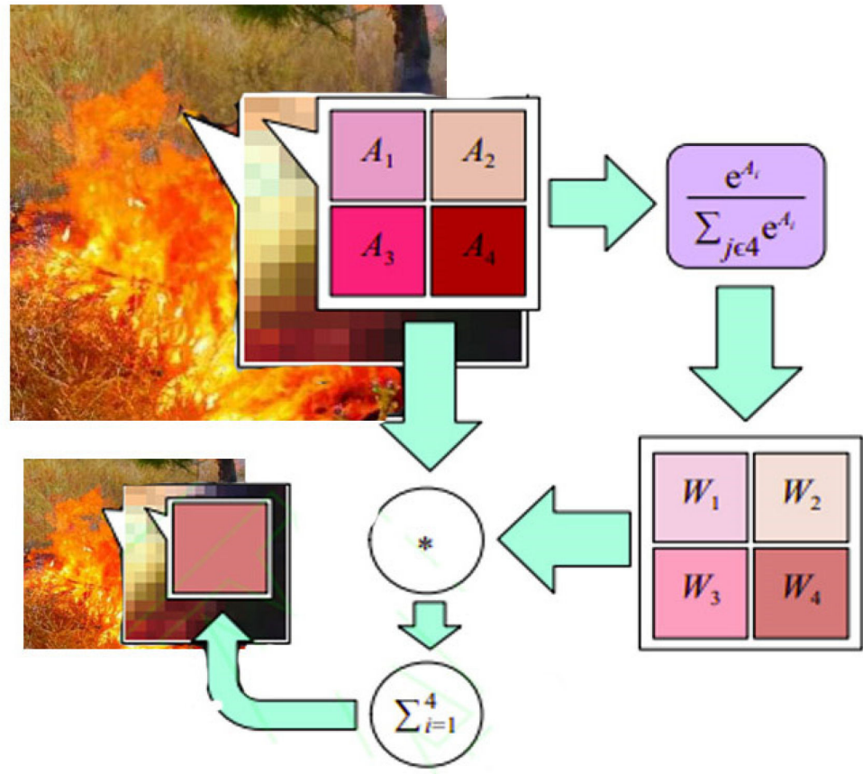
Figure 3. SoftPool calculation flowchart.
