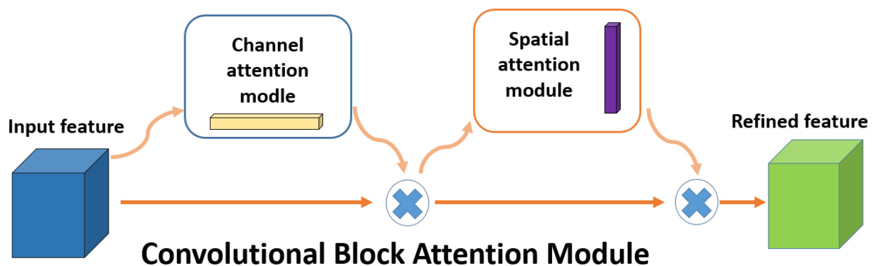
Figure 2. Convolutional Block Attention Module.
