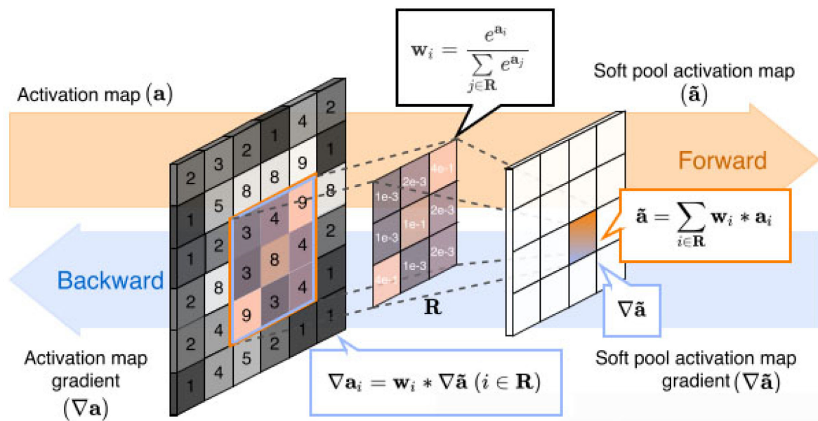
Figure 4. SoftPool transfer process diagram.
