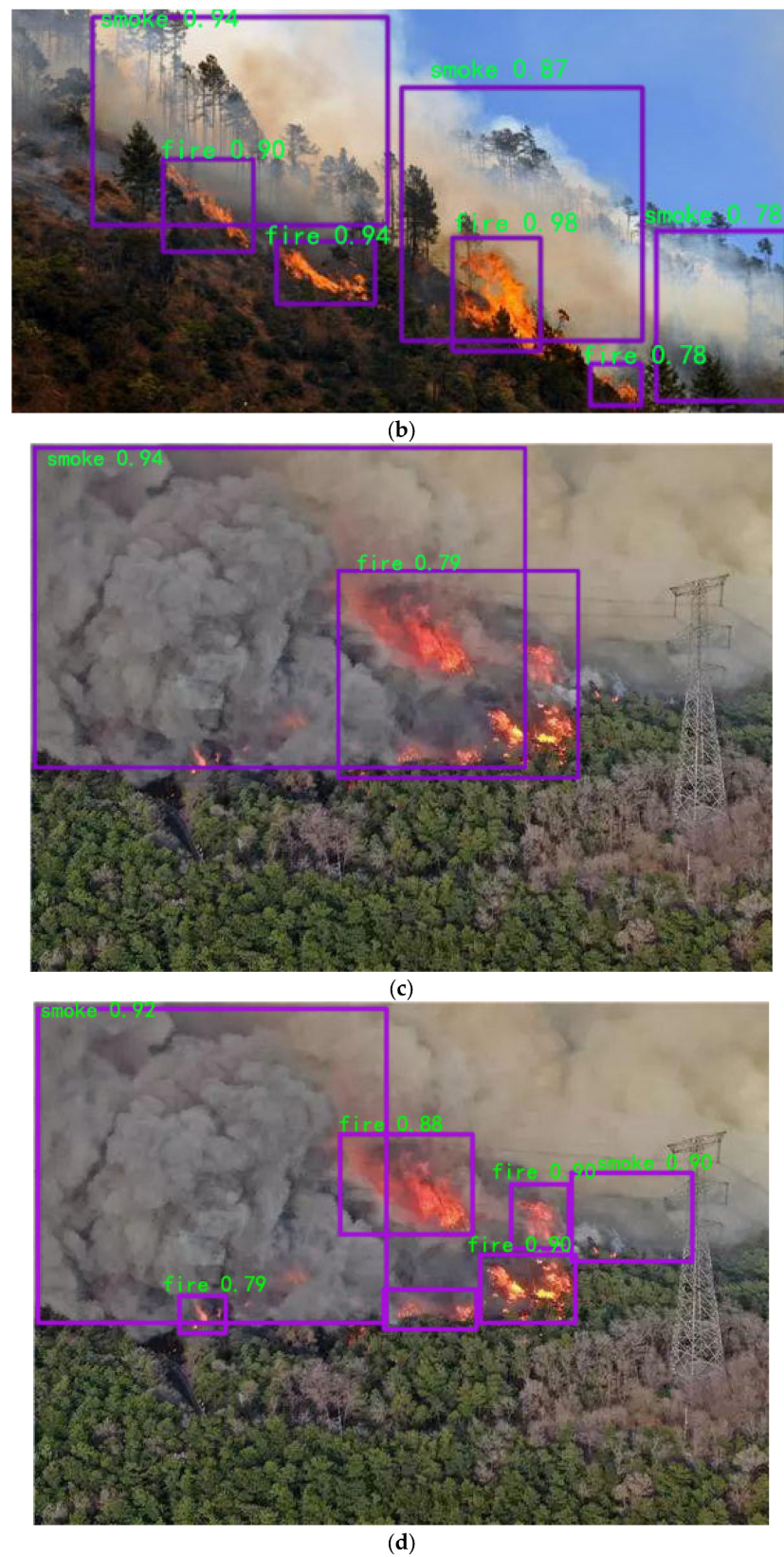
Figure 9. The detection results of the YOLOv5 and YOLOv5-IFFDM models for forest fire and smoke from the UAV camera view. (a) Fire and smoke detection using YOLOv5; (b) Fire and smoke detection using YOLOv5-IFFDM; (c) Fire and smoke detection using YOLOv5; (d) Fire and smoke detection using YOLOv5-IFFDM.
