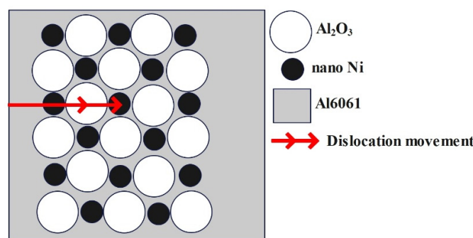
Figure 6. Schematic diagram of hardness enhancement in \text{Al}_2\text{O}_3 -nano-Ni composite coatings.
