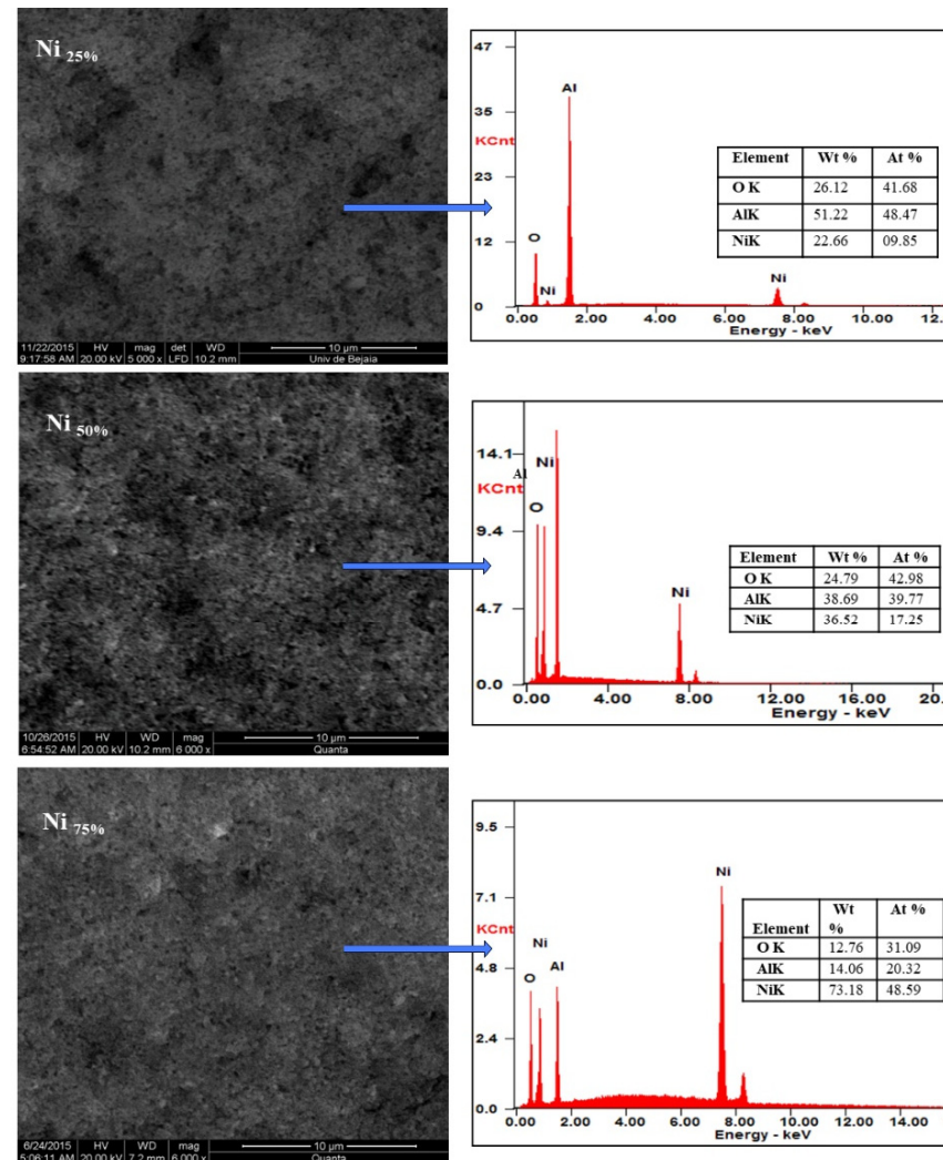
Figure 4. SEM micrographs and EDS spectra of Al 2 O 3 -nano-Ni composite coatings at different nano-Ni ratios.
