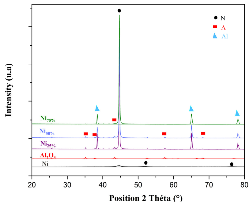
Figure 3. X-ray diffraction patterns of Al 2 O 3 , Ni nanoparticles, and Ni-Al 2 O 3 composite coatings at different ratios of Ni. (N: nickel; A: alumina; Al: aluminium).
