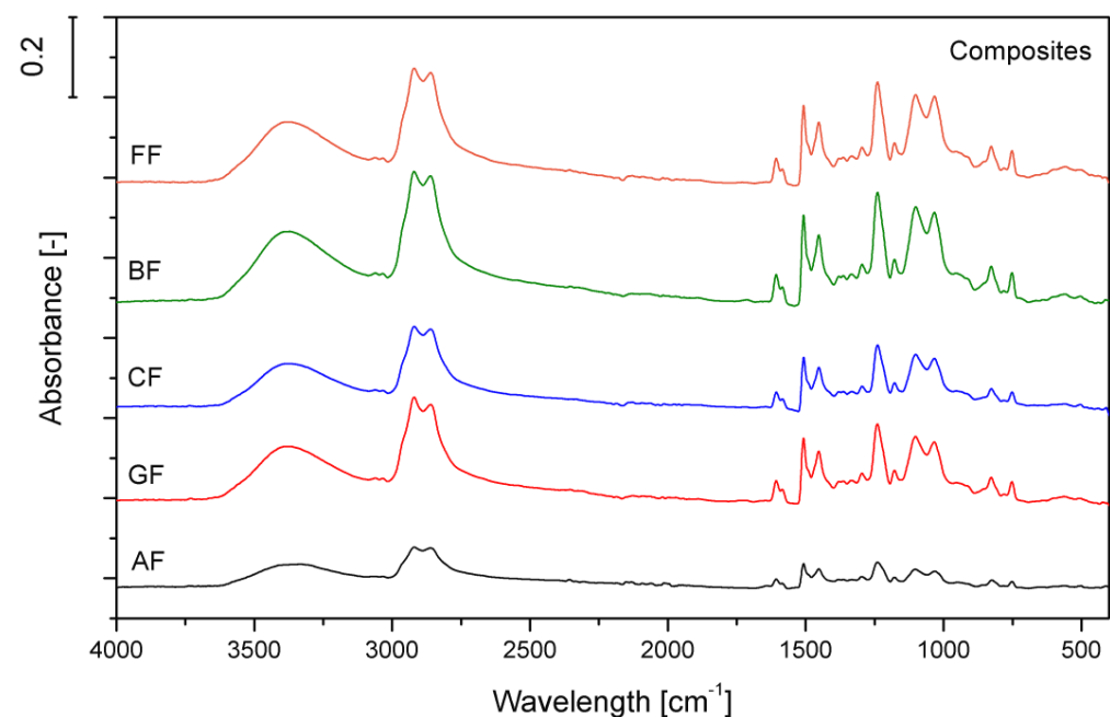
Figure 4. FTIR-ATR spectra of EP laminates.
