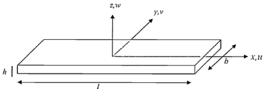
Figure 4. Beam element [21].
