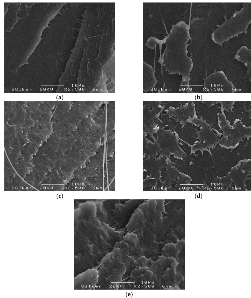
Figure 13. SEM micrographs of fractured surfaces of systems modified with DGEBA, with a magnification of \times 2500 : (a) PLA, (b) 95/5, (c) 90/10, (d) 85/15, and (e) 80/20.
