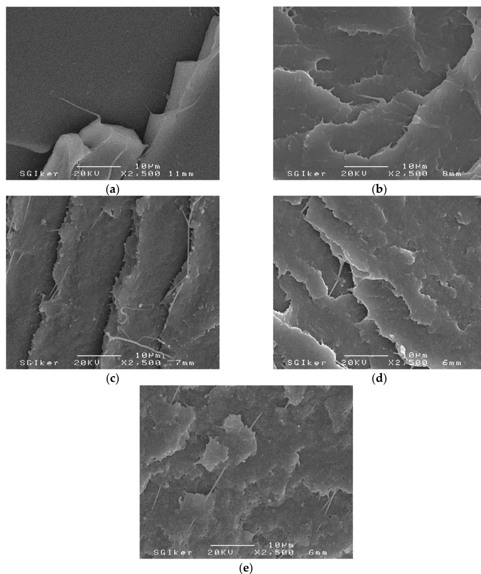
Figure 6. SEM micrographs of fractured surfaces of prepared systems with a magnification of x2500: (a) neat PLA, (b) 95/5, (c) 90/10, (d) 85/15, and (e) 80/20.
