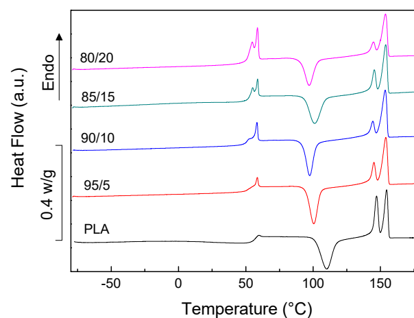
Figure 10. The second heating run thermograms of PLA and blend modified with DGEBA.
