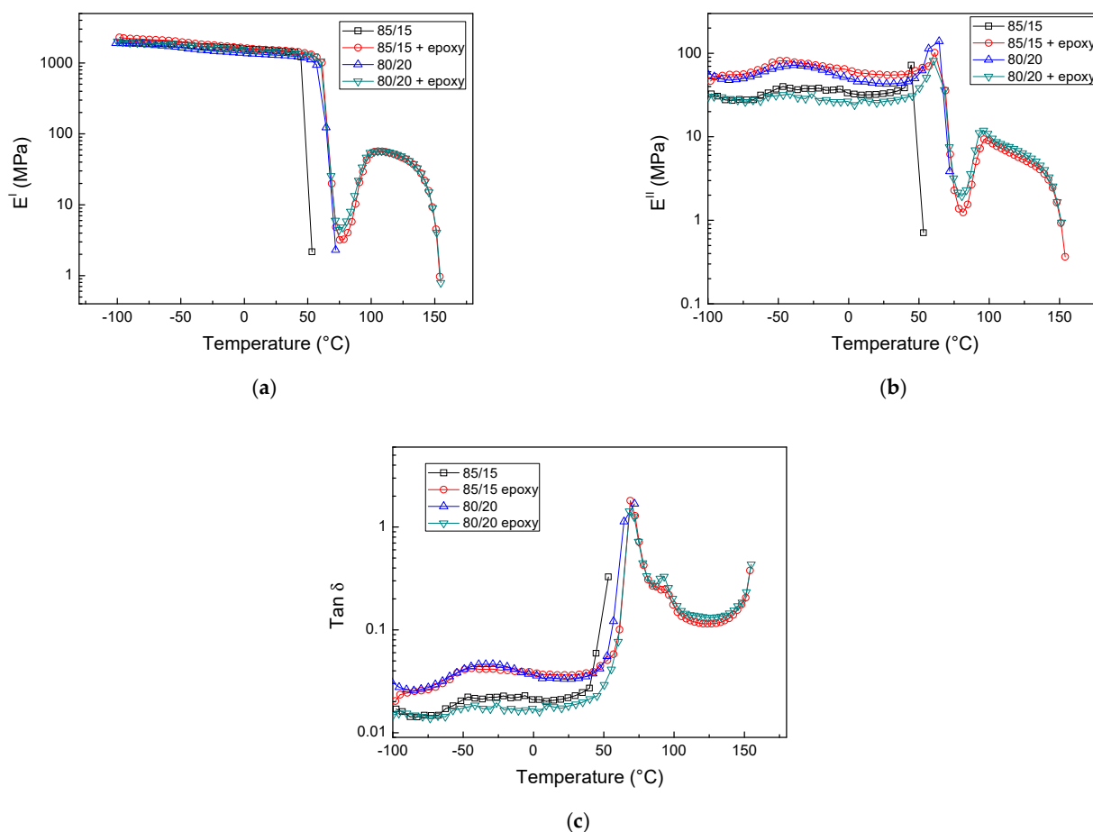
Figure 11. (a) Storage modulus, (b) loss modulus, and (c) \tan \delta variations with temperature.
