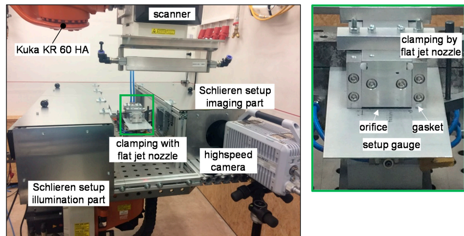
Figure A1. Experimental setup with laser system, Schlieren setup and flat jet nozzle.
