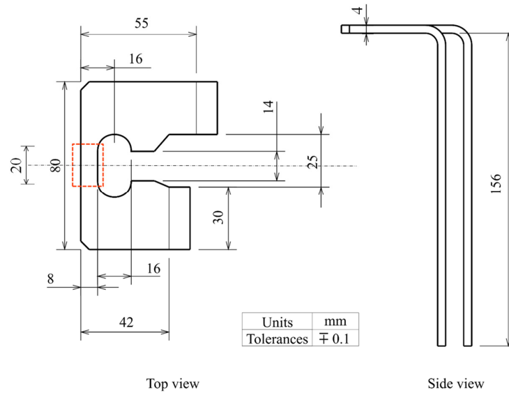
Figure 5. O-shape coil dimensions
