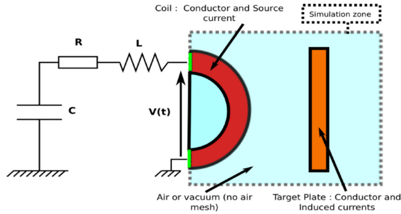
Figure 10. Problem with (R, L, C) imposed voltage on the coil [28]
