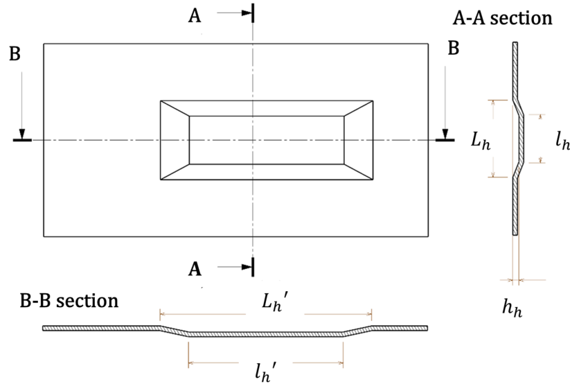
Figure 8. General geometry of the hump for MPSW.
