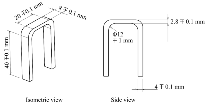
Figure 4. Linear rectangular cross-section coil
