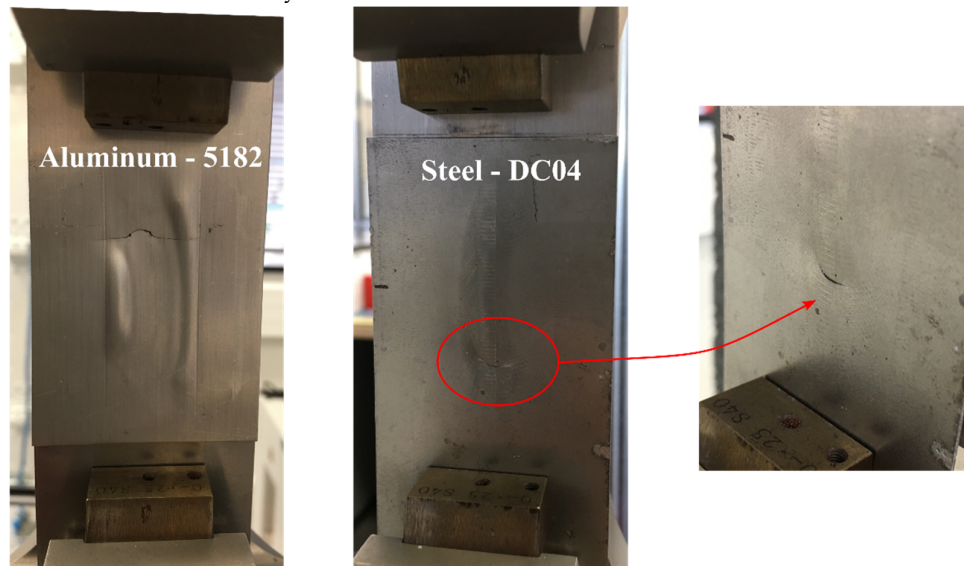
Figure 16. Aluminum 5182 and steel DC04 tearing during fatigue tests
