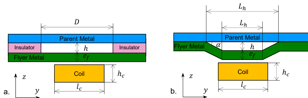
Figure 3. Experimental setup: (a) MPW; (b) MPSW
