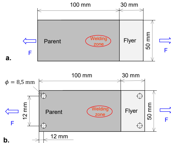
Figure 9. (a) quasi static and fatigue lap shear tests specimen, (b) dynamic lap-shear test specimen
