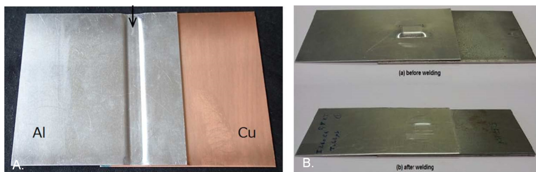
Figure 2. (A) Al/Cu MPW [21]; (B) MPSW [18]
