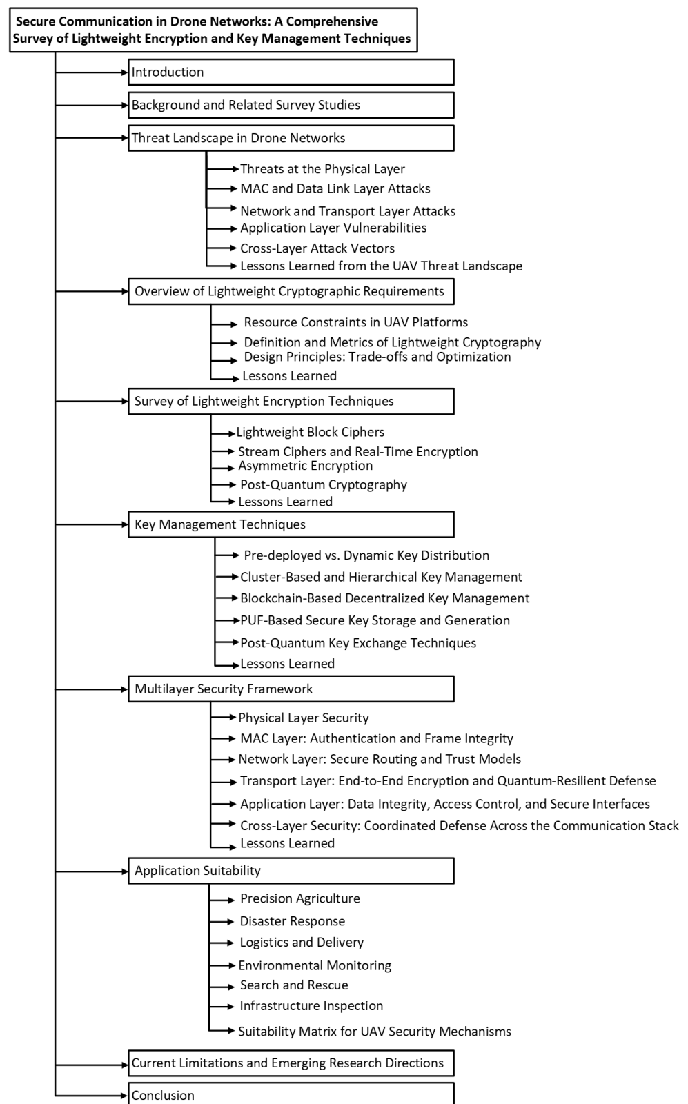
Figure 2. Organizational structure of the UAV communication security survey.
