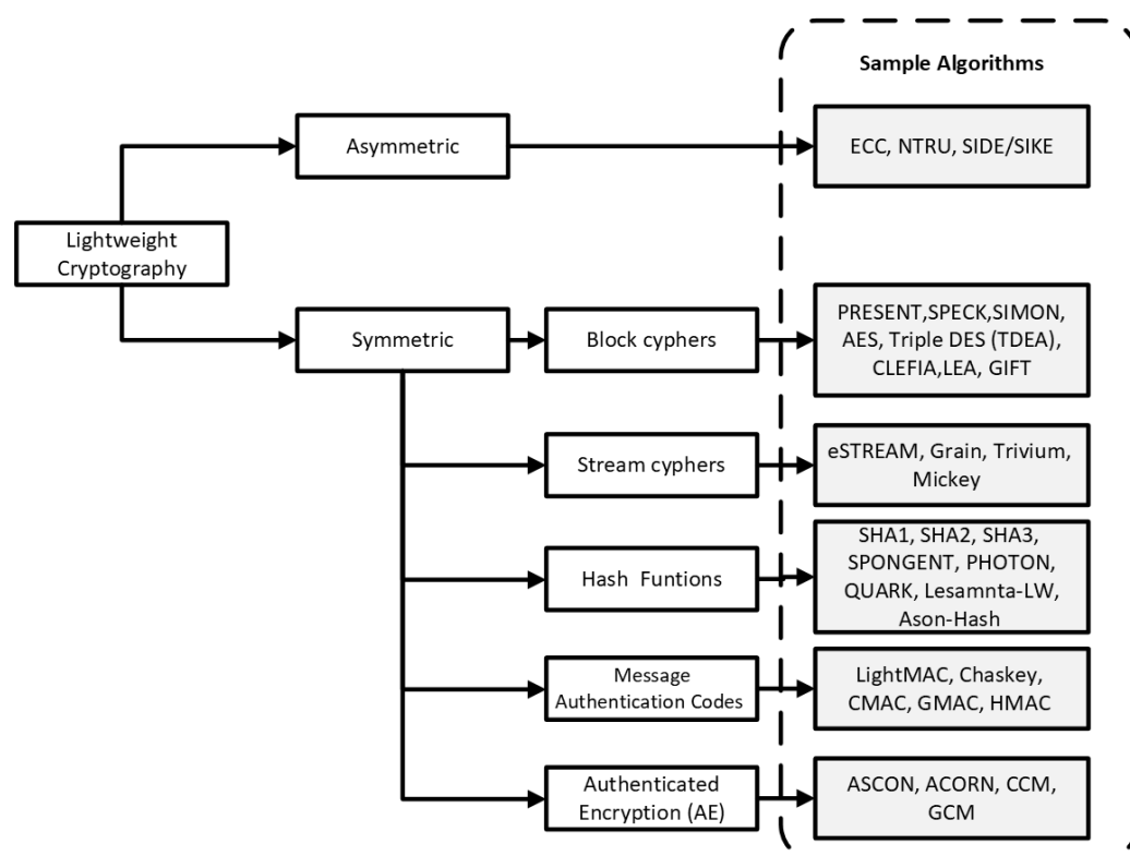
Figure 7. Categories of lightweight cryptographic primitives.
