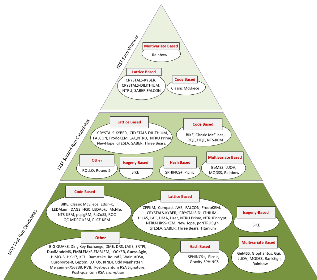
Figure 10. Post-quantum encryption systems in the NIST competition.
