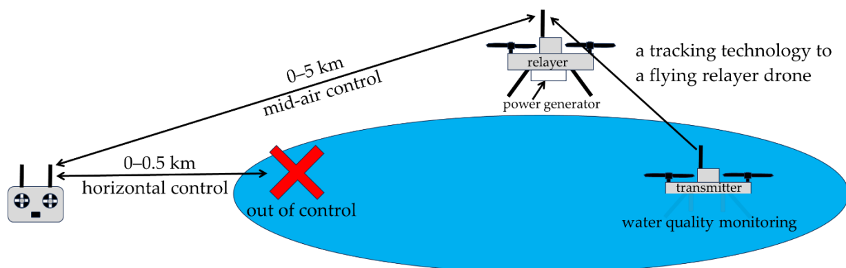
Figure 22. Example of a wireless data relay application to amphibious drones. A tracking (‘follow me’) technology (3D Robotics Inc., United States) enables large-scale water surveys with amphibious drones.
