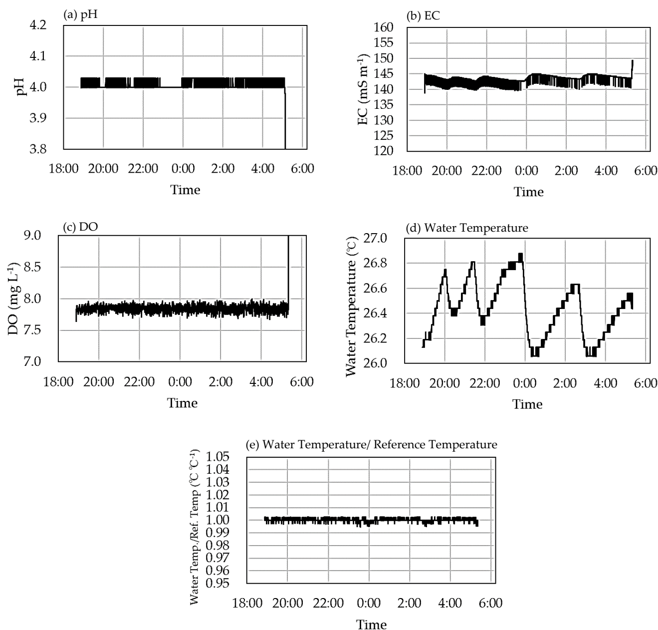
Figure 11. Results of data stability testing of the system for the SplashDrone™3+ with rechargeable batteries: (a) pH values of a standard solution (potassium phthalate buffer, pH 4.01); (b) electrical conductivity values of a 1.41 dS m -1 standard solution (141 mS m -1 ); (c) dissolved oxygen concentration values of the drawn tap water circulated continuously with air bubbling; (d) water temperature values of the tap water; (e) the ratio of water temperature and reference temperature values (the reference temperature values were obtained with stable power source). The EC values were corrected by the water temperature data to represent the values at 298 K. Temperature compensation for the DO measurement was conducted only for the membrane permeability fluctuation (not for standardization).
