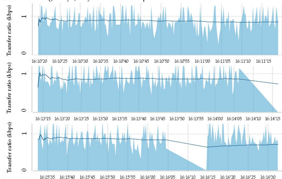
Figure 15. Results of throughput tests with hovering relay drone positioned at the center of a 100 m line of sight. The test for each condition was repeated three times. The test duration (cutoff time)
