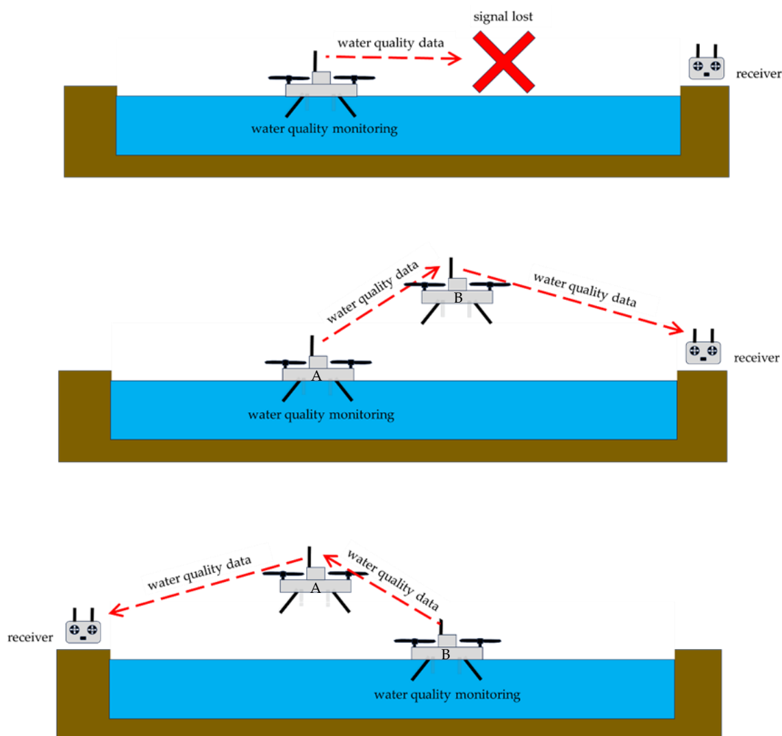
Figure 1. A conceptual illustration of wireless data relay for water quality monitoring using multiple amphibious drones. Upper: no data relay, middle: data relay by a flying drone, lower: data relay with alternated roles of drones for large-scale applications with variable receiver locations. Drones A and B are identical but situated in different locations.
