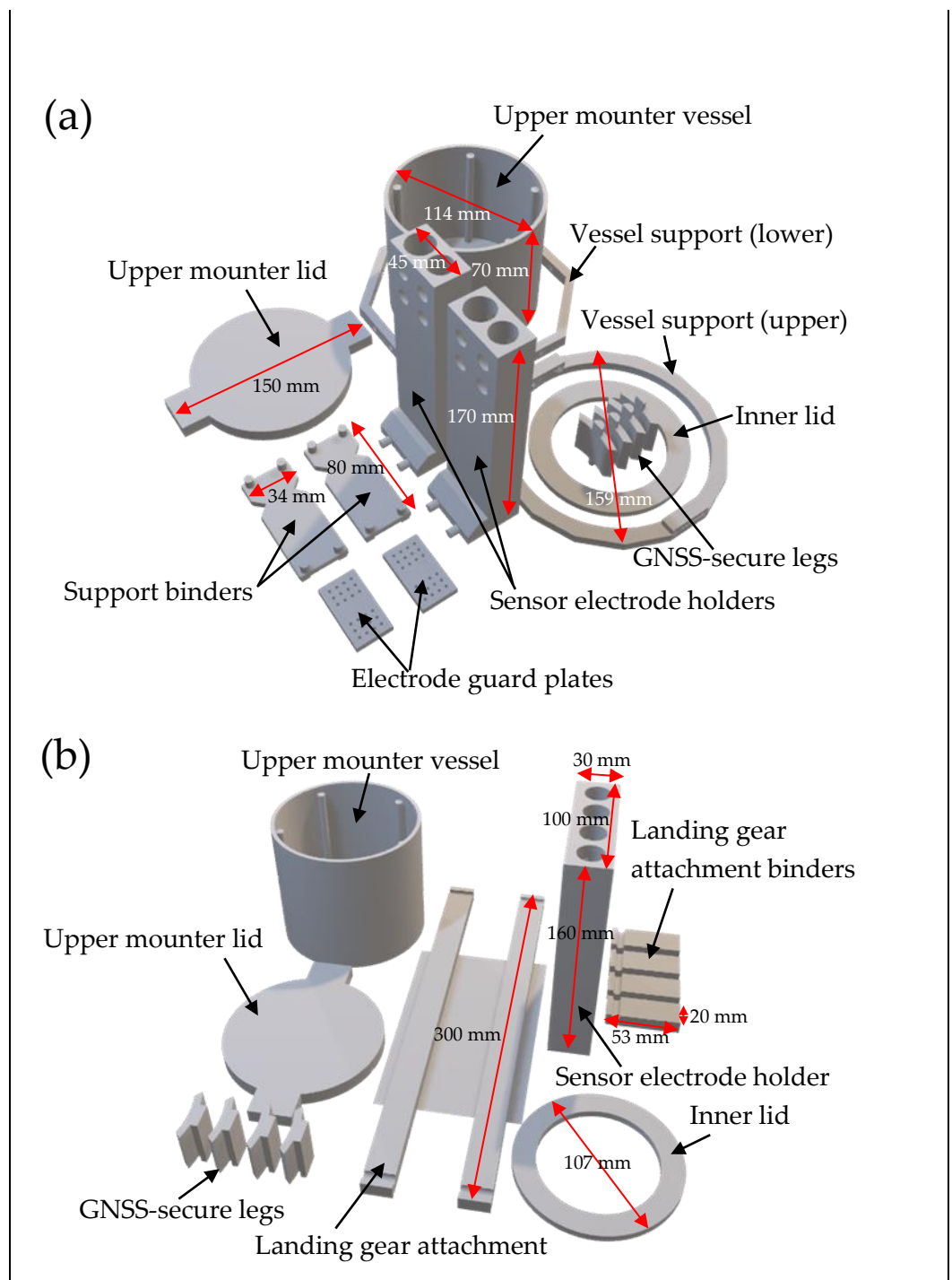
Figure 4. Slicer output images of the mounters for water quality monitoring tools with amphibious drones. (a) Mounters for the SplashDrone™ 3+ with vertical installation of sensor electrodes; (b) mounters for the SplashDrone™ 4 with horizontal installation of sensor electrodes (the holder is shown as a vertical image for 3D-printer output). GNSS-secure legs were used for sufficient space between the bottom of the upper mounter vessel and the GNSS antenna surface of each drone.
