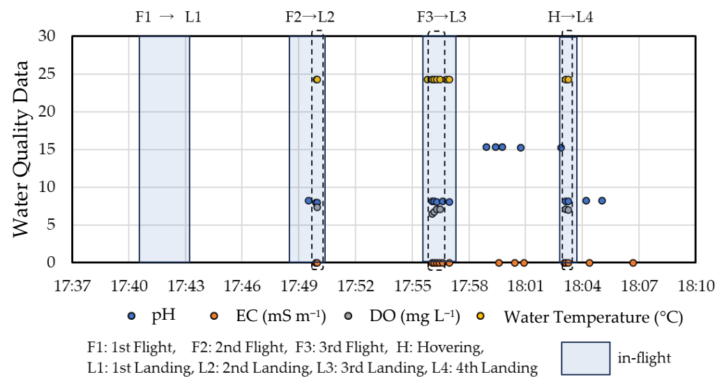
Figure 18. Received water quality data from the extending relay test. The horizontal distance between the transmitter drone and the relay drone at each landing site was the following: L1, 624 m; L2, 500 m; L3, 381 m; L4, 368 m. Each of the complete datasets (pH, EC, DO, and temperature) is surrounded by a dotted line.
