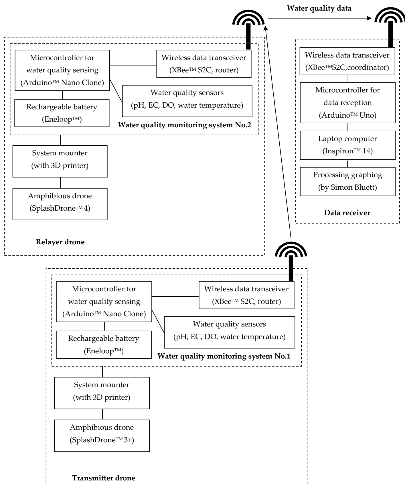
Figure 2. Schematic representation of amphibious drone-mounted water quality monitoring system with wireless data relay.
