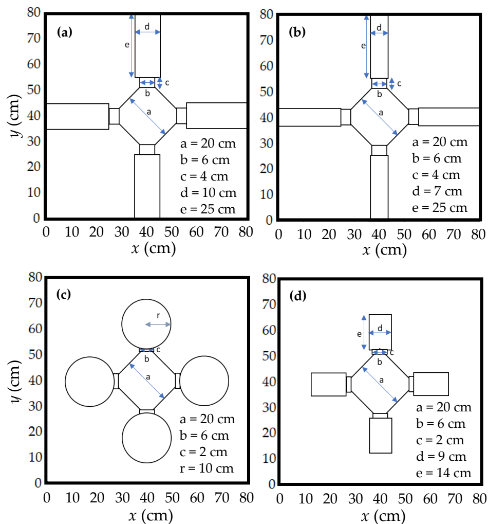
Figure 6. Simplified top view (horizontal view) of the amphibious drone system with additional floating materials: (a) symmetric L-shaped polystyrene-foam bars (the concave of each L-shaped bar is fitted to each of the drone arms, approximately 60 g total weight) made by cutting a polystyrene foam box, (b) empty PET bottles (approximately 940 mL volume, approximately 136 g total weight), (c) coiled tubular polyethylene sponge foam discs (approximately 400 g total weight), and (d) the least amount of sponge-form arm-covers (approximately 85 g total weight) to balance the drones on still water.
