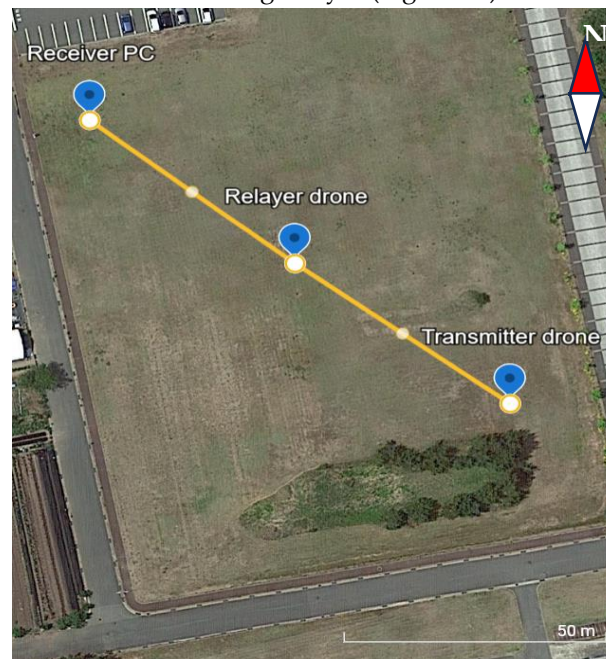
Figure 14. Arrangement of wireless communication devices for quantifying the efficiency of drone hovering in data relaying. The test was conducted on 12 December, 2023 in a flat field at Akita
