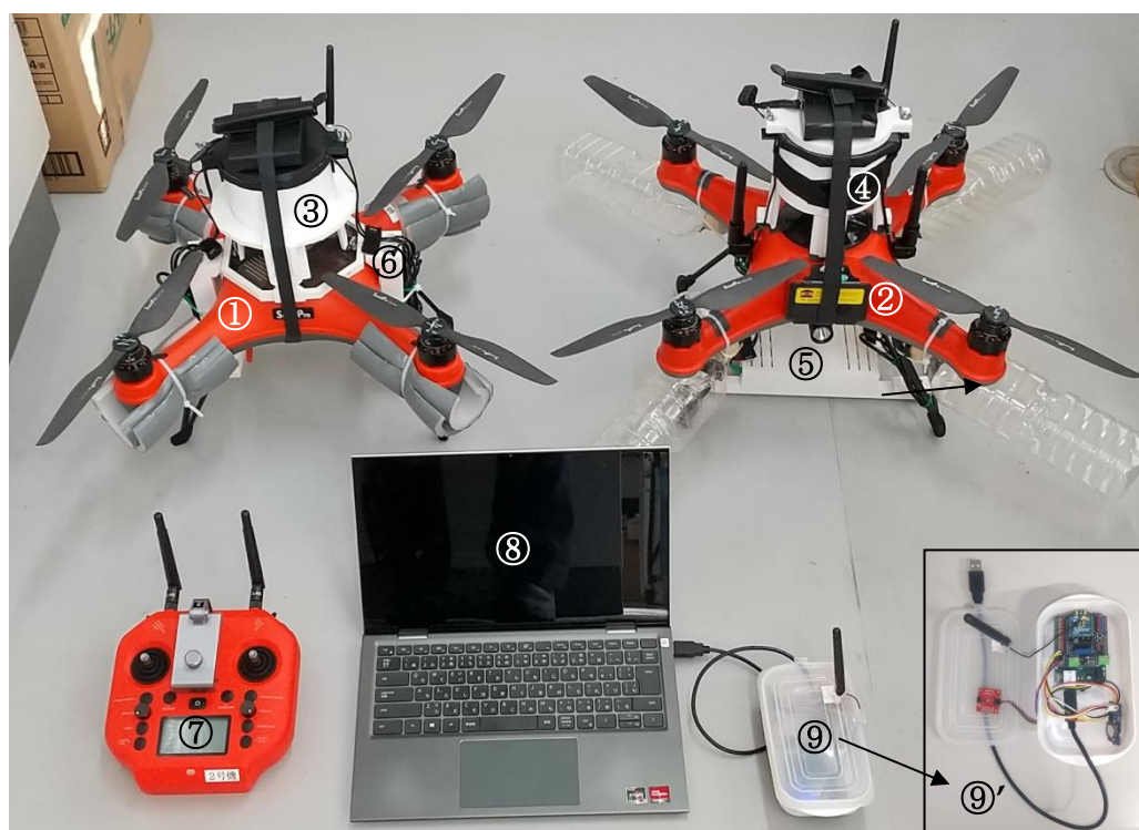
Figure 9. Components of the water quality monitoring system with amphibious drones for wireless data relay tests: 1, SplashDrone™ 3+; 2, SplashDrone™ 4; 3, upper mounter for SplashDrone™ 3+; 4, upper mounter for SplashDrone™ 4; 5, lower mounter for SplashDrone™ 4; 6, side mounter(s) for SplashDrone™ 3+; 7, drone controller for SplashDrone™ 4; 8, laptop computer for data display; 9, receiver; and 9', contents included in the receiver.
