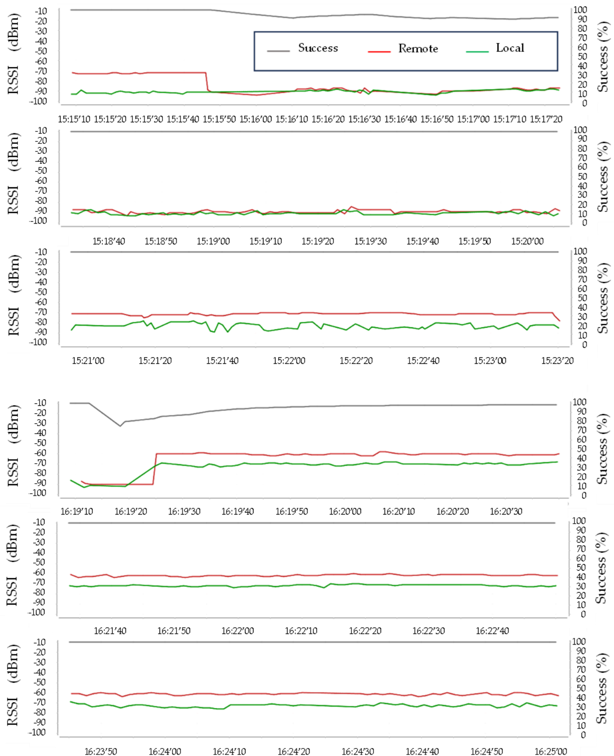
Figure 16. Results of range tests with a hovering relay drone positioned at the center of a 100 m line of sight. RSSI: Received Signal Strength Indicator. Success (%) on the right-side vertical axis represents the Packet Delivery Ratio (PDR, %). The test for each condition was repeated three times. Each packet was to be sent ideally at 1000 ms intervals, but the receiver timeout was set as 10 s for a measurement of water quality at 10 s intervals. The average PDR was 97 \pm 2.7\% for the on-ground
