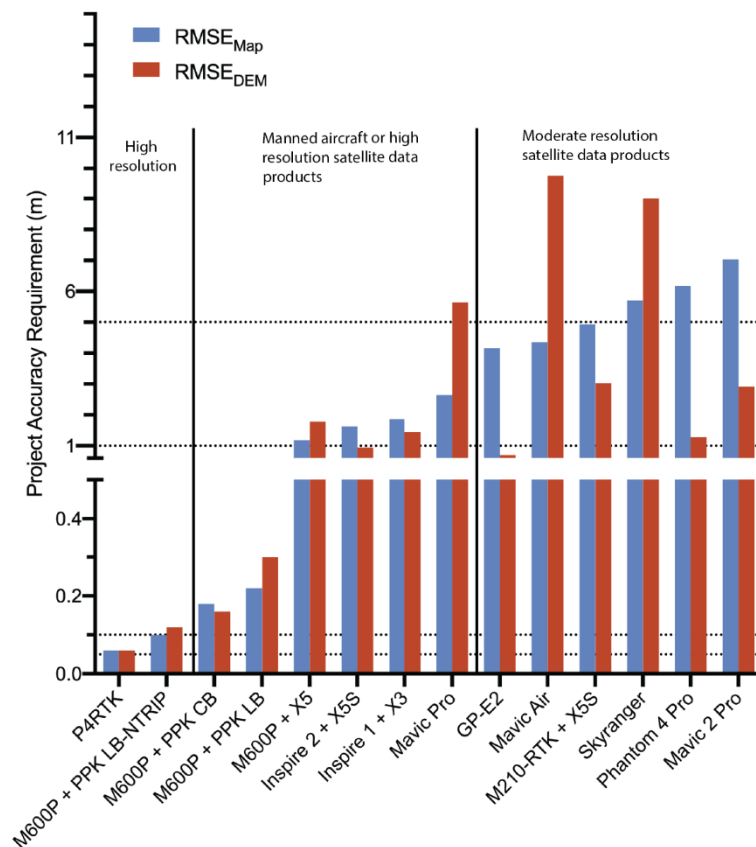
Figure 14. RMSE_{Map,DEM} project accuracy requirements ordered by RMSE_{Map(AT)} . The largest value of RMSE_x or RMSE_y was used to calculate RMSE_{AT} for each UAS. The three project categories, high-resolution, manned aircraft or high-resolution satellite data products, and moderate resolution satellite data products are based on RMSE_{Map(AT)} .
