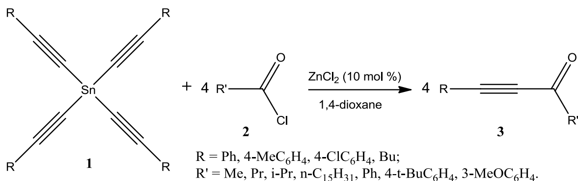
Scheme 1. The reaction of tetraalkynylstannanes with acyl chlorides.
