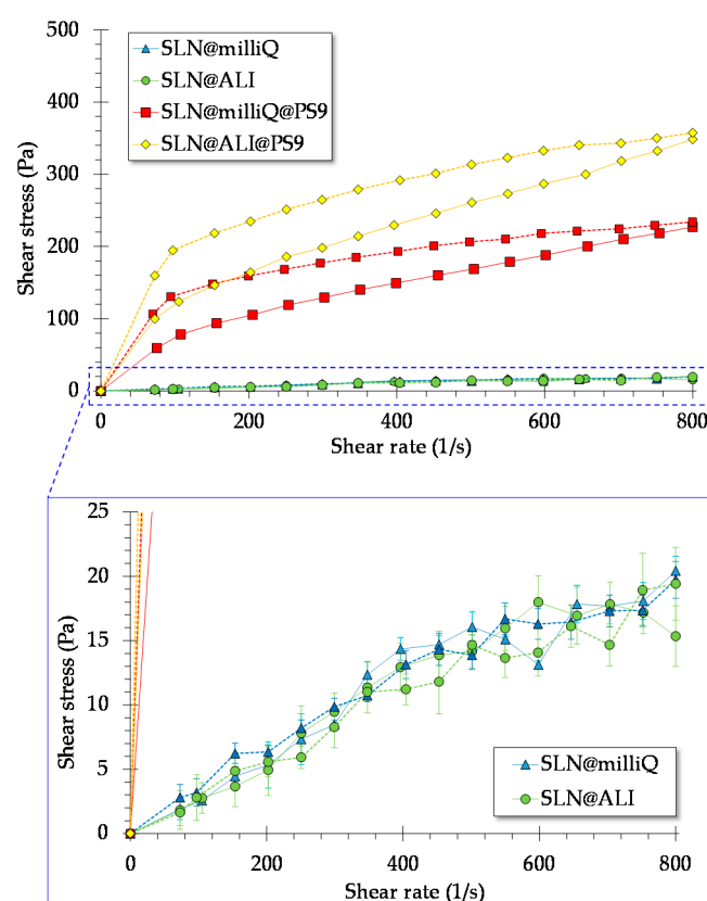
Figure 1. Flow curves of SLN@milliQ, SLN@milliQ@PS9, SLN@ALI, and SLN@ALI@PS9. Uphill curves (70–800 s −1 ) are represented with a continuous line, while dashed lines were used for the return flow curves (800–70 s −1 ).
