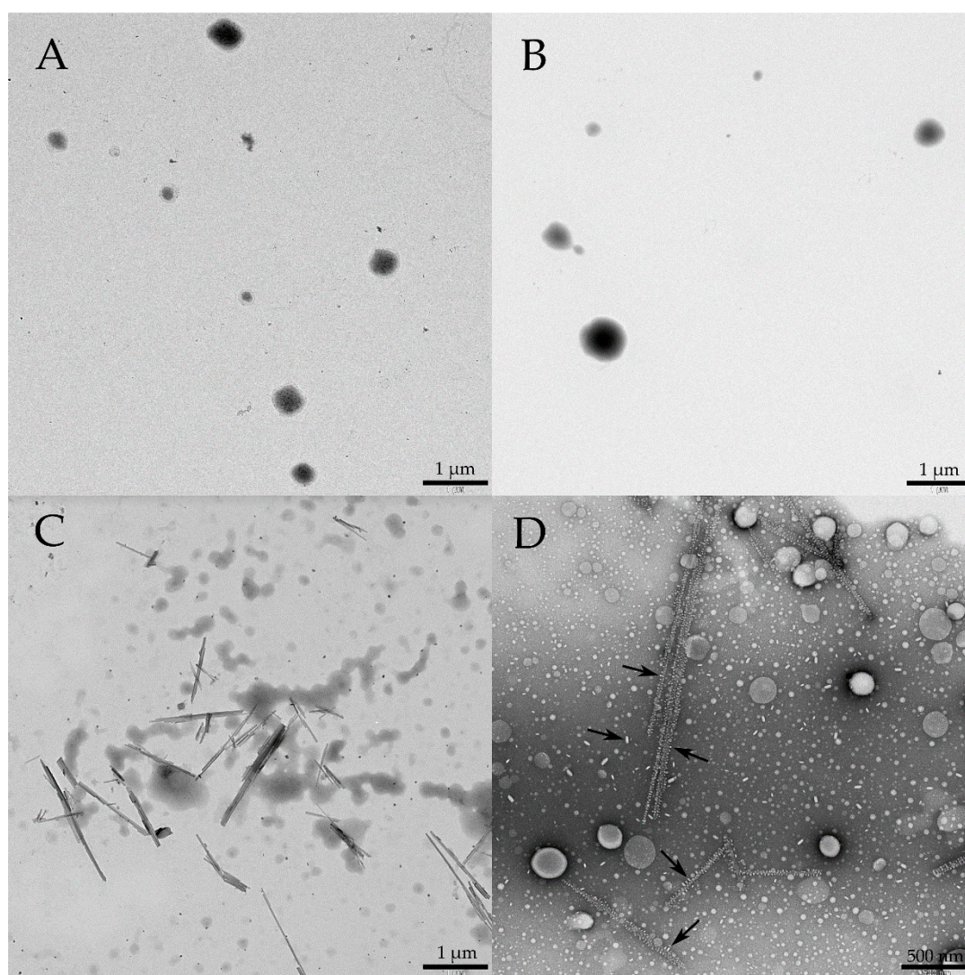
Figure 4. Microphotographs obtained during Transmission Electron Microscopy (TEM) studies of the formulations. (A) SLN@ALI; (B) SLN@milliQ; (C) SLN@ALI@PS9; (D) SLN@milliQ@PS9. Arrows mark tiny micelles surrounding sepiolite fibers.
