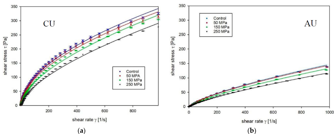
Figure A2. Flowing properties of untreated and UHPH treated (a) CU pectin and (b) AU pectin.
