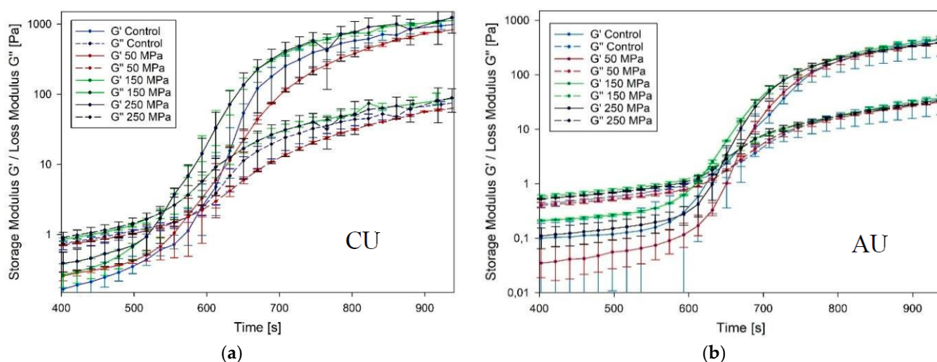
Figure A4. Storage Modulus G' and Loss Modulus G'' of untreated and UHPH treated pectin (a) CU and (b) AU samples during cooling and gelation step.
