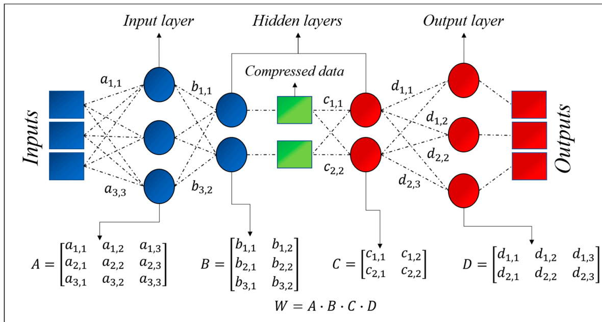
Figure 2. Architecture of the autoencoders used in the present work with the matrixes that multiplied give W . The case shown in the figure is particularised for a latent space of dimension 2.
