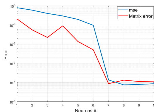
Figure 4. Trend of the errors in the reconstruction of the input data with the dimensionality of the intermediate layer in the autoencoder.
