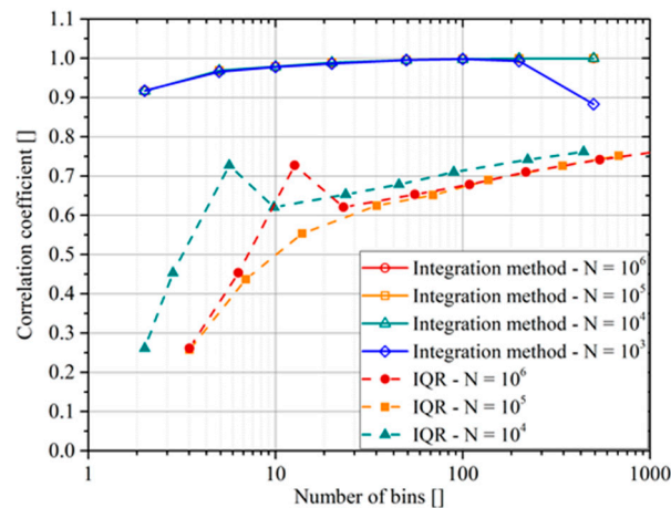
Figure 8. Comparison of the \rho_{int} and the IQR for the negative cubic dependence (third case of Figure 7). The x axis reports the number of bins and N is the number of generated points used to calculate the indicators.
