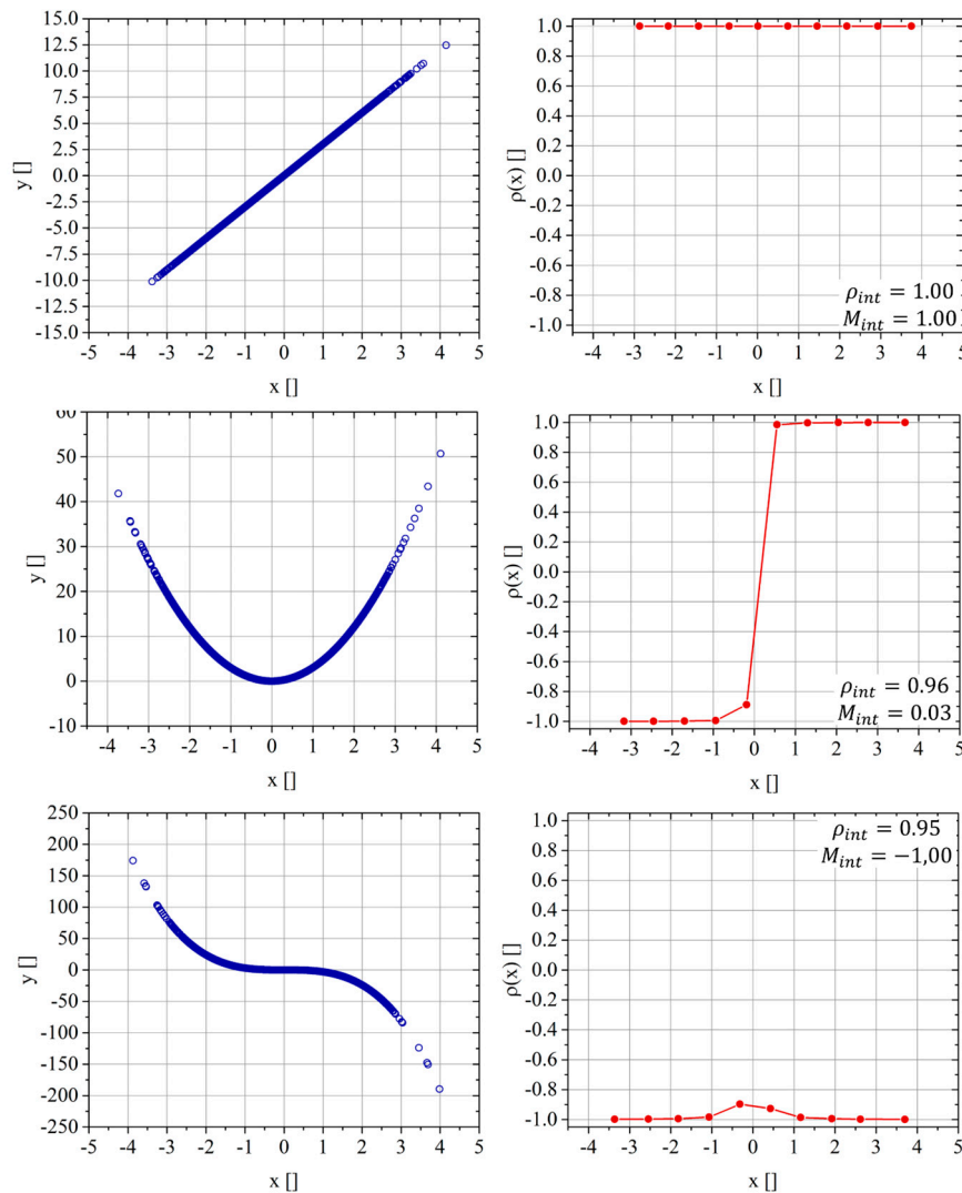
Figure 7. Top: two linearly dependent variables (left) and the relative local correlation coefficient \rho_{int} (right). Middle: two quadratic dependent variables (left) and the relative local correlation coefficient \rho_{int} (right). Bottom: two variables with a cubic negative dependence (left) and the relative local correlation coefficient \rho (right). The integral values of the correlation coefficient and of the monotonicity are reported in the inserts.
