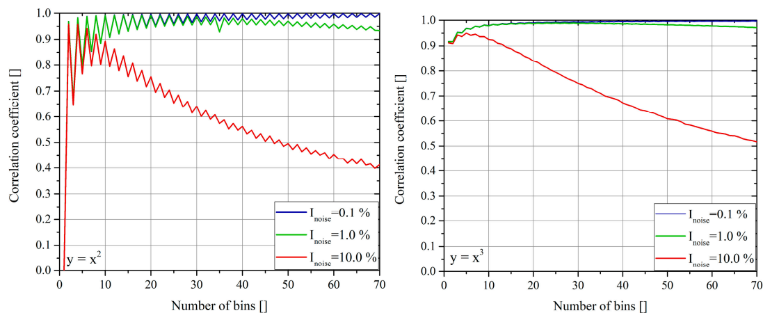
Figure 9. Effects of the noise amplitude on \rho_{int} for various choices of the number of bins. Left plot: the investigated dependence is y = x^2 . Right plot: the investigated dependence is y = x^3 . The independent variable x varies in the range [-10; 10] and the number of points is 10^5 . The noise intensity is calculated as the standard deviation of the noise divided by the standard deviation of the variable amplitude.
