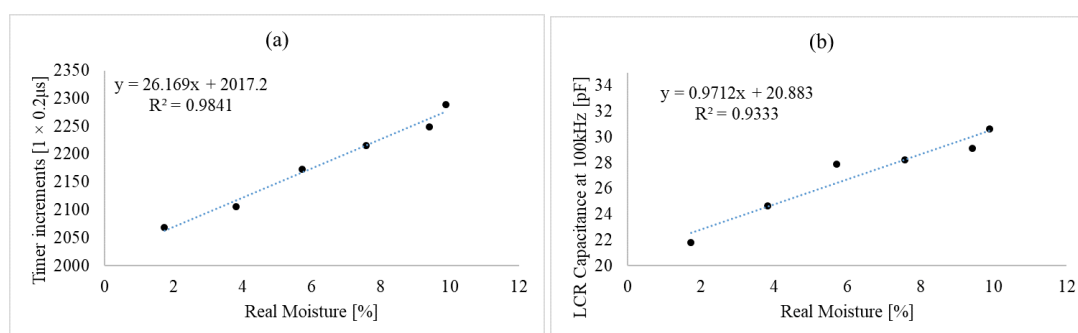
Figure 6. Comparison of calibration results: (a) presents the measurements of the developed system and (b) presents the LCR measurements at 100 kHz.
