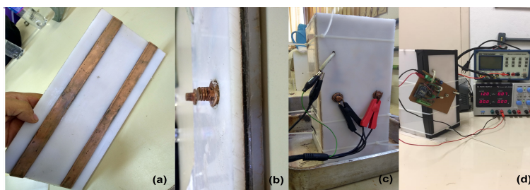
Figure 4. Details of the built capacitive transducer: (a) bottom face, before the PEAD coat; (b) layers and threadable fit to the controller board; (c,d) experimental calibration procedure, alternately performing measurements with the 100 kHz LCR and the built transducer for each wet mineral sample.
