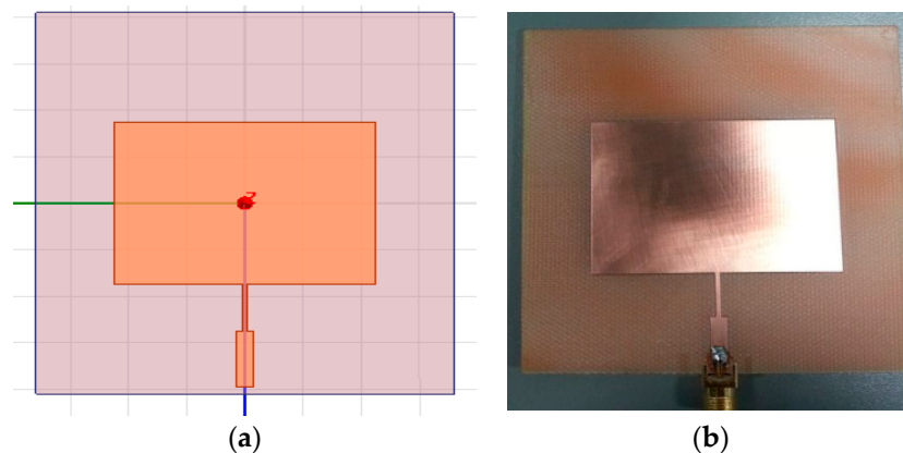
Figure 3. Microwave Patch Antenna: (a) High-Frequency Structural Simulation (HFSS) model and (b) fabricated antenna on a printed circuit board (PCB).
