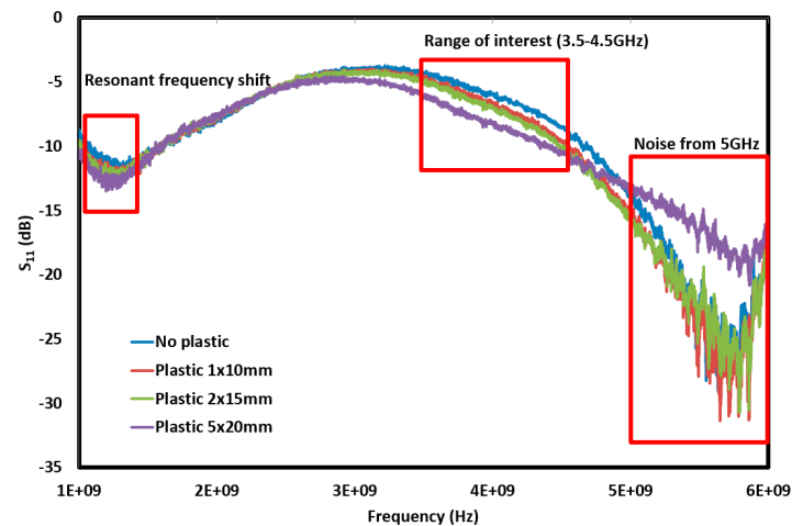
Figure 5. Raw data ( S_{11} ) from the sensor.
