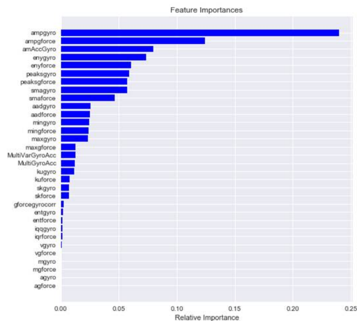
Figure 4. Feature importance.
