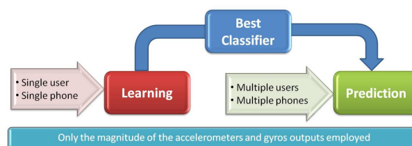
Figure 2. Research methodology.
