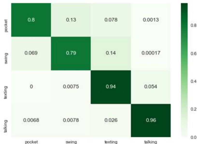
Figure 3. Confusion matrix of the four smartphone modes.
