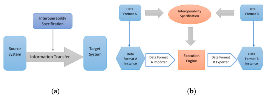
Figure 1. Plug'n'Interoperate Architecture: (a) Interoperability Specifications; (b) Interoperability Execution.
