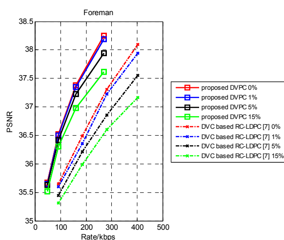
Figure 3. RD of WZF over wireless channel without FC for 'foreman' sequence.
