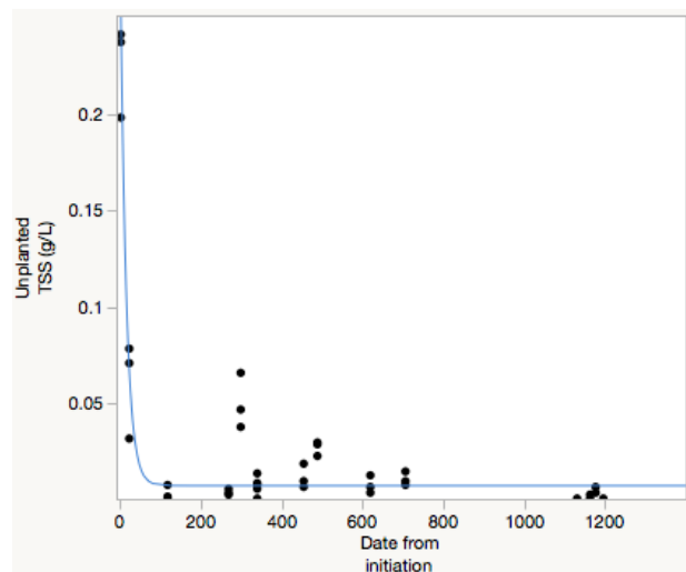
Figure 5. DC FRMS Engine 12 unplanted Aqualok™ total suspended solids (TSS). Total suspended solids (TSS) show high concentrations post-roof installation, but taper off and remain low for the duration of the study. Unplanted TSS (g/L) = 0.2232581 - 0.0706367 \times \text{Log}(\text{Date from initiation}) + 0.005712 \times \text{Log}(\text{Date from initiation})^2 . R = 0.95 .
