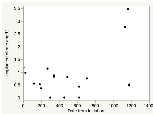
Figure 6. DC FRMS Engine 12 unplanted Aqualok™ NO 3 (mg/L) over time. July 2012 to October 2015.
