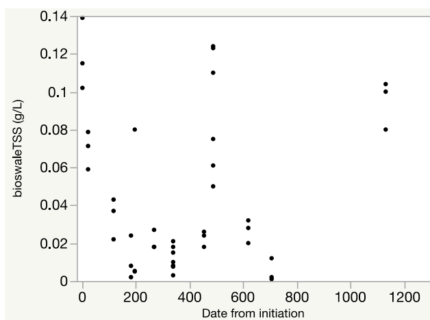
Figure 7. DC FRMS Engine 12 bioswale Aqualok™ total suspended solids (TSS) over time. July 2012 to October 2015.
