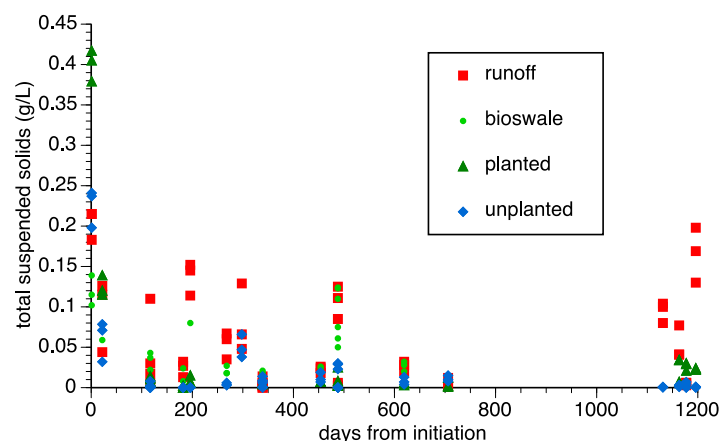
Figure 3. Engine 12 total suspended solids (TSS) from three Aqualok™ treatments vs runoff from the conventional roof. High-throughflow TSS after installation of the Aqualok™ treatments diminished by the 117th day while runoff remained high. Even after >1000 days, the Aqualok™ treatments reduced TSS substantially relative to untreated runoff.
