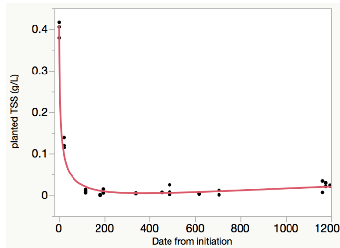
Figure 4. DC FRMS Engine 12 planted Aqualok™, total suspended solids (TSS) versus time. Total suspended solids (TSS) show high concentrations post-roof installation, but taper off and remain low for the duration of the study. Equation of best fit is a second-order logarithmic. Planted TSS (g/L) = 0.4062088 - 0.1355718 \times \text{Log}(\text{Date from initiation}) + 0.0114551 \times \text{Log}(\text{Date from initiation})^2 . R = 0.99 .
