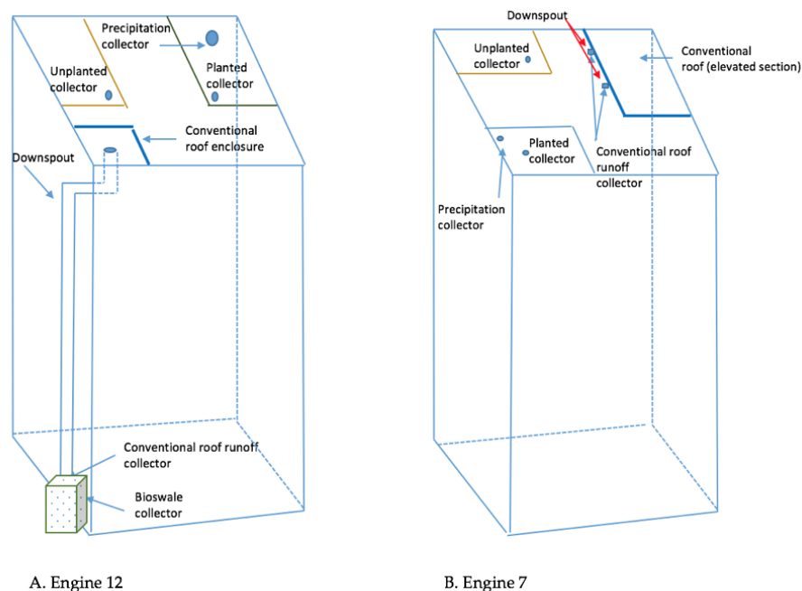
Figure 2. Schematic of green surface plus points of collection from D.C. Fire and Emergency Medical Services (DC FEMS) Engines 12 (A) and 7 (B). The planted and unplanted collectors are under the Aqualok™ foam panels in the respective areas outlined as rectangles in the figure. The figure is not to scale and only represents the positions of the various green surfaces and collection points.
