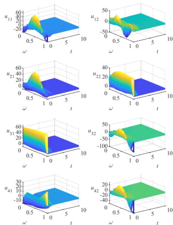
Figure 8. The control input of FCSNHSPDE (16).
