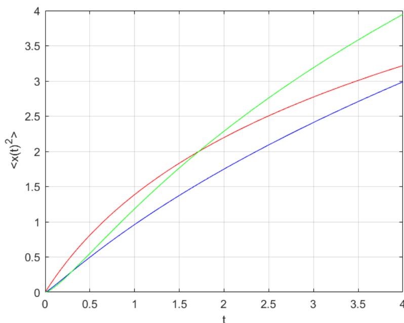
Figure 5. Graph of FMSD of ultra-slow fractal scaled Brownian motion setting \gamma = 1 , \alpha = 1 (red), \gamma = 0.63 , \alpha = 0.5 (blue), and \gamma = 1 , \alpha = 0.7 (green).
