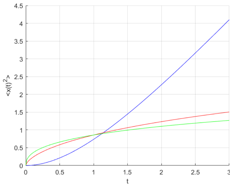
Figure 3. Graph of FMSD of under-damped Langevin equation setting \gamma = 1 , \alpha = 1 (blue), \gamma = 0.63 , \alpha = 0.5 (red), and \gamma = 0.43 , \alpha = 0.5 (green).
