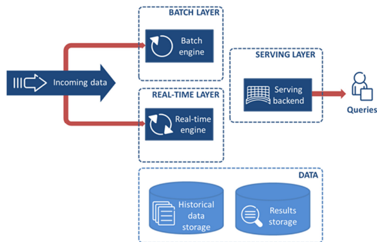
Figure 1. Lambda architecture ( www.ericsson.com ).
