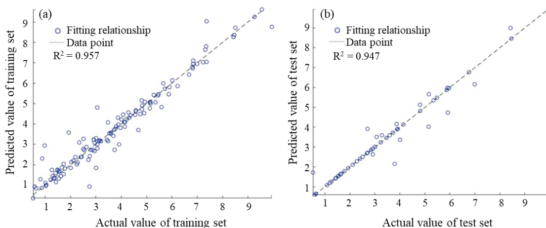
Figure 16. Regression plot between the actual value and the predicted value of the network output: (a) Training set; (b) Test set.
