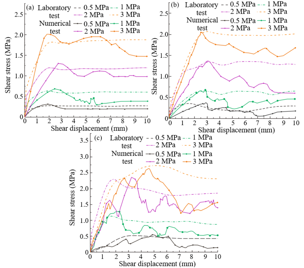
Figure 5. The relationship between shear stress and shear displacement of granite-mortar structural planes: (a) R1; (b) R2; (c) R3.
