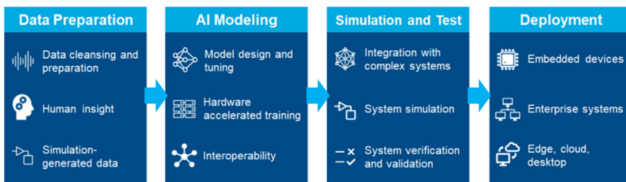
Figure 3. Workflow of AI-based project development in MATLAB.
